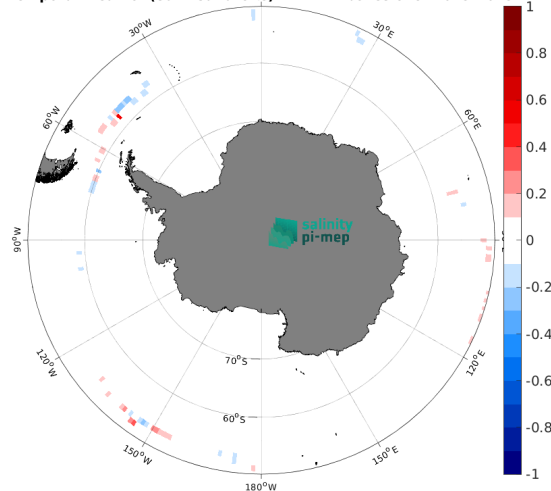
(e) MEAN( \Delta SSS) (Satellite - Saildrone)
