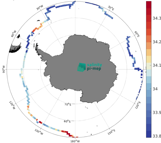
(c) MEAN(Saildrone SSS)
