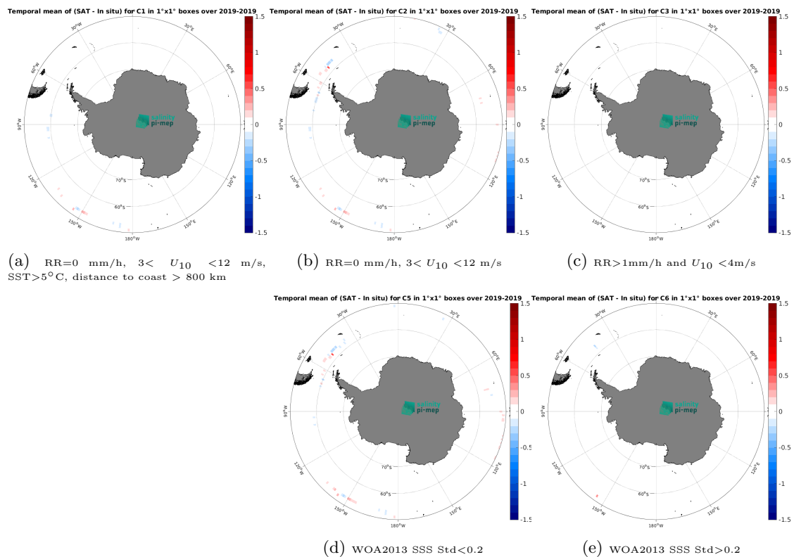
Figure 14: Temporal mean gridded over spatial boxes of size 1^\circ \times 1^\circ of \Delta SSS (SMAP SSS L4 OI v3 - Monthly (ESR) - Saildrone) for 5 different subdatasets corresponding to:RR=0 mm/h, 3 < U_{10} < 12 m/s, SST >5^\circ C, distance to coast > 800 km (a), RR=0 mm/h, 3 < U_{10} < 12 m/s (b), RR >1 mm/h and U_{10} < 4 m/s (c), WOA2013 SSS Std <0.2 (d), WOA2013 SSS Std >0.2 (e).
