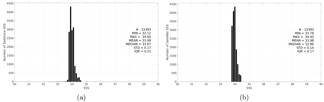
Figure 3: Histograms of SSS from Saildrone (a) and SMAP SSS L4 OI v3 - Monthly (ESR) (b) considering all match-up pairs per bins of 0.1 over the Southern Ocean Pi-MEP region and for the full satellite product period.
