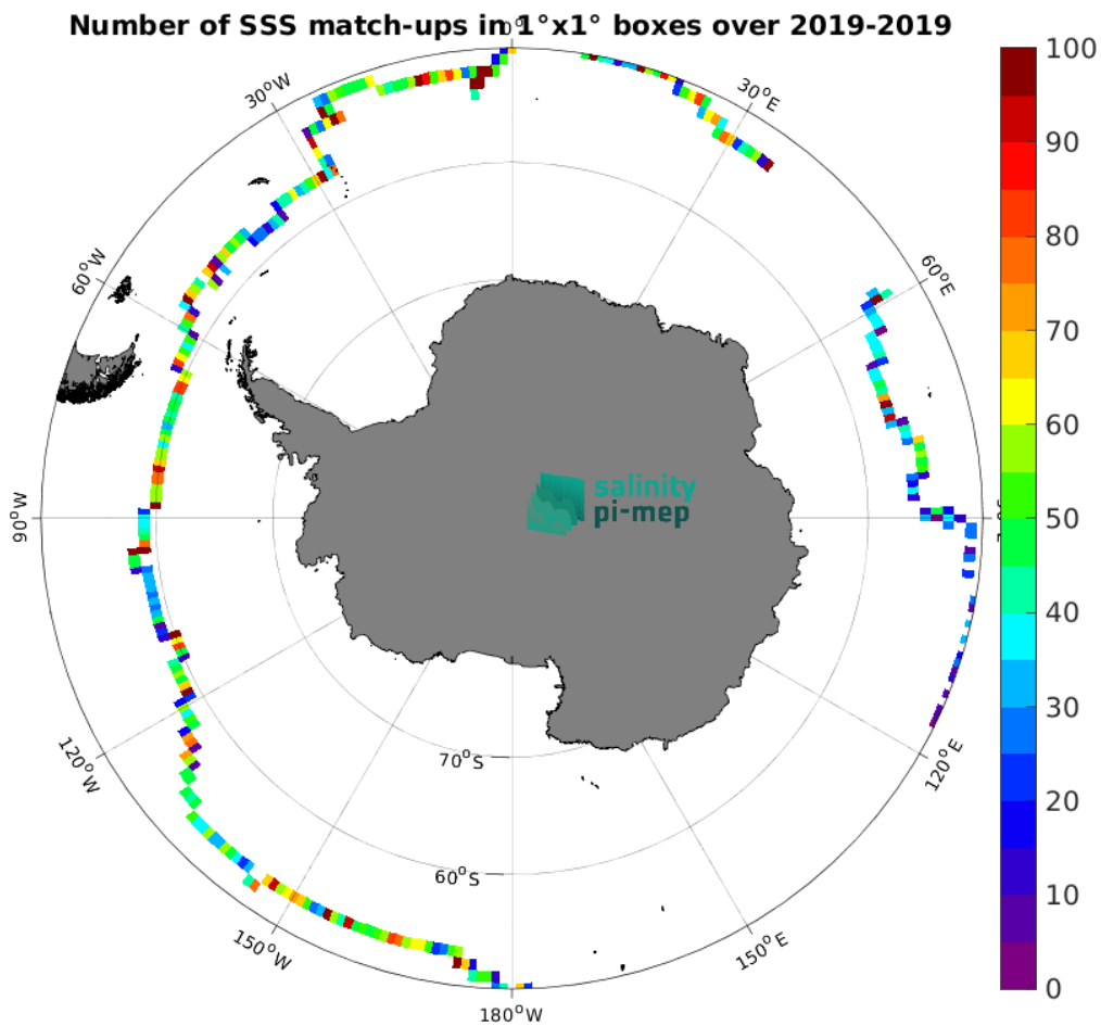
Figure 5: Number of SSS match-ups between Saildrone SSS and the SMAP SSS L4 OI v3 - Monthly (ESR) SSS product for the Southern Ocean Pi-MEP region over 1^\circ \times 1^\circ boxes and for the full satellite product period.
