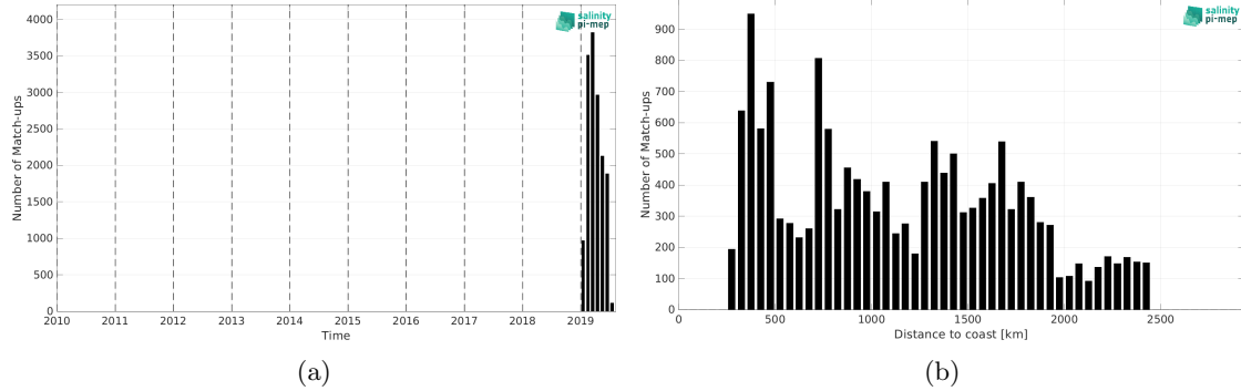
Figure 2: Number of match-ups between Saildrone and SMAP SSS L4 OI v3 - Monthly (ESR) SSS as a function of time (a) and as function of the distance to coast (b) over the Southern Ocean Pi-MEP region and for the full satellite product period.
