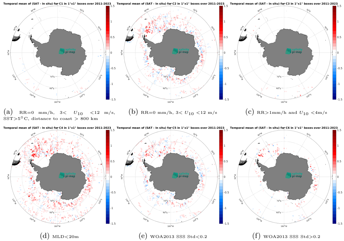
Figure 14: Temporal mean gridded over spatial boxes of size 1^\circ \times 1^\circ of \Delta\text{SSS} (SMAP SSS L4 OI v3 - Monthly (ESR) - Argo) for 6 different subdatasets corresponding to: RR=0 mm/h, 3 < U_{10} < 12 m/s, SST > 5°C, distance to coast > 800 km (a), RR=0 mm/h, 3 < U_{10} < 12 m/s (b), RR > 1mm/h and U_{10} < 4 m/s (c), MLD < 20m (d), WOA2013 SSS Std < 0.2 (e), WOA2013 SSS Std > 0.2 (f).
