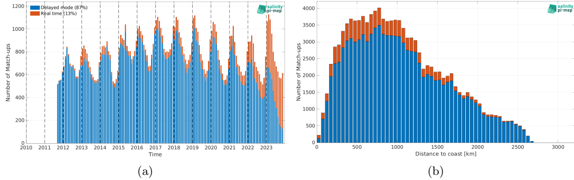
Figure 2: Number of match-ups between Argo and SMAP SSS L4 OI v3 - Monthly (ESR) SSS as a function of time (a) and as function of the distance to coast (b) over the Southern Ocean Pi-MEP region and for the full satellite product period.
