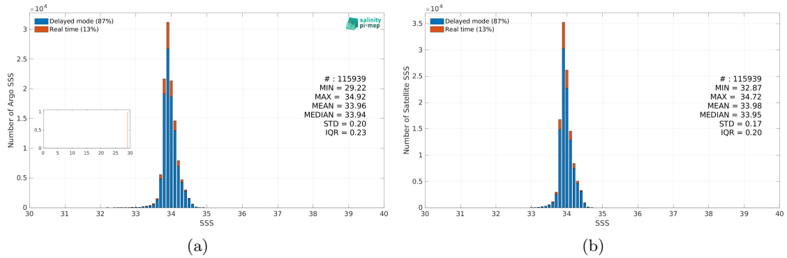
Figure 3: Histograms of SSS from Argo (a) and SMAP SSS L4 OI v3 - Monthly (ESR) (b) considering all match-up pairs per bins of 0.1 over the Southern Ocean Pi-MEP region and for the full satellite product period.
