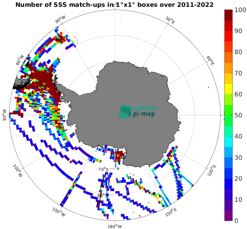
Figure 5: Number of SSS match-ups between TSG (SAMOS) SSS and the SMAP SSS L4 OI v3 - Daily (ESR) SSS product for the Southern Ocean Pi-MEP region over 1^\circ \times 1^\circ boxes and for the full satellite product period.
