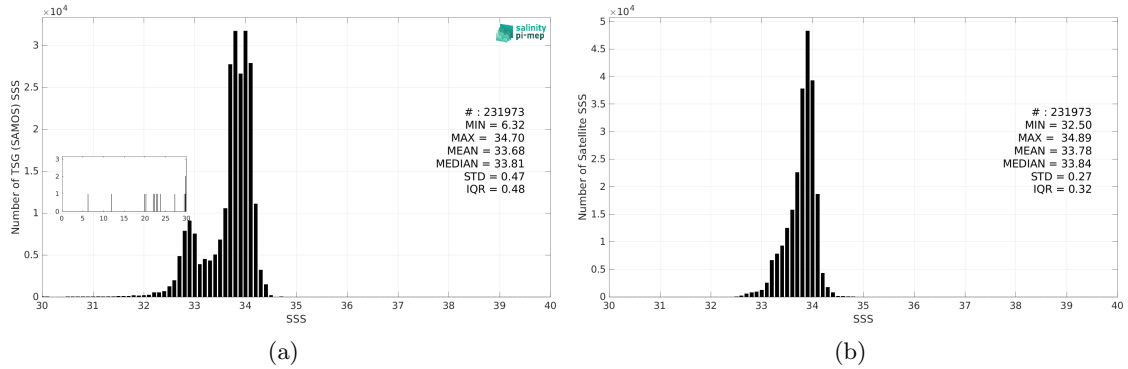
Figure 3: Histograms of SSS from TSG (SAMOS) (a) and SMAP SSS L4 OI v3 - Daily (ESR) (b) considering all match-up pairs per bins of 0.1 over the Southern Ocean Pi-MEP region and for the full satellite product period.
