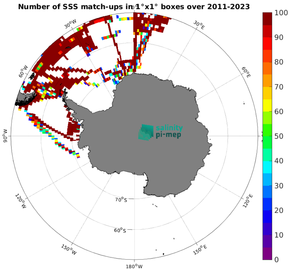
Figure 5: Number of SSS match-ups between TSG (Polarstern) SSS and the SMAP SSS L4 OI v3 - Daily (ESR) SSS product for the Southern Ocean Pi-MEP region over 1^\circ \times 1^\circ boxes and for the full satellite product period.
