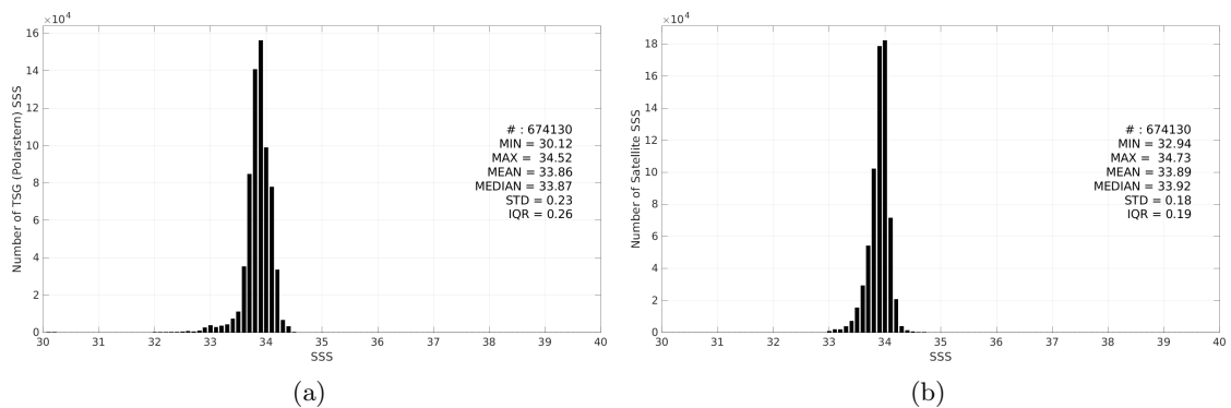
Figure 3: Histograms of SSS from TSG (Polarstern) (a) and SMAP SSS L4 OI v3 - Daily (ESR) (b) considering all match-up pairs per bins of 0.1 over the Southern Ocean Pi-MEP region and for the full satellite product period.
