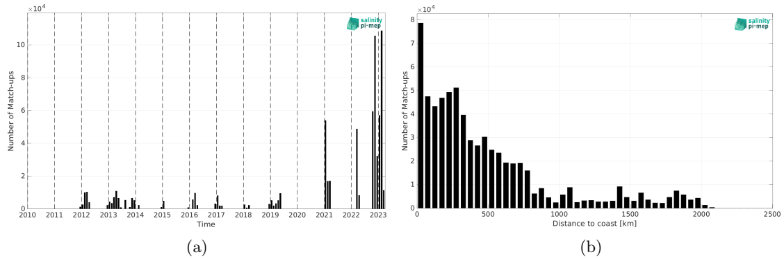
Figure 2: Number of match-ups between TSG (Polarstern) and SMAP SSS L4 OI v3 - Daily (ESR) SSS as a function of time (a) and as function of the distance to coast (b) over the Southern Ocean Pi-MEP region and for the full satellite product period.
