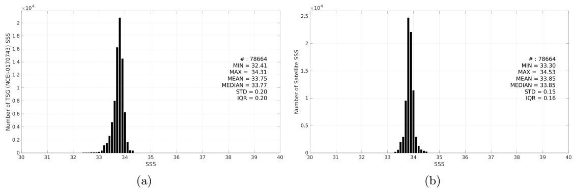
Figure 3: Histograms of SSS from TSG (NCEI-0170743) (a) and SMAP SSS L4 OI v3 - Daily (ESR) (b) considering all match-up pairs per bins of 0.1 over the Southern Ocean Pi-MEP region and for the full satellite product period.
