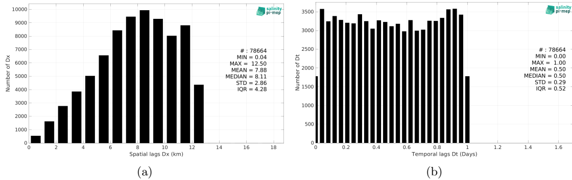
Figure 6: Histograms of the spatial (a) and temporal (b) lags between the location/time of the TSG (NCEI-0170743) measurement and the date of the corresponding SMAP SSS L4 OI v3 - Daily (ESR) SSS pixel.
