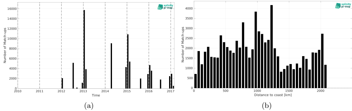
Figure 2: Number of match-ups between TSG (NCEI-0170743) and SMAP SSS L4 OI v3 - Daily (ESR) SSS as a function of time (a) and as function of the distance to coast (b) over the Southern Ocean Pi-MEP region and for the full satellite product period.
