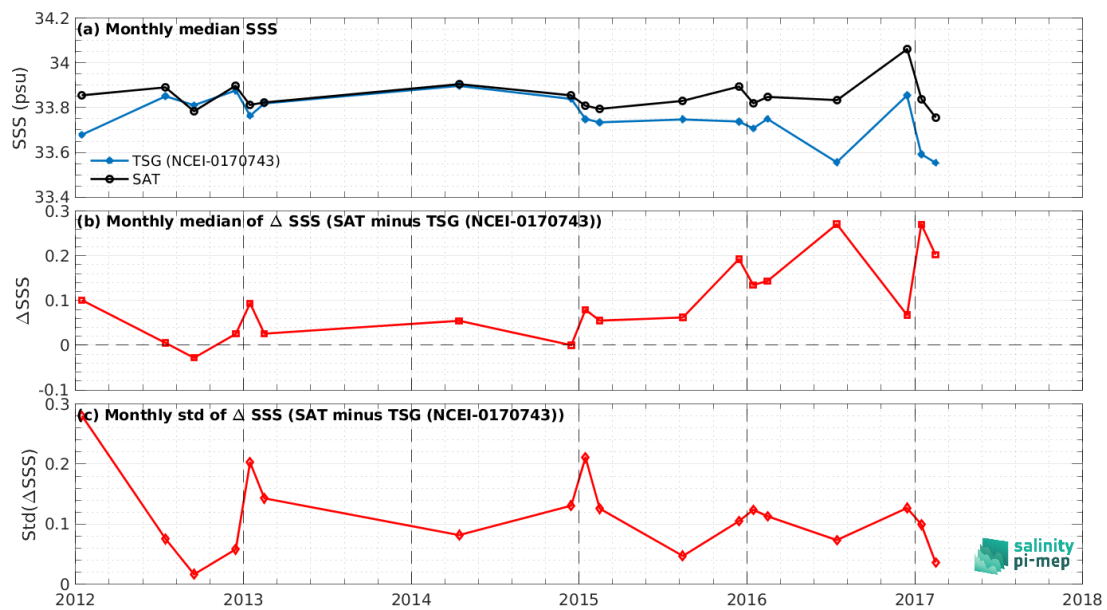
Figure 8: Time series of the monthly median SSS (top), median of \Delta SSS (Satellite - TSG (NCEI-0170743)) and Std of \Delta SSS (Satellite - TSG (NCEI-0170743)) over the Southern Ocean Pi-MEP region considering all match-ups collected by the Pi-MEP.
