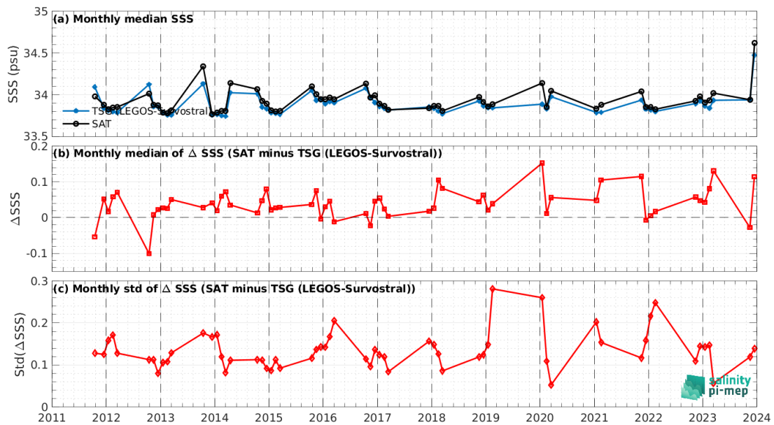
Figure 8: Time series of the monthly median SSS (top), median of \Delta SSS (Satellite - TSG (LEGOS-Survostral)) and Std of \Delta SSS (Satellite - TSG (LEGOS-Survostral)) over the Southern Ocean Pi-MEP region considering all match-ups collected by the Pi-MEP.
