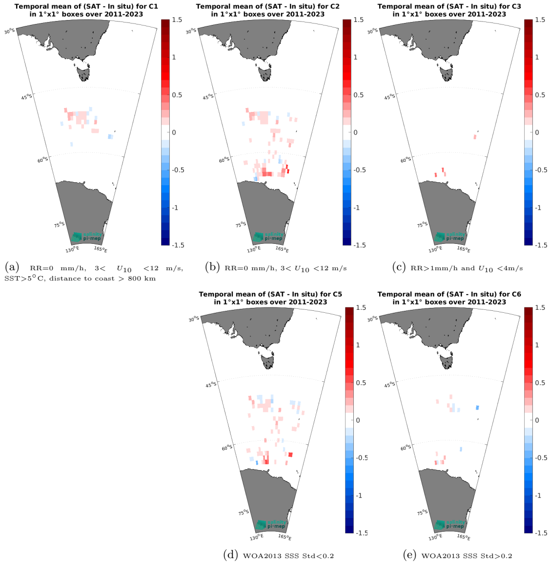
Figure 14: Temporal mean gridded over spatial boxes of size 1^\circ \times 1^\circ of \Delta SSS (SMAP SSS L4 OI v3 - Daily (ESR) - TSG (LEGOS-Survostral)) for 5 different subdatasets corresponding to:RR=0 mm/h, 3 < U_{10} < 12 m/s, SST>5°C, distance to coast > 800 km (a), RR=0 mm/h, 3 < U_{10} < 12 m/s (b), RR>1mm/h and U_{10} < 4 m/s (c), WOA2013 SSS Std<0.2 (d), WOA2013 SSS Std>0.2 (e).
