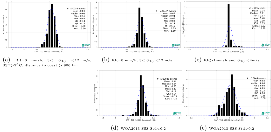
Figure 15: Normalized histogram of \Delta\text{SSS} (SMAP SSS L4 OI v3 - Daily (ESR) - TSG (LEGOS-Survostral)) for 5 different subdatasets corresponding to: RR=0 mm/h, 3 < U_{10} < 12 m/s, SST>5°C, distance to coast > 800 km (a), RR=0 mm/h, 3 < U_{10} < 12 m/s (b), RR>1mm/h and U_{10} < 4 m/s (c), WOA2013 SSS Std<0.2 (d), WOA2013 SSS Std>0.2 (e).
