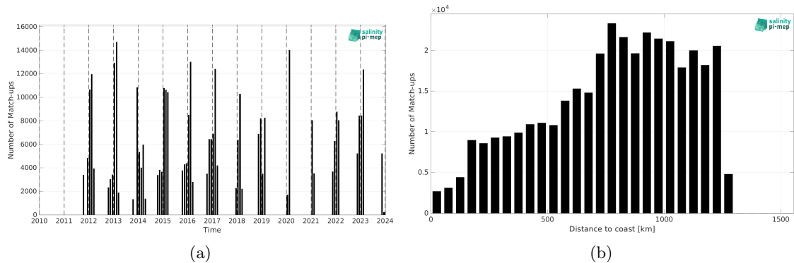
Figure 2: Number of match-ups between TSG (LEGOS-Survostral) and SMAP SSS L4 OI v3 - Daily (ESR) SSS as a function of time (a) and as function of the distance to coast (b) over the Southern Ocean Pi-MEP region and for the full satellite product period.
