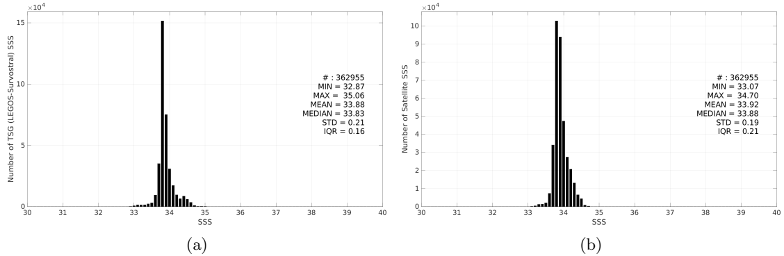
Figure 3: Histograms of SSS from TSG (LEGOS-Survostral) (a) and SMAP SSS L4 OI v3 - Daily (ESR) (b) considering all match-up pairs per bins of 0.1 over the Southern Ocean Pi-MEP region and for the full satellite product period.
