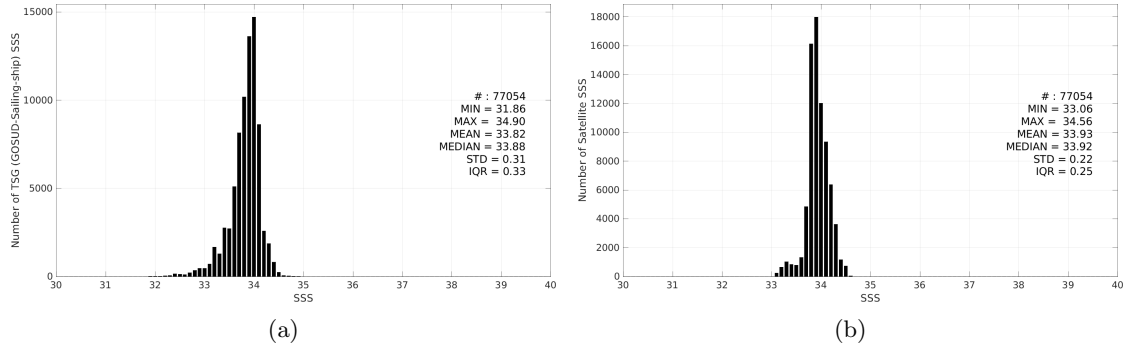
Figure 3: Histograms of SSS from TSG (GOSUD-Sailing-ship) (a) and SMAP SSS L4 OI v3 - Daily (ESR) (b) considering all match-up pairs per bins of 0.1 over the Southern Ocean Pi-MEP region and for the full satellite product period.
