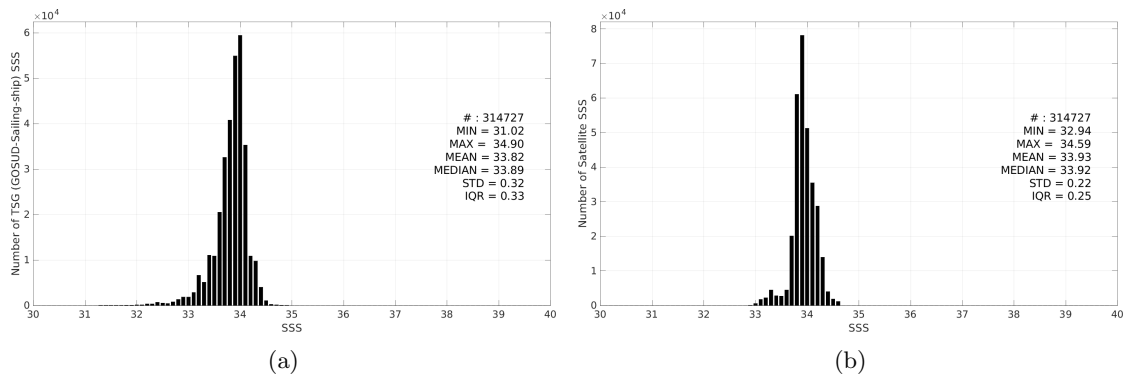
Figure 3: Histograms of SSS from TSG (GOSUD-Sailing-ship) (a) and SMAP SSS L4 OI v3 - Daily (ESR) (b) considering all match-up pairs per bins of 0.1 over the Southern Ocean Pi-MEP region and for the full satellite product period.
