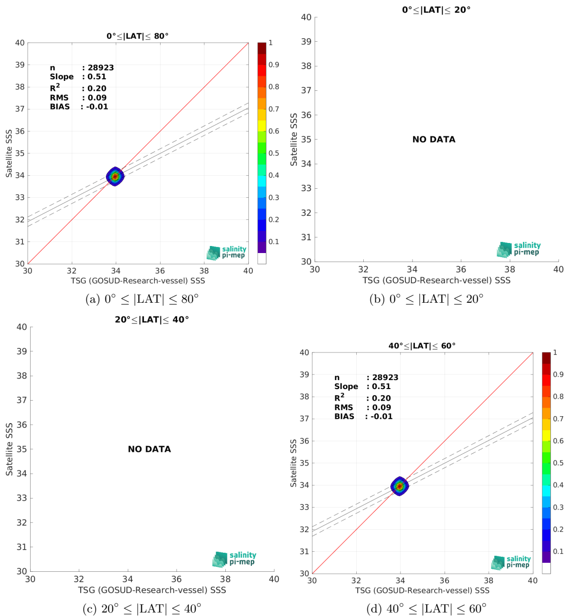
Figure 10: Contour maps of the concentration of SMAP SSS L4 OI v3 - Daily (ESR) SSS (y-axis) versus TSG (GOSUD-Research-vessel) SSS (x-axis) at match-up pairs for different latitude bands. For each plot, the red line shows x=y . The black thin and dashed lines indicate a linear fit through the data cloud and the \pm 95\% confidence levels, respectively. The number match-up pairs n , the slope and R^2 coefficient of the linear fit, the root mean square (RMS) and the mean bias between satellite and in situ data are indicated for each latitude band in each plots.
