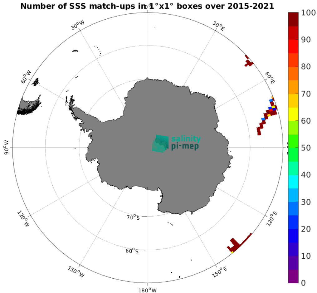
Figure 5: Number of SSS match-ups between TSG (GOSUD-Research-vessel) SSS and the SMAP SSS L4 OI v3 - Daily (ESR) SSS product for the Southern Ocean Pi-MEP region over 1^\circ \times 1^\circ boxes and for the full satellite product period.
