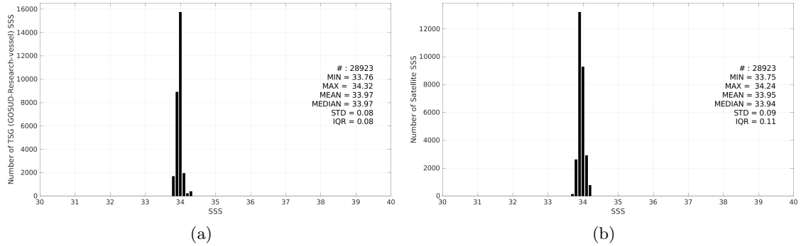
Figure 3: Histograms of SSS from TSG (GOSUD-Research-vessel) (a) and SMAP SSS L4 OI v3 - Daily (ESR) (b) considering all match-up pairs per bins of 0.1 over the Southern Ocean Pi-MEP region and for the full satellite product period.
