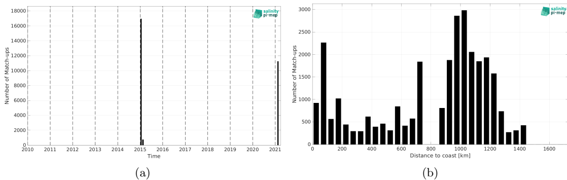
Figure 2: Number of match-ups between TSG (GOSUD-Research-vessel) and SMAP SSS L4 OI v3 - Daily (ESR) SSS as a function of time (a) and as function of the distance to coast (b) over the Southern Ocean Pi-MEP region and for the full satellite product period.
