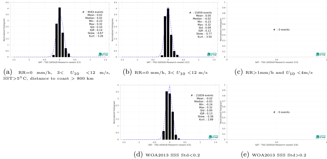
Figure 15: Normalized histogram of \Delta SSS (SMAP SSS L4 OI v3 - Daily (ESR) - TSG (GOSUD-Research-vessel)) for 5 different subdatasets corresponding to: RR=0 mm/h, 3 < U_{10} < 12 m/s, SST > 5°C, distance to coast > 800 km (a), RR=0 mm/h, 3 < U_{10} < 12 m/s (b), RR > 1mm/h and U_{10} < 4 m/s (c), WOA2013 SSS Std < 0.2 (d), WOA2013 SSS Std > 0.2 (e).
