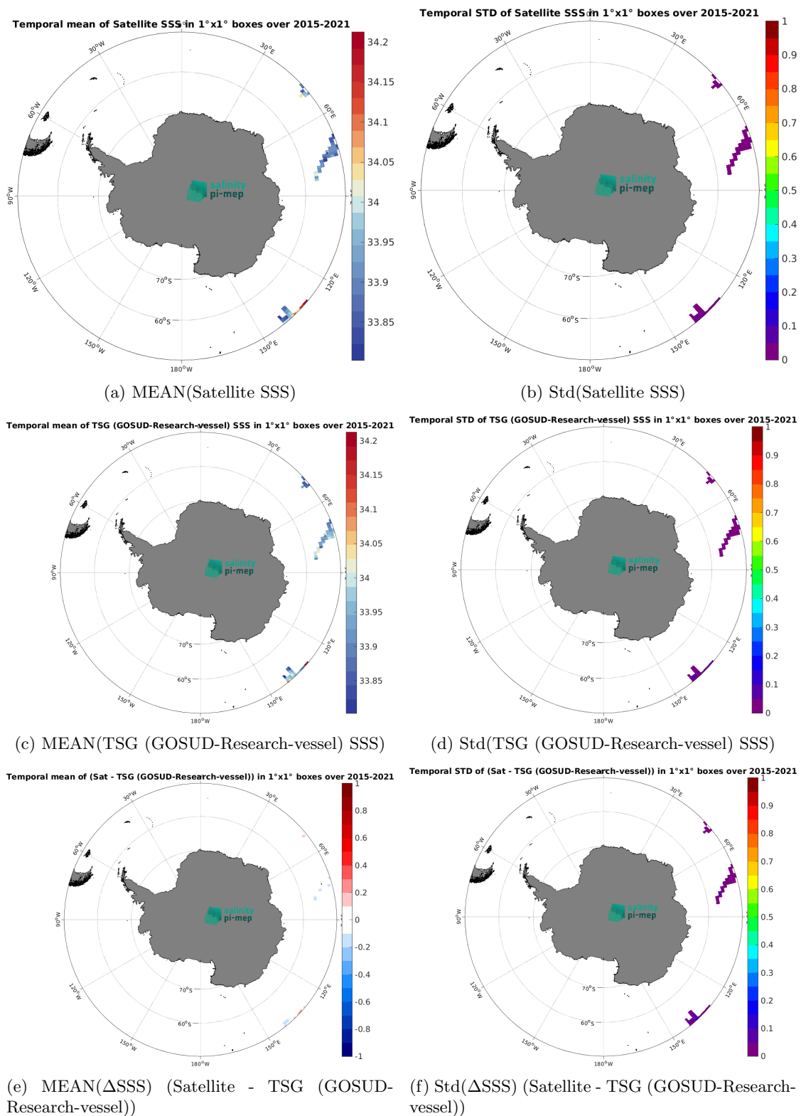
Figure 7: Temporal mean (left) and Std (right) of SSS from SMAP SSS L4 OI v3 - Daily (ESR) (top), TSG (GOSUD-Research-vessel) (middle), and of \Delta SSS (Satellite - TSG (GOSUD-Research-vessel)). Only match-up pairs are used to generate these maps.
