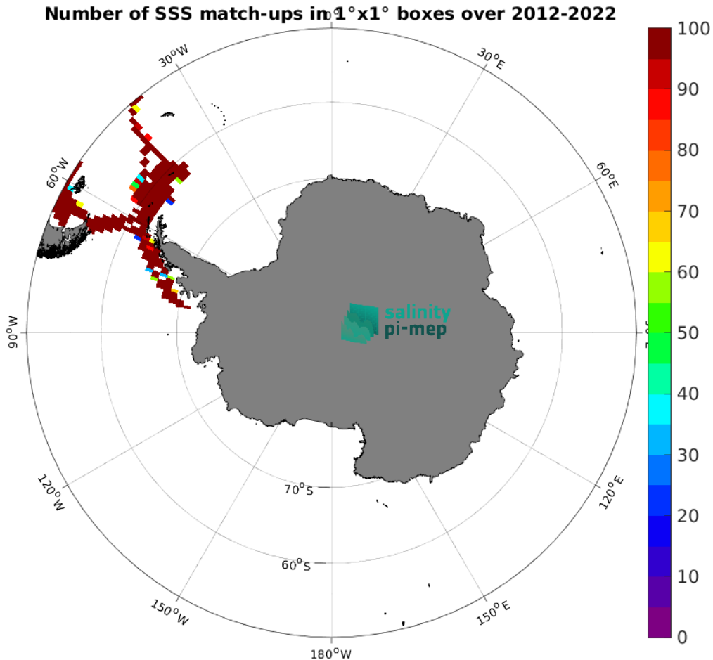
Figure 5: Number of SSS match-ups between TSG (CSIC-UTM) SSS and the SMAP SSS L4 OI v3 - Daily (ESR) SSS product for the Southern Ocean Pi-MEP region over 1^\circ \times 1^\circ boxes and for the full satellite product period.
