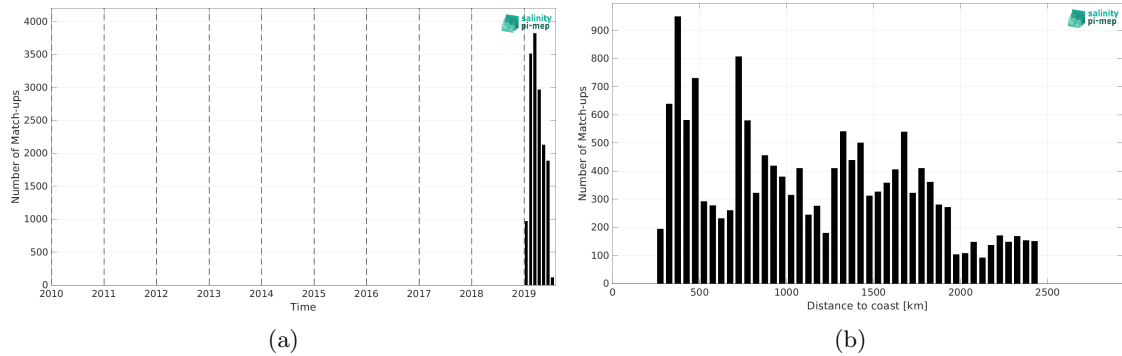
Figure 2: Number of match-ups between Saildrone and SMAP SSS L4 OI v3 - Daily (ESR) SSS as a function of time (a) and as function of the distance to coast (b) over the Southern Ocean Pi-MEP region and for the full satellite product period.
