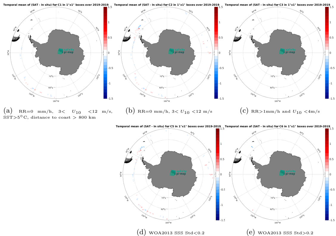
Figure 14: Temporal mean gridded over spatial boxes of size 1^\circ \times 1^\circ of \Delta\text{SSS} (SMAP SSS L4 OI v3 - Daily (ESR) - Saildrone) for 5 different subdatasets corresponding to:RR=0 mm/h, 3 < U_{10} < 12 m/s, SST>5°C, distance to coast > 800 km (a), RR=0 mm/h, 3 < U_{10} < 12 m/s (b), RR>1mm/h and U_{10} < 4 m/s (c), WOA2013 SSS Std<0.2 (d), WOA2013 SSS Std>0.2 (e).
