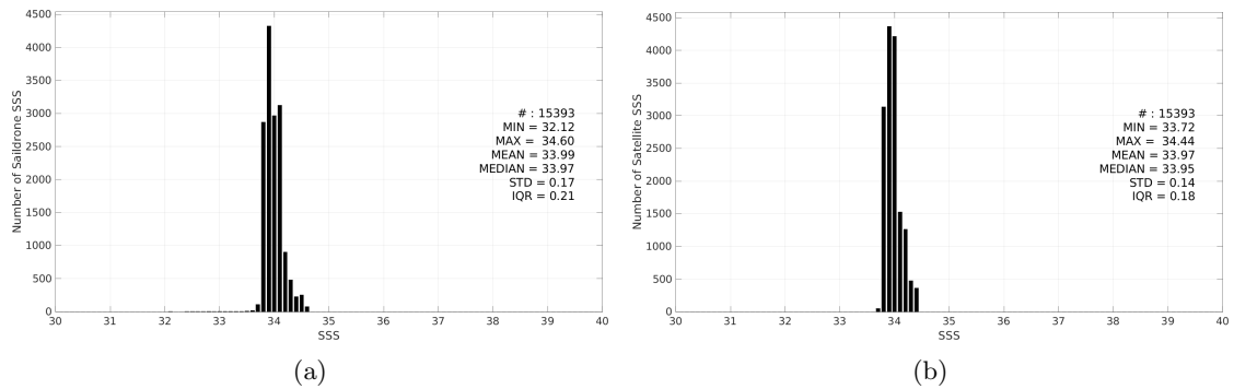
Figure 3: Histograms of SSS from Saildrone (a) and SMAP SSS L4 OI v3 - Daily (ESR) (b) considering all match-up pairs per bins of 0.1 over the Southern Ocean Pi-MEP region and for the full satellite product period.
