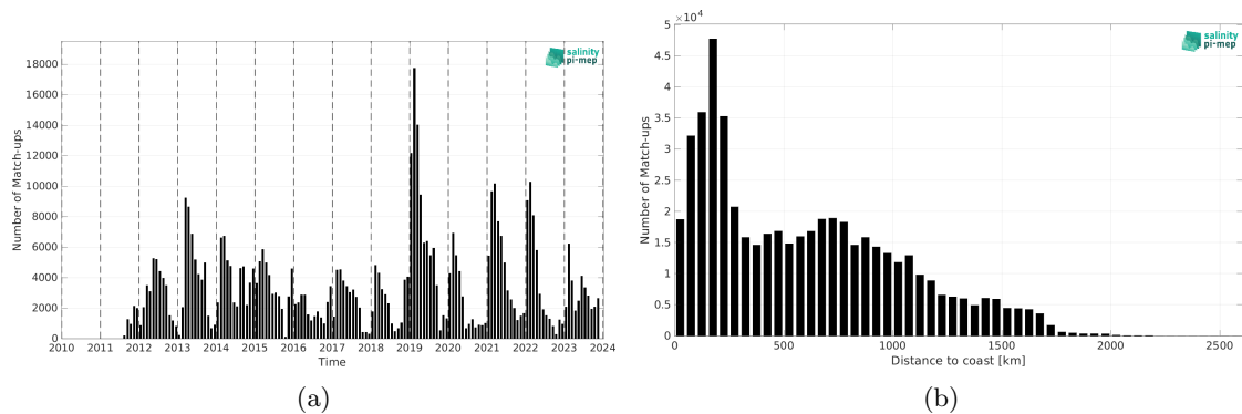
Figure 2: Number of match-ups between Marine mammals and SMAP SSS L4 OI v3 - Daily (ESR) SSS as a function of time (a) and as function of the distance to coast (b) over the Southern Ocean Pi-MEP region and for the full satellite product period.
