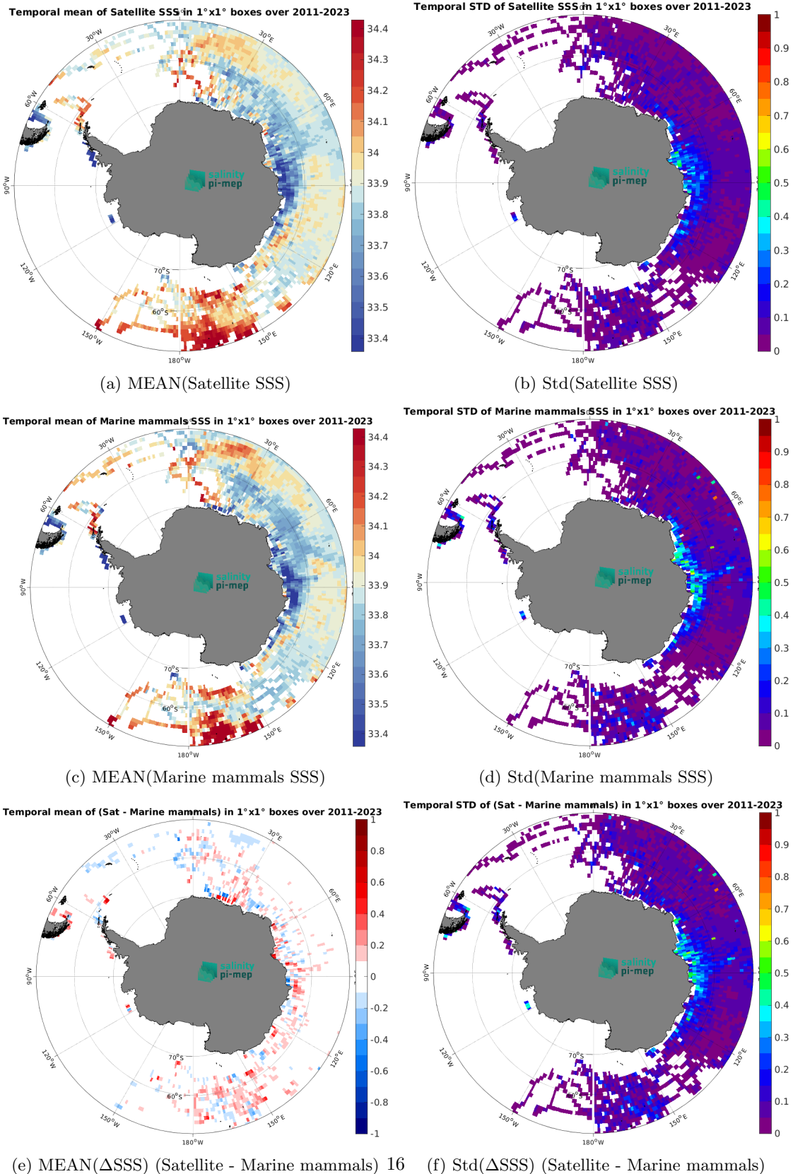
Figure 7: Temporal mean (left) and Std (right) of SSS from SMAP SSS L4 OI v3 - Daily (ESR) (top), Marine mammals (middle), and of \Delta SSS (Satellite - Marine mammals). Only match-up pairs are used to generate these maps.
