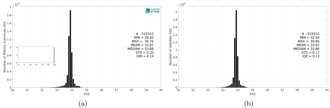
Figure 3: Histograms of SSS from Marine mammals (a) and SMAP SSS L4 OI v3 - Daily (ESR) (b) considering all match-up pairs per bins of 0.1 over the Southern Ocean Pi-MEP region and for the full satellite product period.
