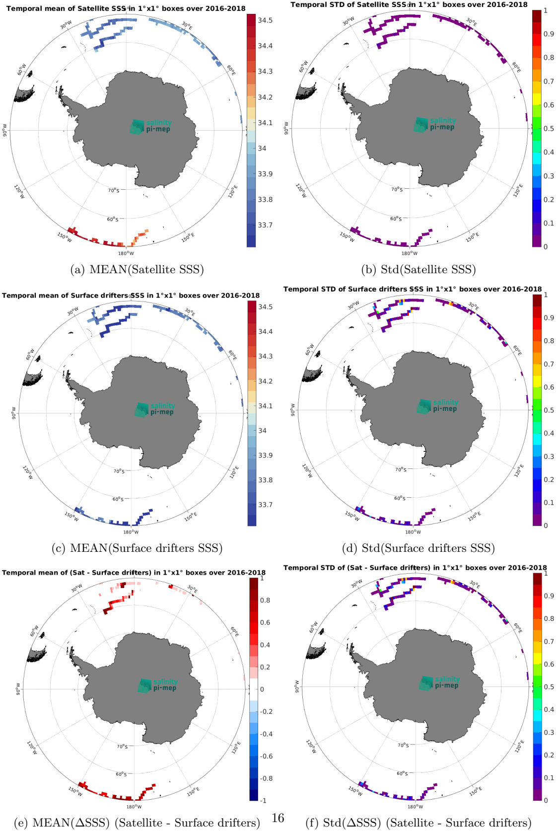
Figure 6: Temporal mean (left) and Std (right) of SSS from SMAP SSS L4 OI v3 - Daily (ESR) (top), Surface drifters (middle), and of \Delta SSS (Satellite - Surface drifters). Only match-up pairs are used to generate these maps.
