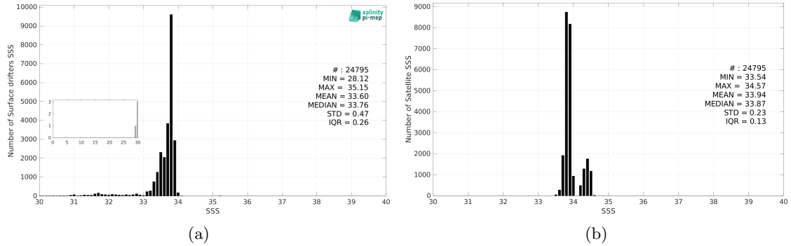
Figure 3: Histograms of SSS from Surface drifters (a) and SMAP SSS L4 OI v3 - Daily (ESR) (b) considering all match-up pairs per bins of 0.1 over the Southern Ocean Pi-MEP region and for the full satellite product period.
