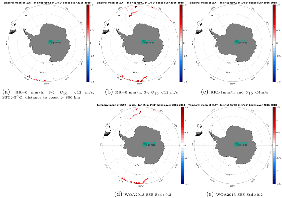
Figure 13: Temporal mean gridded over spatial boxes of size 1^\circ \times 1^\circ of \Delta SSS (SMAP SSS L4 OI v3 - Daily (ESR) - Surface drifters) for 5 different subdatasets corresponding to:RR=0 mm/h, 3 < U_{10} < 12 m/s, SST >5^\circ C, distance to coast > 800 km (a), RR=0 mm/h, 3 < U_{10} < 12 m/s (b), RR >1 mm/h and U_{10} < 4 m/s (c), WOA2013 SSS Std <0.2 (d), WOA2013 SSS Std >0.2 (e).
