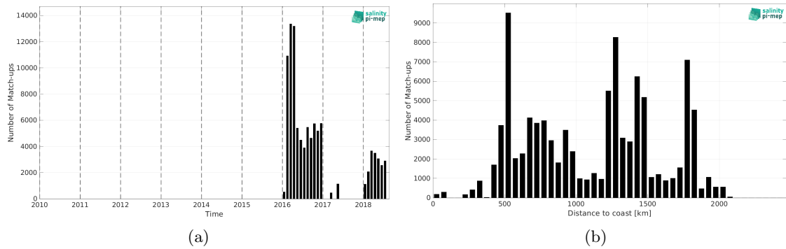
Figure 2: Number of match-ups between Surface drifters and SMAP SSS L4 OI v3 - Daily (ESR) SSS as a function of time (a) and as function of the distance to coast (b) over the Southern Ocean Pi-MEP region and for the full satellite product period.
