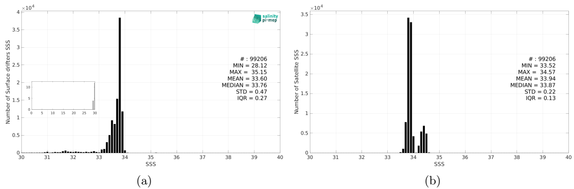
Figure 3: Histograms of SSS from Surface drifters (a) and SMAP SSS L4 OI v3 - Daily (ESR) (b) considering all match-up pairs per bins of 0.1 over the Southern Ocean Pi-MEP region and for the full satellite product period.
