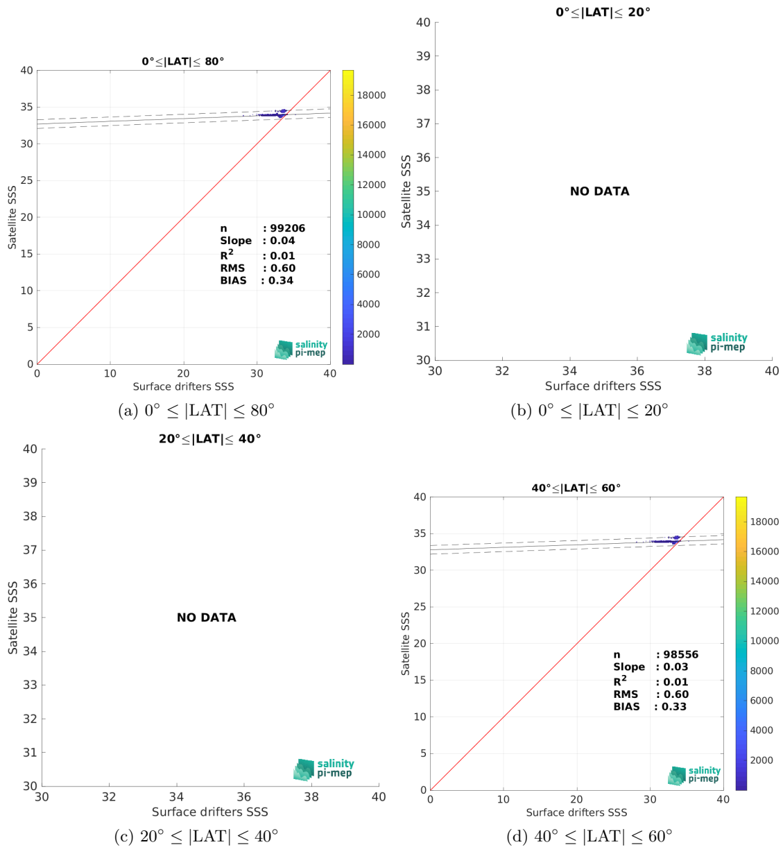
Figure 9: Contour maps of the concentration of SMAP SSS L4 OI v3 - Daily (ESR) SSS (y-axis) versus Surface drifters SSS (x-axis) at match-up pairs for different latitude bands. For each plot, the red line shows x=y . The black thin and dashed lines indicate a linear fit through the data cloud and the \pm 95\% confidence levels, respectively. The number match-up pairs n , the slope and R^2 coefficient of the linear fit, the root mean square (RMS) and the mean bias between satellite and in situ data are indicated for each latitude band in each plots.
