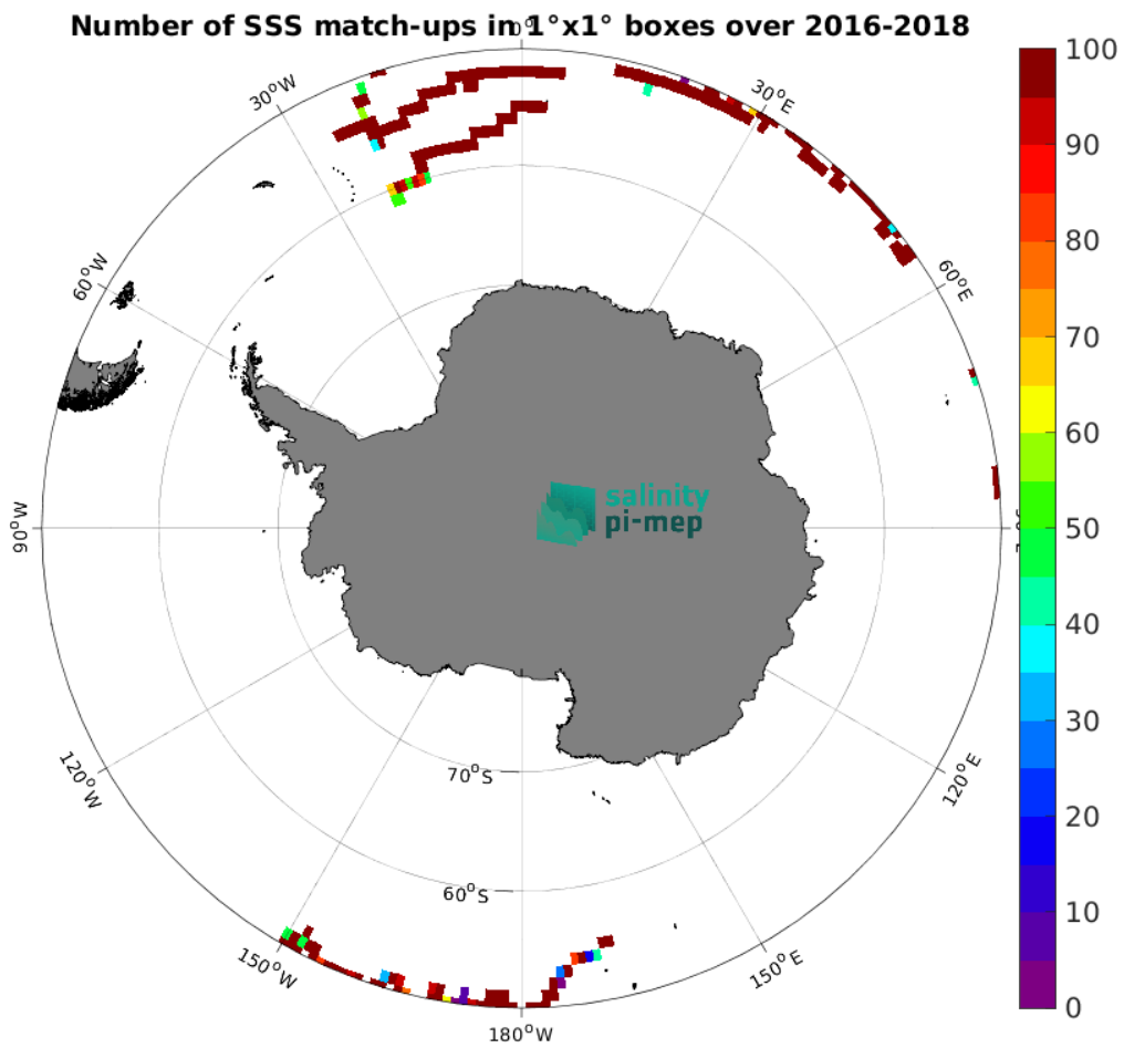
Figure 4: Number of SSS match-ups between Surface drifters SSS and the SMAP SSS L4 OI v3 - Daily (ESR) SSS product for the Southern Ocean Pi-MEP region over 1^\circ \times 1^\circ boxes and for the full satellite product period.
