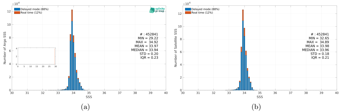
Figure 3: Histograms of SSS from Argo (a) and SMAP SSS L4 OI v3 - Daily (ESR) (b) considering all match-up pairs per bins of 0.1 over the Southern Ocean Pi-MEP region and for the full satellite product period.
