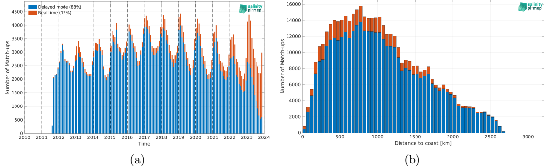
Figure 2: Number of match-ups between Argo and SMAP SSS L4 OI v3 - Daily (ESR) SSS as a function of time (a) and as function of the distance to coast (b) over the Southern Ocean Pi-MEP region and for the full satellite product period.
