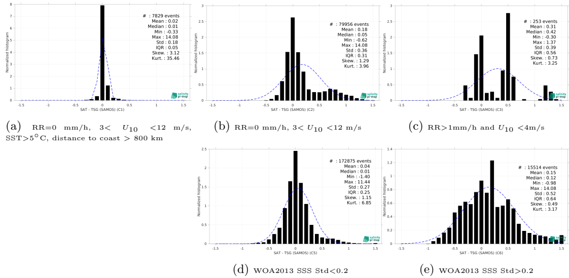
Figure 13: Normalized histogram of \Delta\text{SSS} (SMAP SSS L4 OI v2 - 7 Days (ESR) - TSG (SAMOS)) for 5 different subdatasets corresponding to: RR=0 mm/h, 3 < U_{10} < 12 m/s, SST > 5^{\circ}\text{C} , distance to coast > 800 km (a), RR=0 mm/h, 3 < U_{10} < 12 m/s (b), RR > 1\text{mm/h} and U_{10} < 4\text{m/s} (c), WOA2013 SSS Std < 0.2 (d), WOA2013 SSS Std > 0.2 (e).
