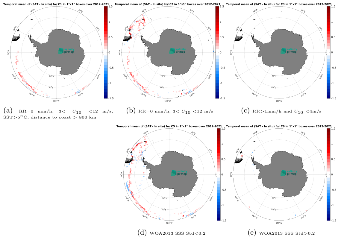
Figure 12: Temporal mean gridded over spatial boxes of size 1^{\circ} \times 1^{\circ} of \Delta SSS (SMAP SSS L4 OI v2 - 7 Days (ESR) - TSG (GOSUD-Sailing-ship)) for 5 different subdatasets corresponding to: RR=0 mm/h, 3 < U_{10} < 12 m/s, SST>5°C, distance to coast > 800 km (a), RR=0 mm/h, 3 < U_{10} < 12 m/s (b), RR>1mm/h and U_{10} < 4 m/s (c), WOA2013 SSS Std<0.2 (d), WOA2013 SSS Std>0.2 (e).
