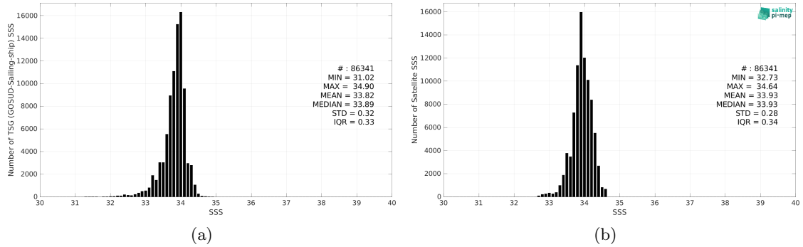
Figure 2: Histograms of SSS from TSG (GOSUD-Sailing-ship) (a) and SMAP SSS L4 OI v2 - 7 Days (ESR) (b) considering all match-up pairs per bins of 0.1 over the Southern Ocean Pi-MEP region and for the full satellite product period.
