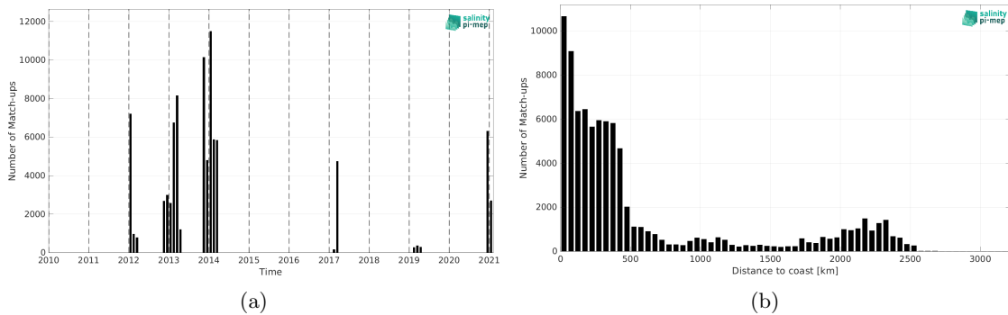
Figure 1: Number of match-ups between TSG (GOSUD-Sailing-ship) and SMAP SSS L4 OI v2 - 7 Days (ESR) SSS as a function of time (a) and as function of the distance to coast (b) over the Southern Ocean Pi-MEP region and for the full satellite product period.
