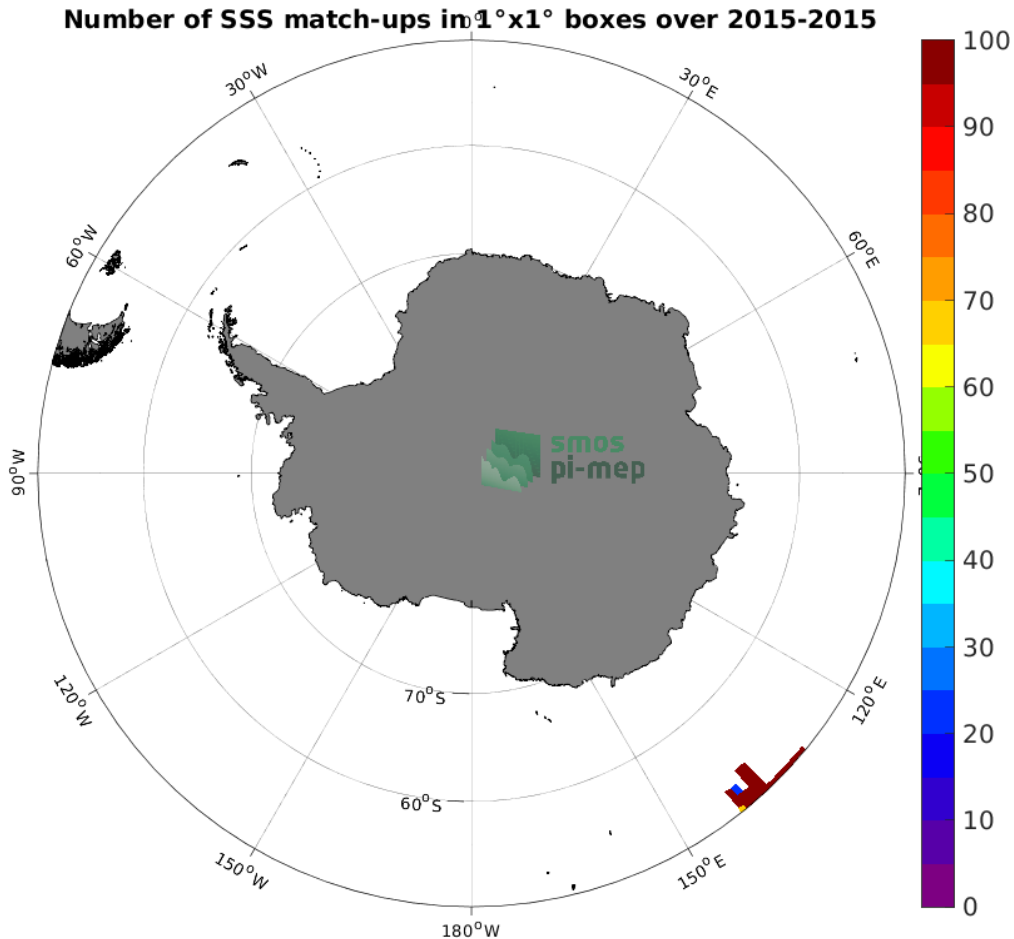
Figure 4: Number of SSS match-ups between TSG (GOSUD-Research-vessel) SSS and the SMAP SSS L4 OI v2 - 7 Days (ESR) SSS product for the Southern Ocean Pi-MEP region over 1^\circ \times 1^\circ boxes and for the full satellite product period.
