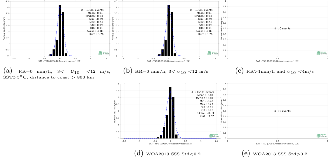
Figure 13: Normalized histogram of \Delta SSS (SMAP SSS L4 OI v2 - 7 Days (ESR) - TSG (GOSUD-Research-vessel)) for 5 different subdatasets corresponding to: RR=0 mm/h, 3 < U_{10} < 12 m/s, SST>5°C, distance to coast > 800 km (a), RR=0 mm/h, 3 < U_{10} < 12 m/s (b), RR>1mm/h and U_{10} < 4 m/s (c), WOA2013 SSS Std<0.2 (d), WOA2013 SSS Std>0.2 (e).
