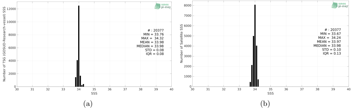
Figure 2: Histograms of SSS from TSG (GOSUD-Research-vessel) (a) and SMAP SSS L4 OI v2 - 7 Days (ESR) (b) considering all match-up pairs per bins of 0.1 over the Southern Ocean Pi-MEP region and for the full satellite product period.
