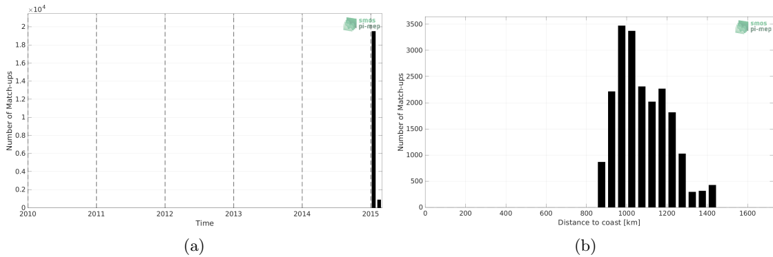
Figure 1: Number of match-ups between TSG (GOSUD-Research-vessel) and SMAP SSS L4 OI v2 - 7 Days (ESR) SSS as a function of time (a) and as function of the distance to coast (b) over the Southern Ocean Pi-MEP region and for the full satellite product period.
