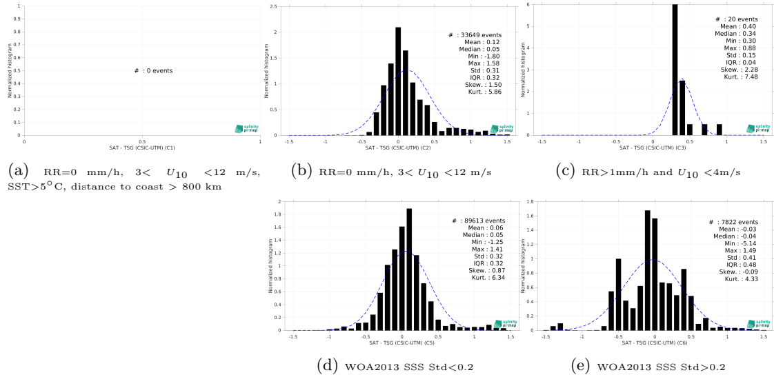
Figure 13: Normalized histogram of \Delta\text{SSS} (SMAP SSS L4 OI v2 - 7 Days (ESR) - TSG (CSIC-UTM)) for 5 different subdatasets corresponding to: RR=0 mm/h, 3 < U_{10} < 12 m/s, SST > 5^\circ\text{C} , distance to coast > 800 km (a), RR=0 mm/h, 3 < U_{10} < 12 m/s (b), RR > 1\text{mm/h} and U_{10} < 4\text{m/s} (c), WOA2013 SSS Std < 0.2 (d), WOA2013 SSS Std > 0.2 (e).
