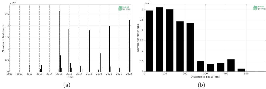
Figure 1: Number of match-ups between TSG (CSIC-UTM) and SMAP SSS L4 OI v2 - 7 Days (ESR) SSS as a function of time (a) and as function of the distance to coast (b) over the Southern Ocean Pi-MEP region and for the full satellite product period.
