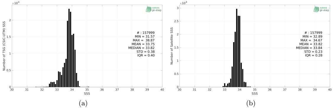
Figure 2: Histograms of SSS from TSG (CSIC-UTM) (a) and SMAP SSS L4 OI v2 - 7 Days (ESR) (b) considering all match-up pairs per bins of 0.1 over the Southern Ocean Pi-MEP region and for the full satellite product period.
