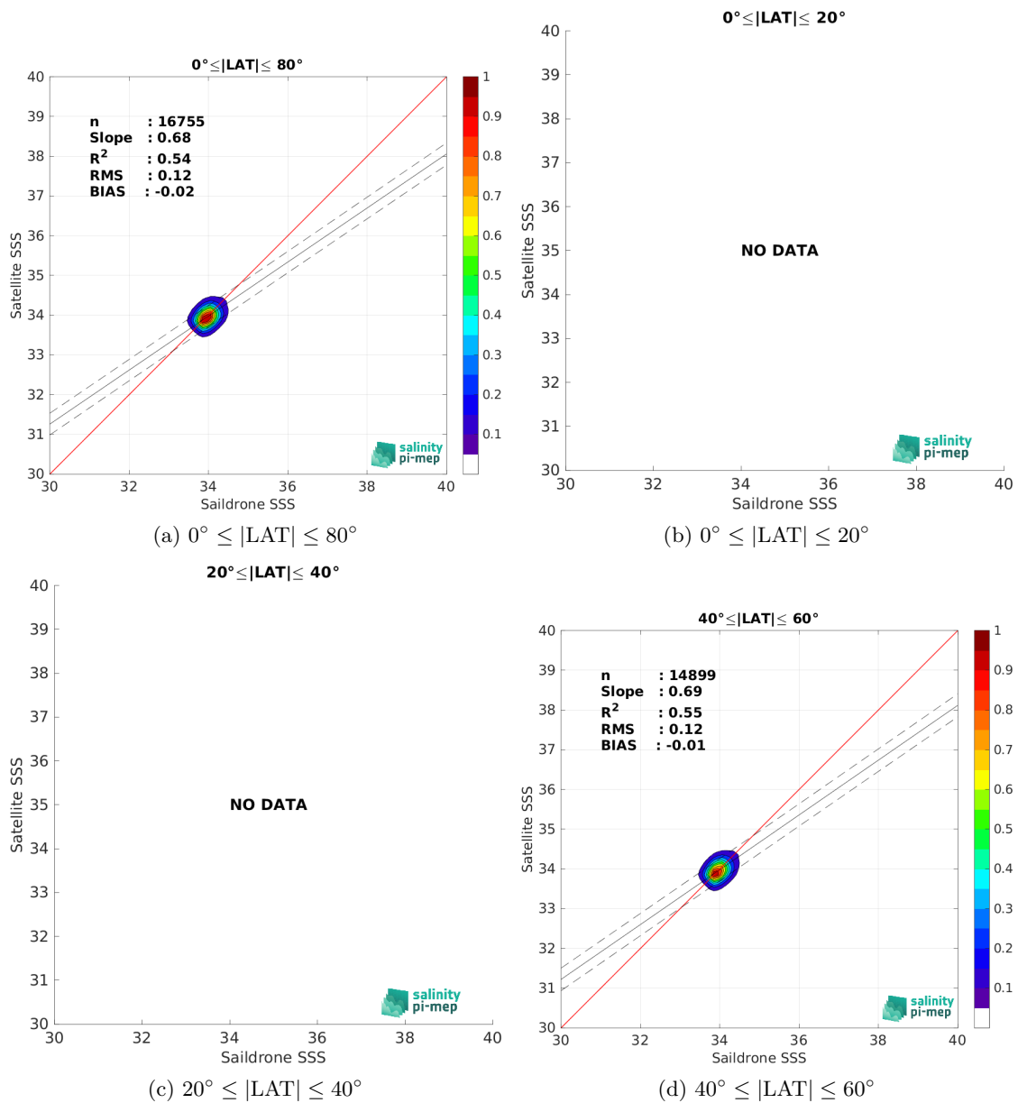
Figure 9: Contour maps of the concentration of SMAP SSS L4 OI v2 - 7 Days (ESR) SSS (y-axis) versus Saildrone SSS (x-axis) at match-up pairs for different latitude bands. For each plot, the red line shows x=y . The black thin and dashed lines indicate a linear fit through the data cloud and the \pm 95\% confidence levels, respectively. The number match-up pairs n , the slope and R^2 coefficient of the linear fit, the root mean square (RMS) and the mean bias between satellite and in situ data are indicated for each latitude band in each plots.
