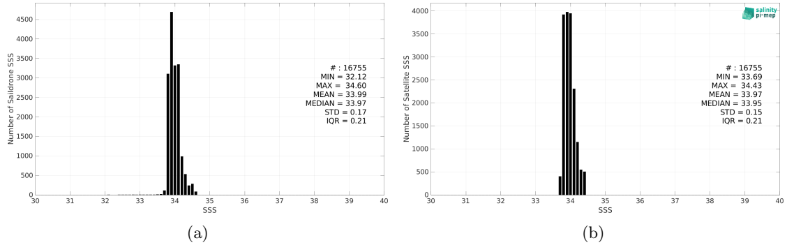
Figure 2: Histograms of SSS from Saildrone (a) and SMAP SSS L4 OI v2 - 7 Days (ESR) (b) considering all match-up pairs per bins of 0.1 over the Southern Ocean Pi-MEP region and for the full satellite product period.
