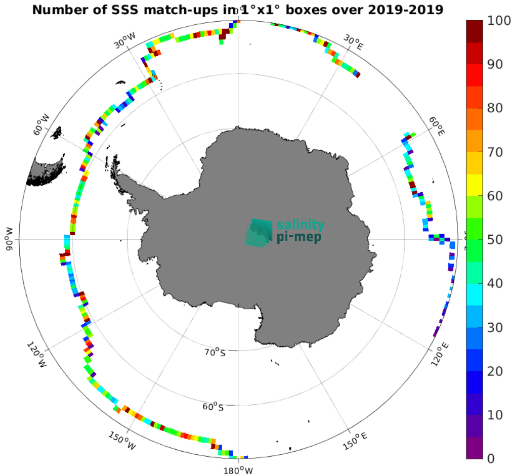
Figure 4: Number of SSS match-ups between Saildrone SSS and the SMAP SSS L4 OI v2 - 7 Days (ESR) SSS product for the Southern Ocean Pi-MEP region over 1^\circ \times 1^\circ boxes and for the full satellite product period.
