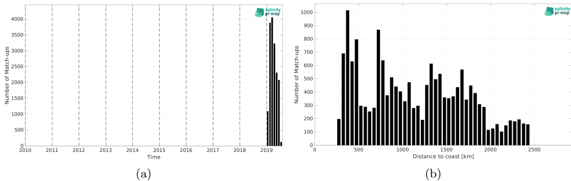
Figure 1: Number of match-ups between Saildrone and SMAP SSS L4 OI v2 - 7 Days (ESR) SSS as a function of time (a) and as function of the distance to coast (b) over the Southern Ocean Pi-MEP region and for the full satellite product period.
