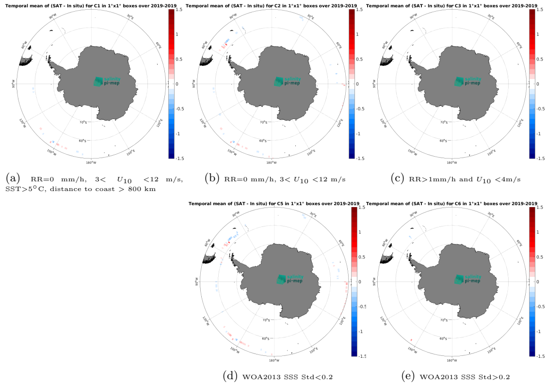
Figure 12: Temporal mean gridded over spatial boxes of size 1^{\circ}\times 1^{\circ} of \Delta\text{SSS} (SMAP SSS L4 OI v2 - 7 Days (ESR) - Saildrone) for 5 different subdatasets corresponding to:RR=0 mm/h, 3 < U_{10} < 12 m/s, SST >5^{\circ}\text{C} , distance to coast > 800 km (a), RR=0 mm/h, 3 < U_{10} < 12 m/s (b), RR >1 mm/h and U_{10} < 4 m/s (c), WOA2013 SSS Std <0.2 (d), WOA2013 SSS Std >0.2 (e).
