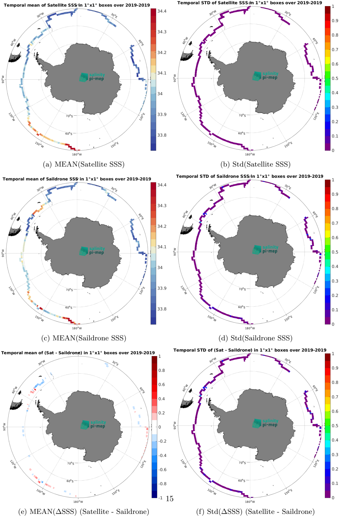
Figure 6: Temporal mean (left) and Std (right) of SSS from SMAP SSS L4 OI v2 - 7 Days (ESR) (top), Saildrone (middle), and of \Delta SSS (Satellite - Saildrone). Only match-up pairs are used to generate these maps.
