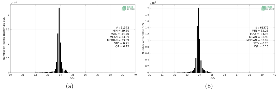
Figure 2: Histograms of SSS from Marine mammals (a) and SMAP SSS L4 OI v2 - 7 Days (ESR) (b) considering all match-up pairs per bins of 0.1 over the Southern Ocean Pi-MEP region and for the full satellite product period.
