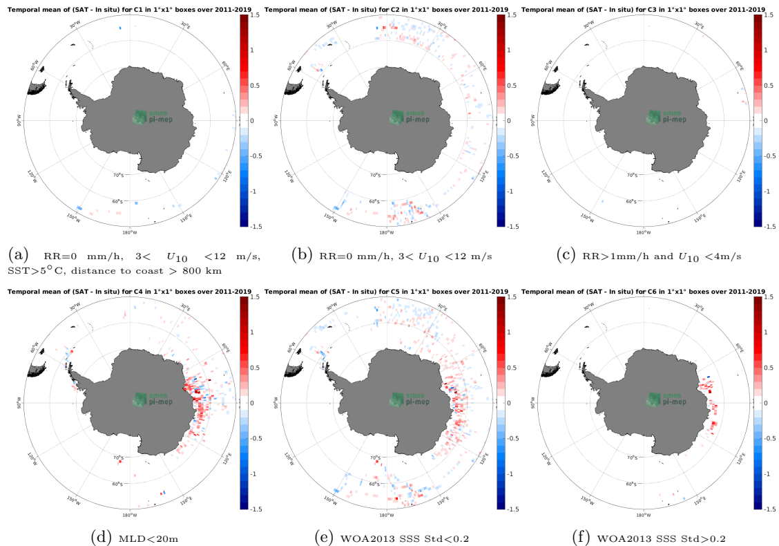
Figure 12: Temporal mean gridded over spatial boxes of size 1^{\circ}\times 1^{\circ} of \Delta\text{SSS} (SMAP SSS L4 OI v2 - 7 Days (ESR) - Marine mammals) for 6 different subdatasets corresponding to: RR=0 mm/h, 3 < U_{10} < 12 m/s, SST > 5^{\circ}\text{C} , distance to coast > 800 km (a), RR=0 mm/h, 3 < U_{10} < 12 m/s (b), RR > 1 mm/h and U_{10} < 4 m/s (c), MLD < 20\text{m} (d), WOA2013 SSS Std < 0.2 (e), WOA2013 SSS Std > 0.2 (f).
