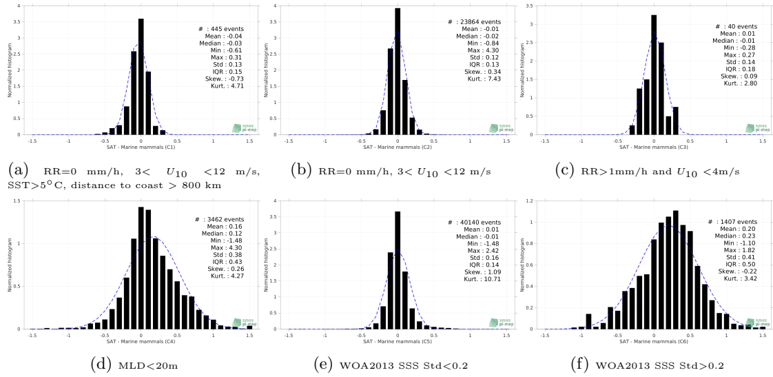
Figure 13: Normalized histogram of \Delta SSS (SMAP SSS L4 OI v2 - 7 Days (ESR) - Marine mammals) for 6 different subdatasets corresponding to: RR=0 mm/h, 3 < U_{10} < 12 m/s, SST>5°C, distance to coast > 800 km (a), RR=0 mm/h, 3 < U_{10} < 12 m/s (b), RR>1mm/h and U_{10} < 4 m/s (c), MLD<20m (d), WOA2013 SSS Std<0.2 (e), WOA2013 SSS Std>0.2 (f).
