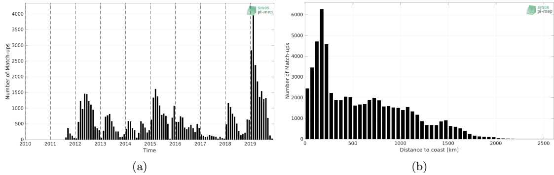
Figure 1: Number of match-ups between Marine mammals and SMAP SSS L4 OI v2 - 7 Days (ESR) SSS as a function of time (a) and as function of the distance to coast (b) over the Southern Ocean Pi-MEP region and for the full satellite product period.
