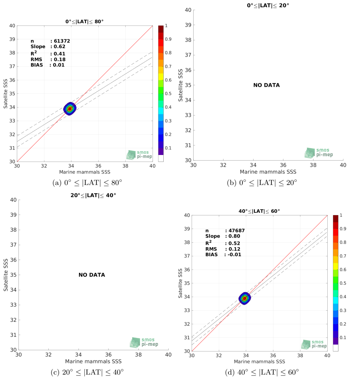
Figure 9: Contour maps of the concentration of SMAP SSS L4 OI v2 - 7 Days (ESR) SSS (y-axis) versus Marine mammals SSS (x-axis) at match-up pairs for different latitude bands. For each plot, the red line shows x=y . The black thin and dashed lines indicate a linear fit through the data cloud and the \pm 95\% confidence levels, respectively. The number match-up pairs n , the slope and R^2 coefficient of the linear fit, the root mean square (RMS) and the mean bias between satellite and in situ data are indicated for each latitude band in each plots.
