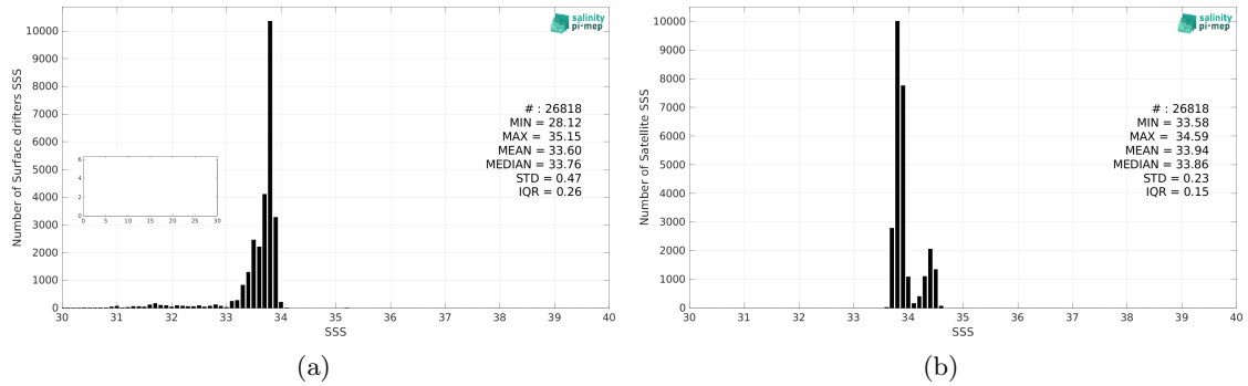
Figure 2: Histograms of SSS from Surface drifters (a) and SMAP SSS L4 OI v2 - 7 Days (ESR) (b) considering all match-up pairs per bins of 0.1 over the Southern Ocean Pi-MEP region and for the full satellite product period.
