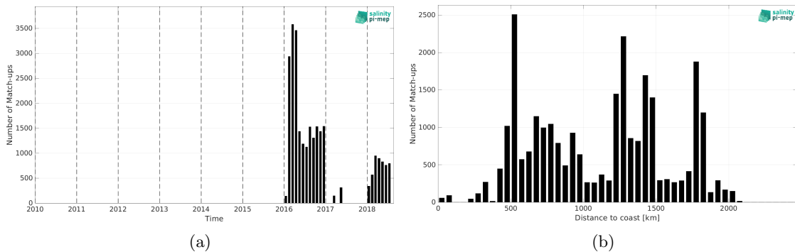
Figure 1: Number of match-ups between Surface drifters and SMAP SSS L4 OI v2 - 7 Days (ESR) SSS as a function of time (a) and as function of the distance to coast (b) over the Southern Ocean Pi-MEP region and for the full satellite product period.
