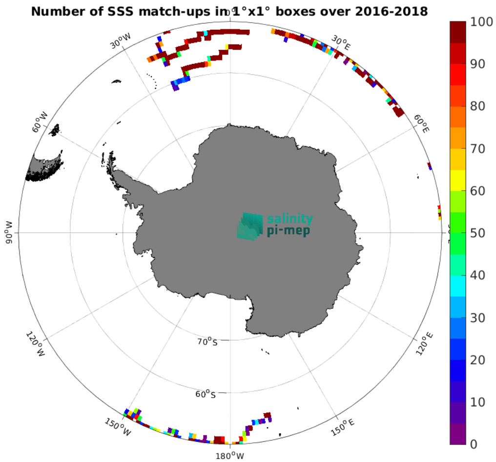
Figure 3: Number of SSS match-ups between Surface drifters SSS and the SMAP SSS L4 OI v2 - 7 Days (ESR) SSS product for the Southern Ocean Pi-MEP region over 1^\circ \times 1^\circ boxes and for the full satellite product period.
