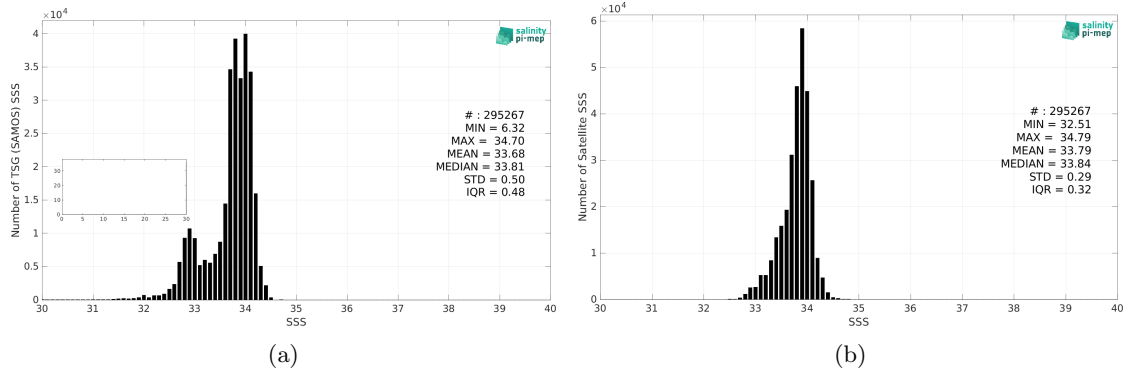
Figure 2: Histograms of SSS from TSG (SAMOS) (a) and SMAP SSS L4 OI v2 - Monthly (IPRC) (b) considering all match-up pairs per bins of 0.1 over the Southern Ocean Pi-MEP region and for the full satellite product period.
