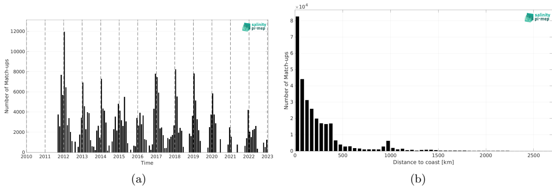
Figure 1: Number of match-ups between TSG (SAMOS) and SMAP SSS L4 OI v2 - Monthly (IPRC) SSS as a function of time (a) and as function of the distance to coast (b) over the Southern Ocean Pi-MEP region and for the full satellite product period.
