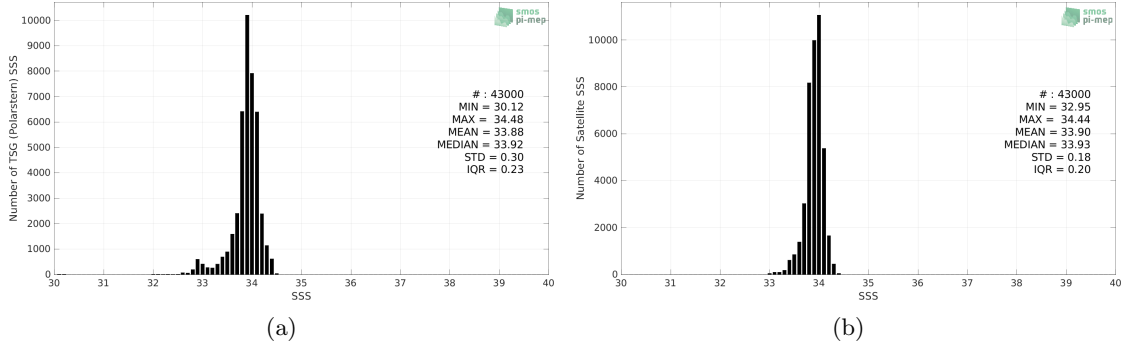
Figure 2: Histograms of SSS from TSG (Polarstern) (a) and SMAP SSS L4 OI v2 - Monthly (IPRC) (b) considering all match-up pairs per bins of 0.1 over the Southern Ocean Pi-MEP region and for the full satellite product period.
