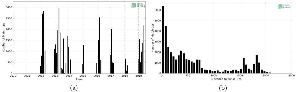
Figure 1: Number of match-ups between TSG (Polarstern) and SMAP SSS L4 OI v2 - Monthly (IPRC) SSS as a function of time (a) and as function of the distance to coast (b) over the Southern Ocean Pi-MEP region and for the full satellite product period.
