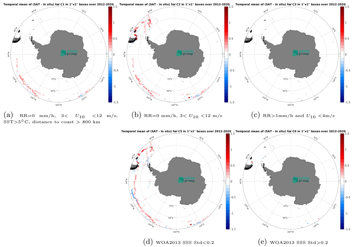
Figure 12: Temporal mean gridded over spatial boxes of size 1^\circ \times 1^\circ of \Delta\text{SSS} (SMAP SSS L4 OI v2 - Monthly (IPRC) - TSG (GOSUD-Sailing-ship)) for 5 different subdatasets corresponding to: RR=0 mm/h, 3 < U_{10} < 12 m/s, SST > 5^\circ\text{C} , distance to coast > 800 km (a), RR=0 mm/h, 3 < U_{10} < 12 m/s (b), RR > 1 mm/h and U_{10} < 4 m/s (c), WOA2013 SSS Std < 0.2 (d), WOA2013 SSS Std > 0.2 (e).
