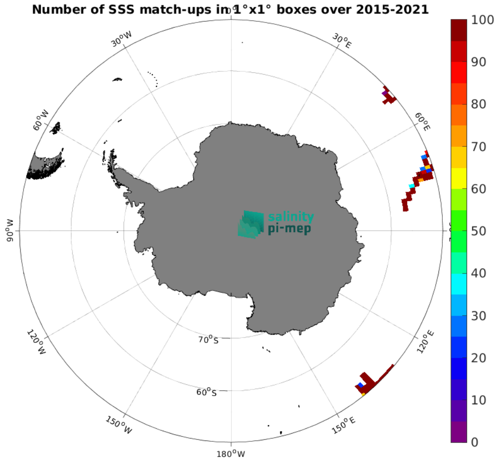
Figure 4: Number of SSS match-ups between TSG (GOSUD-Research-vessel) SSS and the SMAP SSS L4 OI v2 - Monthly (IPRC) SSS product for the Southern Ocean Pi-MEP region over 1^\circ \times 1^\circ boxes and for the full satellite product period.
