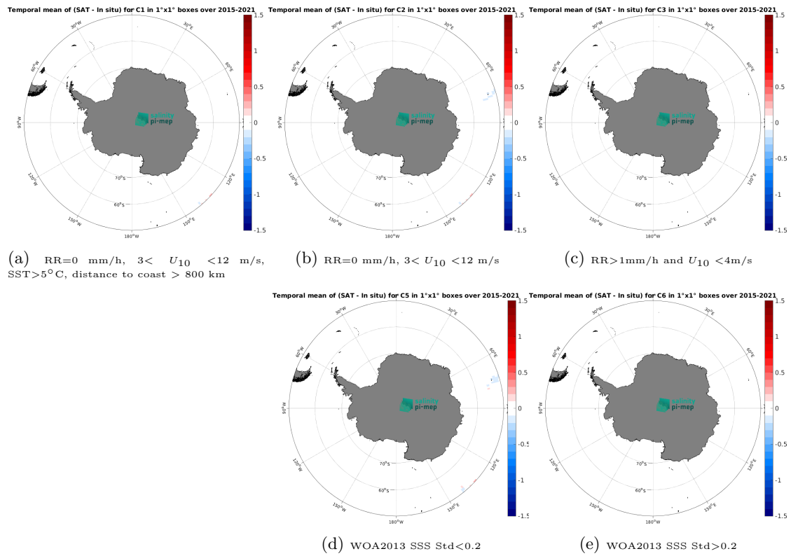
Figure 12: Temporal mean gridded over spatial boxes of size 1^\circ \times 1^\circ of \Delta\text{SSS} (SMAP SSS L4 OI v2 - Monthly (IPRC) - TSG (GOSUD-Research-vessel)) for 5 different subdatasets corresponding to: RR=0 mm/h, 3 < U_{10} < 12 m/s, SST > 5^\circ\text{C} , distance to coast > 800 km (a), RR=0 mm/h, 3 < U_{10} < 12 m/s (b), RR > 1 mm/h and U_{10} < 4 m/s (c), WOA2013 SSS Std < 0.2 (d), WOA2013 SSS Std > 0.2 (e).
