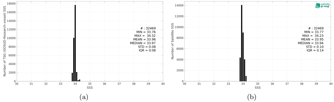
Figure 2: Histograms of SSS from TSG (GOSUD-Research-vessel) (a) and SMAP SSS L4 OI v2 - Monthly (IPRC) (b) considering all match-up pairs per bins of 0.1 over the Southern Ocean Pi-MEP region and for the full satellite product period.
