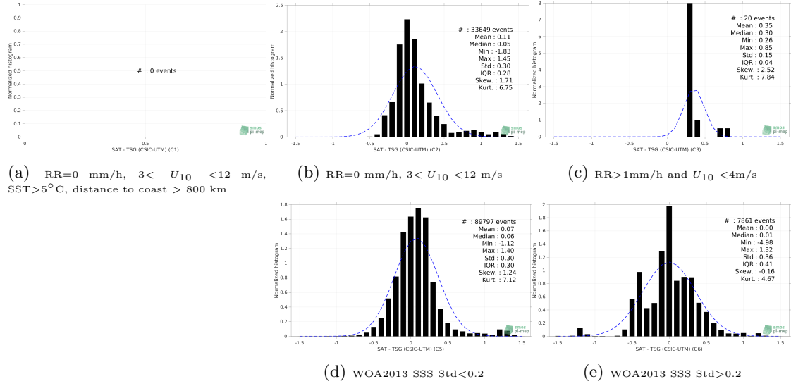
Figure 13: Normalized histogram of \Delta\text{SSS} (SMAP SSS L4 OI v2 - Monthly (IPRC) - TSG (CSIC-UTM)) for 5 different subdatasets corresponding to: RR=0 mm/h, 3 < U_{10} < 12 m/s, SST >5^{\circ}\text{C} , distance to coast > 800 km (a), RR=0 mm/h, 3 < U_{10} < 12 m/s (b), RR>1\text{mm/h} and U_{10} < 4\text{m/s} (c), WOA2013 SSS Std <0.2 (d), WOA2013 SSS Std >0.2 (e).
