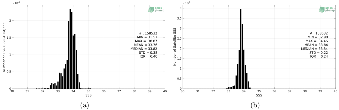
Figure 2: Histograms of SSS from TSG (CSIC-UTM) (a) and SMAP SSS L4 OI v2 - Monthly (IPRC) (b) considering all match-up pairs per bins of 0.1 over the Southern Ocean Pi-MEP region and for the full satellite product period.
