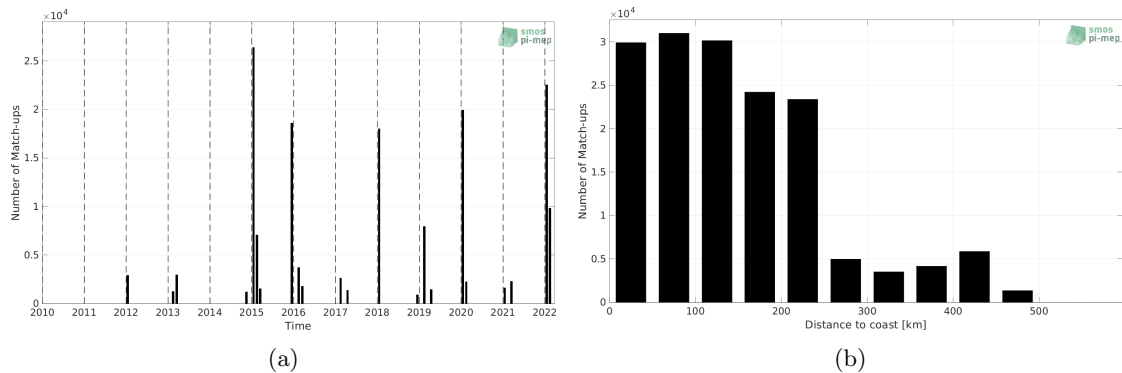
Figure 1: Number of match-ups between TSG (CSIC-UTM) and SMAP SSS L4 OI v2 - Monthly (IPRC) SSS as a function of time (a) and as function of the distance to coast (b) over the Southern Ocean Pi-MEP region and for the full satellite product period.
