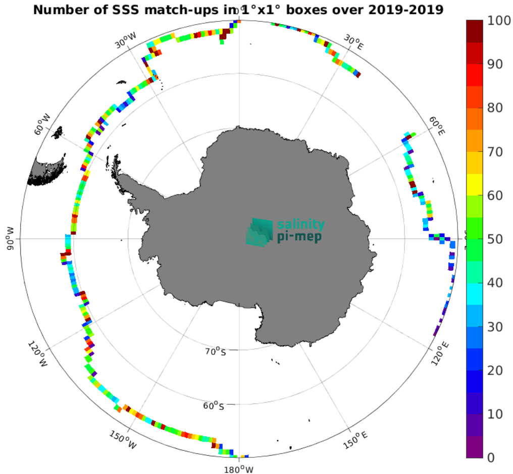
Figure 4: Number of SSS match-ups between Saildrone SSS and the SMAP SSS L4 OI v2 - Monthly (IPRC) SSS product for the Southern Ocean Pi-MEP region over 1^\circ \times 1^\circ boxes and for the full satellite product period.
