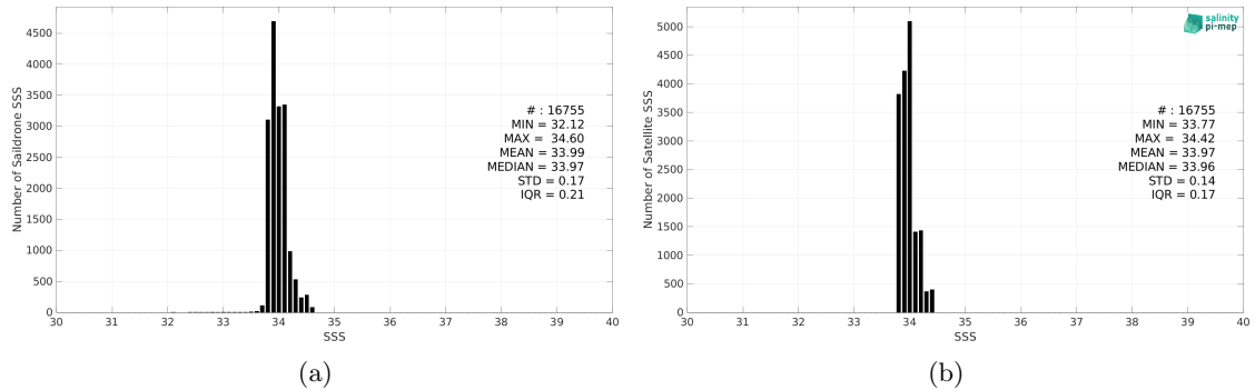
Figure 2: Histograms of SSS from Saildrone (a) and SMAP SSS L4 OI v2 - Monthly (IPRC) (b) considering all match-up pairs per bins of 0.1 over the Southern Ocean Pi-MEP region and for the full satellite product period.
