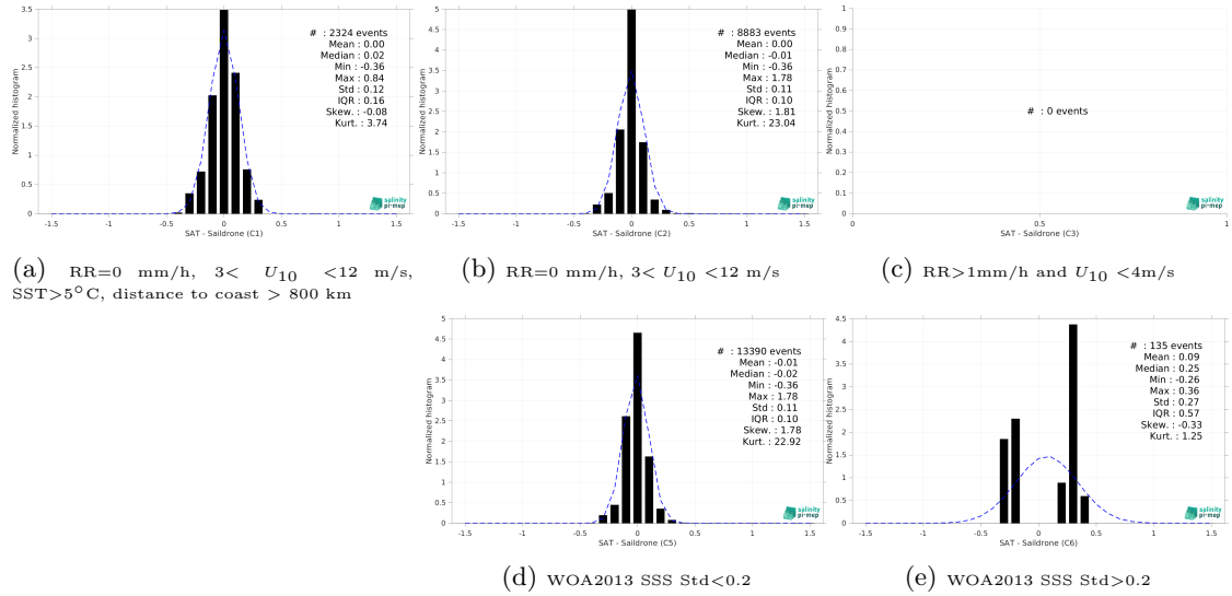
Figure 13: Normalized histogram of \Delta SSS (SMAP SSS L4 OI v2 - Monthly (IPRC) - Saldrone) for 5 different subdatasets corresponding to: RR=0 mm/h, 3 < U_{10} < 12 m/s, SST > 5°C, distance to coast > 800 km (a), RR=0 mm/h, 3 < U_{10} < 12 m/s (b), RR > 1mm/h and U_{10} < 4 m/s (c), WOA2013 SSS Std < 0.2 (d), WOA2013 SSS Std > 0.2 (e).
