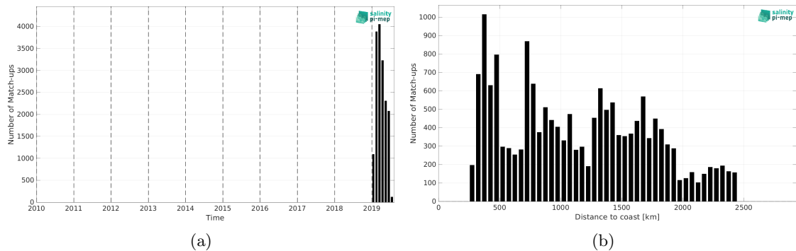
Figure 1: Number of match-ups between Saildrone and SMAP SSS L4 OI v2 - Monthly (IPRC) SSS as a function of time (a) and as function of the distance to coast (b) over the Southern Ocean Pi-MEP region and for the full satellite product period.
