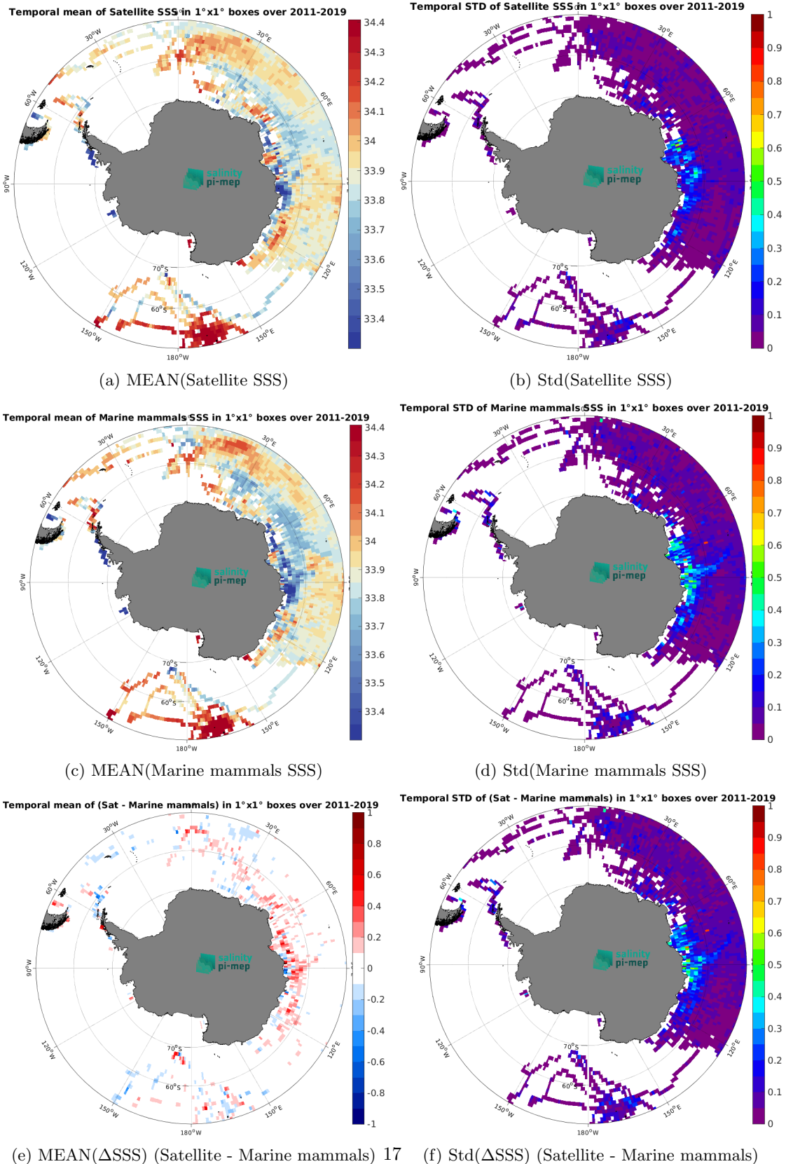
Figure 6: Temporal mean (left) and Std (right) of SSS from SMAP SSS L4 OI v2 - Monthly (IPRC) (top), Marine mammals (middle), and of \Delta SSS (Satellite - Marine mammals). Only match-up pairs are used to generate these maps.
