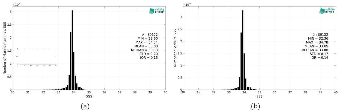
Figure 2: Histograms of SSS from Marine mammals (a) and SMAP SSS L4 OI v2 - Monthly (IPRC) (b) considering all match-up pairs per bins of 0.1 over the Southern Ocean Pi-MEP region and for the full satellite product period.
