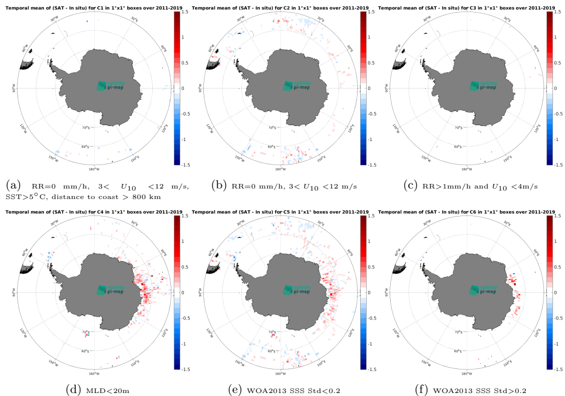
Figure 12: Temporal mean gridded over spatial boxes of size 1^{\circ}\times 1^{\circ} of \Delta\text{SSS} (SMAP SSS L4 OI v2 - Monthly (IPRC) - Marine mammals) for 6 different subdatasets corresponding to:RR=0 mm/h, 3 < U_{10} < 12 m/s, \text{SST} > 5^{\circ}\text{C} , distance to coast > 800 km (a), RR=0 mm/h, 3 < U_{10} < 12 m/s (b), RR > 1\text{mm/h} and U_{10} < 4\text{m/s} (c),MLD < 20\text{m} (d),WOA2013 SSS Std < 0.2 (e),WOA2013 SSS Std > 0.2 (f).
