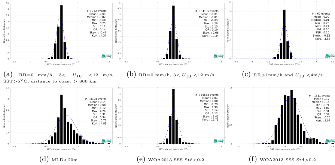
Figure 13: Normalized histogram of \Delta\text{SSS} (SMAP SSS L4 OI v2 - Monthly (IPRC) - Marine mammals) for 6 different subdatasets corresponding to: RR=0 mm/h, 3 < U_{10} < 12 m/s, SST>5°C, distance to coast > 800 km (a), RR=0 mm/h, 3 < U_{10} < 12 m/s (b), RR>1mm/h and U_{10} < 4 m/s (c), MLD<20m (d), WOA2013 SSS Std<0.2 (e), WOA2013 SSS Std>0.2 (f).
