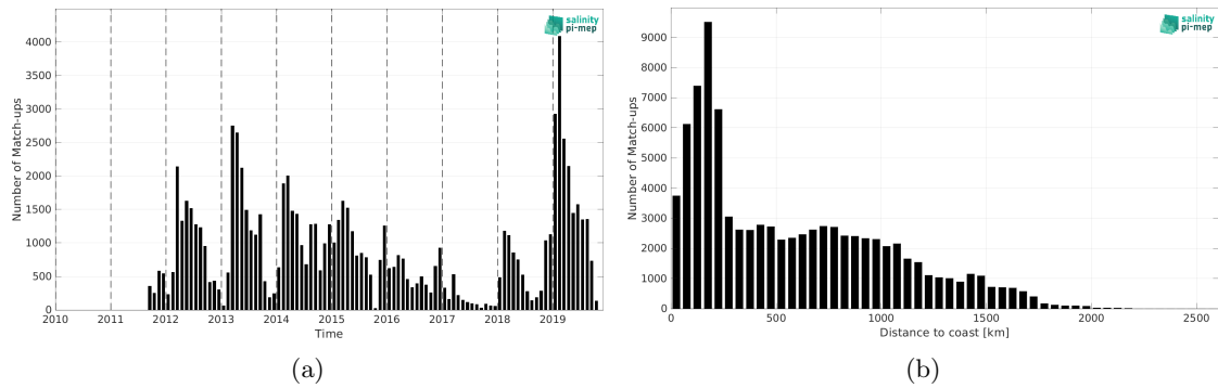
Figure 1: Number of match-ups between Marine mammals and SMAP SSS L4 OI v2 - Monthly (IPRC) SSS as a function of time (a) and as function of the distance to coast (b) over the Southern Ocean Pi-MEP region and for the full satellite product period.
