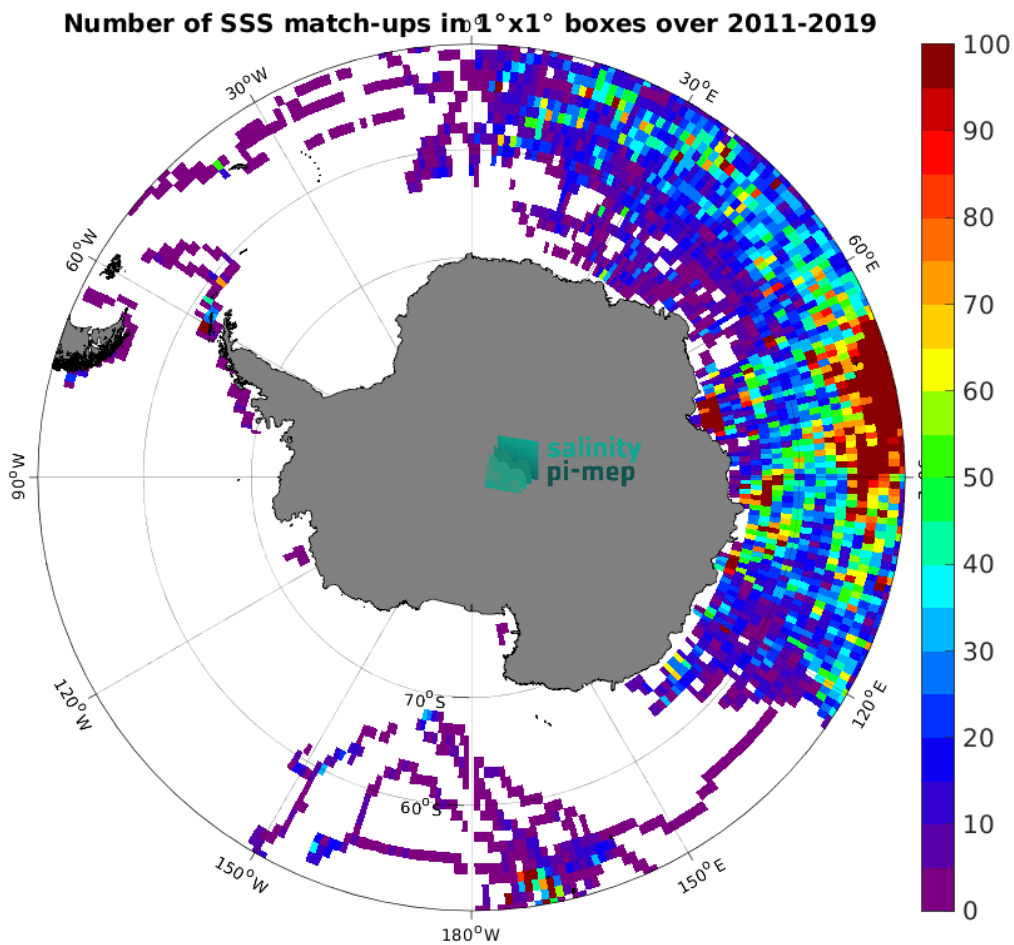
Figure 4: Number of SSS match-ups between Marine mammals SSS and the SMAP SSS L4 OI v2 - Monthly (IPRC) SSS product for the Southern Ocean Pi-MEP region over 1^\circ \times 1^\circ boxes and for the full satellite product period.
