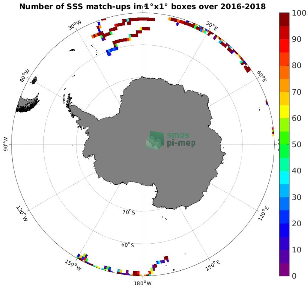
Figure 3: Number of SSS match-ups between Surface drifters SSS and the SMAP SSS L4 OI v2 - Monthly (IPRC) SSS product for the Southern Ocean Pi-MEP region over 1^\circ \times 1^\circ boxes and for the full satellite product period.
