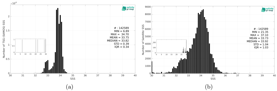
Figure 3: Histograms of SSS from TSG (SAMOS) (a) and SMAP SSS L3 v6 - 8-Day running (RSS) (b) considering all match-up pairs per bins of 0.1 over the Southern Ocean Pi-MEP region and for the full satellite product period.
