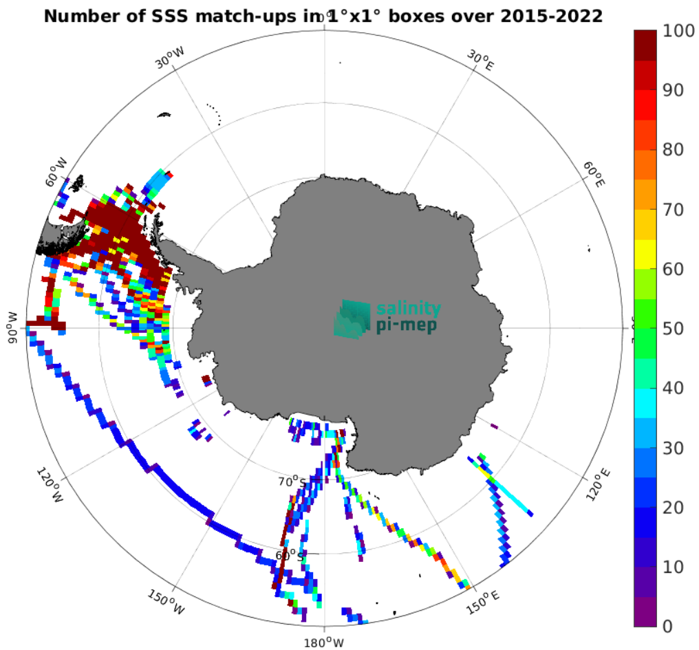
Figure 5: Number of SSS match-ups between TSG (SAMOS) SSS and the SMAP SSS L3 v6 - 8-Day running (RSS) SSS product for the Southern Ocean Pi-MEP region over 1^\circ \times 1^\circ boxes and for the full satellite product period.
