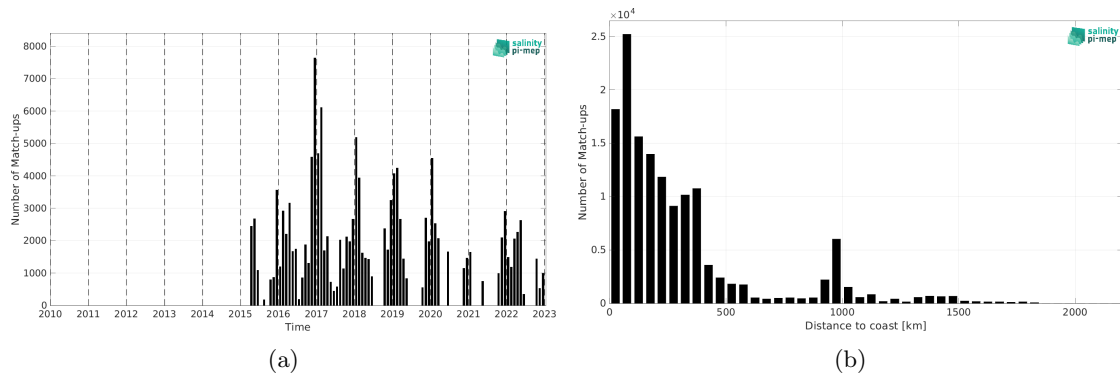
Figure 2: Number of match-ups between TSG (SAMOS) and SMAP SSS L3 v6 - 8-Day running (RSS) SSS as a function of time (a) and as function of the distance to coast (b) over the Southern Ocean Pi-MEP region and for the full satellite product period.
