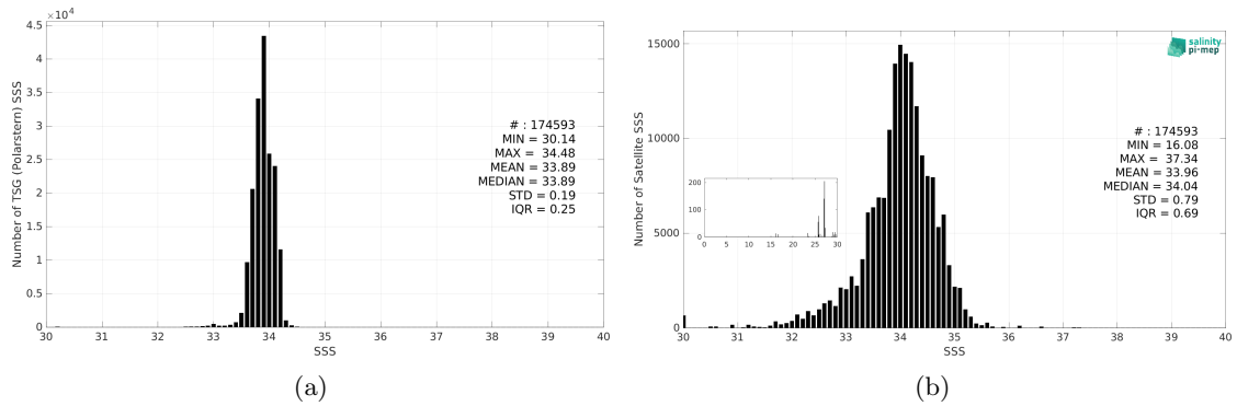
Figure 3: Histograms of SSS from TSG (Polarstern) (a) and SMAP SSS L3 v6 - 8-Day running (RSS) (b) considering all match-up pairs per bins of 0.1 over the Southern Ocean Pi-MEP region and for the full satellite product period.
