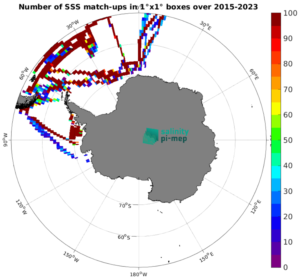
Figure 5: Number of SSS match-ups between TSG (Polarstern) SSS and the SMAP SSS L3 v6 - 8-Day running (RSS) SSS product for the Southern Ocean Pi-MEP region over 1^\circ \times 1^\circ boxes and for the full satellite product period.
