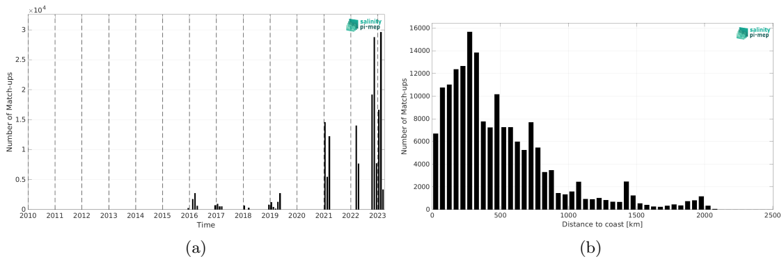
Figure 2: Number of match-ups between TSG (Polarstern) and SMAP SSS L3 v6 - 8-Day running (RSS) SSS as a function of time (a) and as function of the distance to coast (b) over the Southern Ocean Pi-MEP region and for the full satellite product period.
