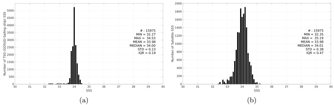
Figure 3: Histograms of SSS from TSG (GOSUD-Sailing-ship) (a) and SMAP SSS L3 v6 - 8-Day running (RSS) (b) considering all match-up pairs per bins of 0.1 over the Southern Ocean Pi-MEP region and for the full satellite product period.
