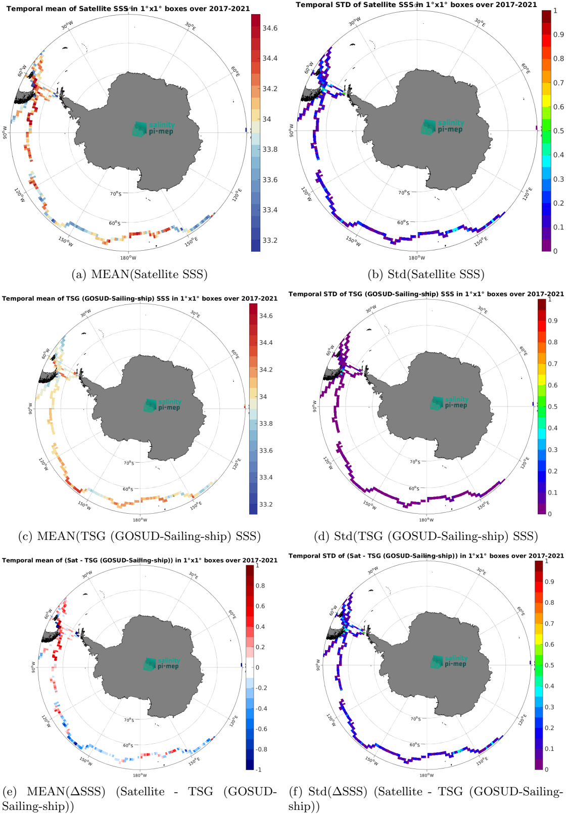
Figure 7: Temporal mean (left) and Std (right) of SSS from SMAP SSS L3 v6 - 8-Day running (RSS) (top), TSG (GOSUD-Sailing-ship) (middle), and of \Delta SSS (Satellite - TSG (GOSUD-Sailing-ship)). Only match-up pairs are used to generate these maps.
