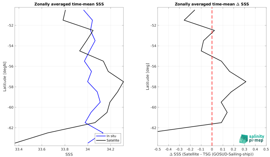
Figure 9: Left panel: Zonal mean SSS from SMAP SSS L3 v6 - 8-Day running (RSS) satellite product (black) and from TSG (GOSUD-Sailing-ship) (blue). Right panel: Zonal mean of \Delta SSS (Satellite - TSG (GOSUD-Sailing-ship)) for all the collected Pi-MEP match-up pairs estimated over the full satellite product period.
