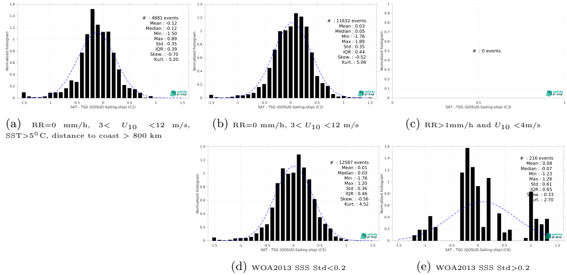
Figure 15: Normalized histogram of \Delta SSS (SMAP SSS L3 v6 - 8-Day running (RSS) - TSG (GOSUD-Sailing-ship)) for 5 different subdatasets corresponding to: RR=0 mm/h, 3 < U_{10} < 12 m/s, SST > 5°C, distance to coast > 800 km (a), RR=0 mm/h, 3 < U_{10} < 12 m/s (b), RR > 1mm/h and U_{10} < 4 m/s (c), WOA2013 SSS Std < 0.2 (d), WOA2013 SSS Std > 0.2 (e).
