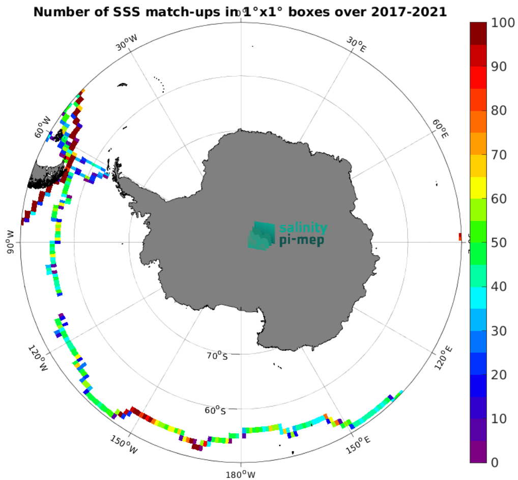
Figure 5: Number of SSS match-ups between TSG (GOSUD-Sailing-ship) SSS and the SMAP SSS L3 v6 - 8-Day running (RSS) SSS product for the Southern Ocean Pi-MEP region over 1^\circ \times 1^\circ boxes and for the full satellite product period.
