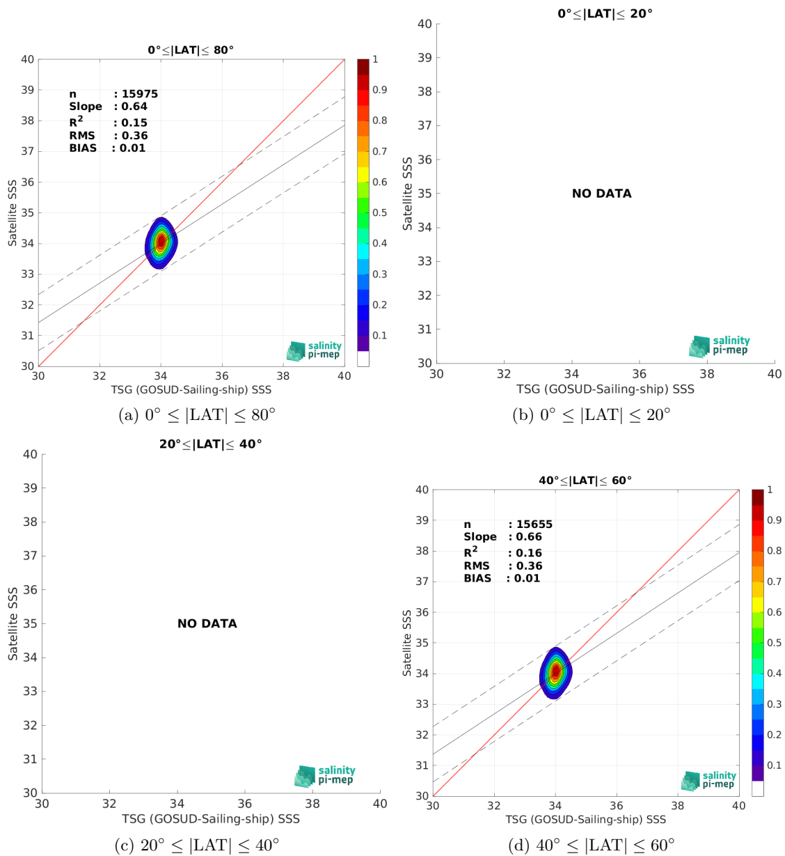
Figure 10: Contour maps of the concentration of SMAP SSS L3 v6 - 8-Day running (RSS) SSS (y-axis) versus TSG (GOSUD-Sailing-ship) SSS (x-axis) at match-up pairs for different latitude bands. For each plot, the red line shows x=y . The black thin and dashed lines indicate a linear fit through the data cloud and the \pm 95\% confidence levels, respectively. The number match-up pairs n , the slope and R^2 coefficient of the linear fit, the root mean square (RMS) and the mean bias between satellite and in situ data are indicated for each latitude band in each plots.
