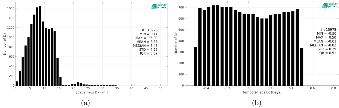
Figure 6: Histograms of the spatial (a) and temporal (b) lags between the location/time of the TSG (GOSUD-Sailing-ship) measurement and the date of the corresponding SMAP SSS L3 v6 - 8-Day running (RSS) SSS pixel.
