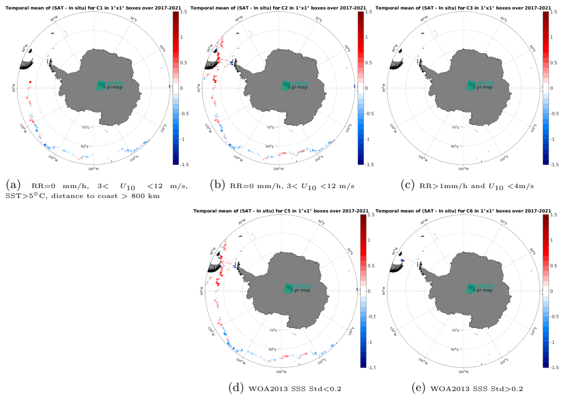
Figure 14: Temporal mean gridded over spatial boxes of size 1^\circ \times 1^\circ of \Delta SSS (SMAP SSS L3 v6 - 8-Day running (RSS) - TSG (GOSUD-Sailing-ship)) for 5 different subdatasets corresponding to:RR=0 mm/h, 3 < U_{10} < 12 m/s, SST > 5^\circ\text{C} , distance to coast > 800 km (a), RR=0 mm/h, 3 < U_{10} < 12 m/s (b), RR > 1 mm/h and U_{10} < 4 m/s (c), WOA2013 SSS Std < 0.2 (d), WOA2013 SSS Std > 0.2 (e).
