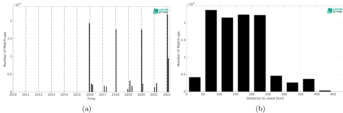
Figure 2: Number of match-ups between TSG (CSIC-UTM) and SMAP SSS L3 v6 - 8-Day running (RSS) SSS as a function of time (a) and as function of the distance to coast (b) over the Southern Ocean Pi-MEP region and for the full satellite product period.
