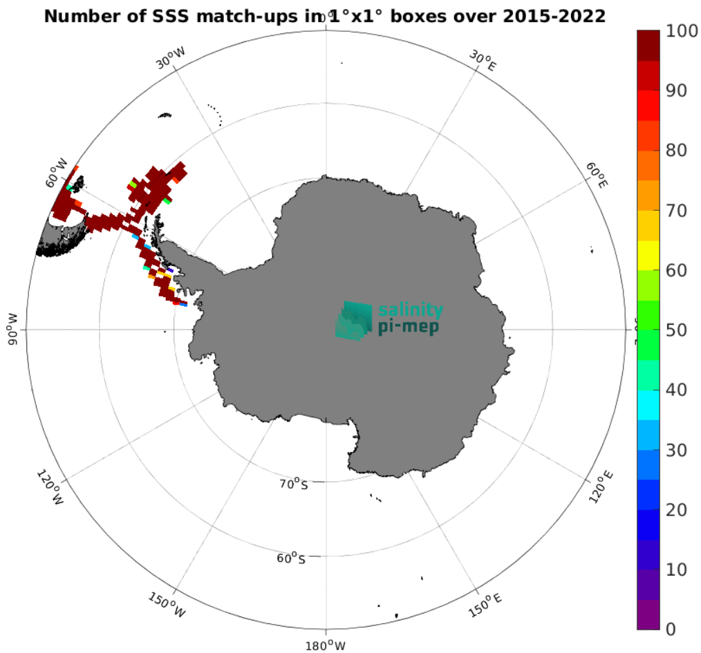
Figure 5: Number of SSS match-ups between TSG (CSIC-UTM) SSS and the SMAP SSS L3 v6 - 8-Day running (RSS) SSS product for the Southern Ocean Pi-MEP region over 1^{\circ} \times 1^{\circ} boxes and for the full satellite product period.
