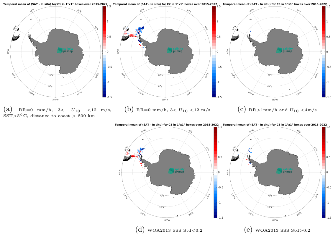
Figure 14: Temporal mean gridded over spatial boxes of size 1^\circ \times 1^\circ of \Delta\text{SSS} (SMAP SSS L3 v6 - 8-Day running (RSS) - TSG (CSIC-UTM)) for 5 different subdatasets corresponding to:RR=0 mm/h, 3 < U_{10} < 12 m/s, SST > 5°C, distance to coast > 800 km (a), RR=0 mm/h, 3 < U_{10} < 12 m/s (b), RR > 1mm/h and U_{10} < 4 m/s (c), WOA2013 SSS Std < 0.2 (d), WOA2013 SSS Std > 0.2 (e).
