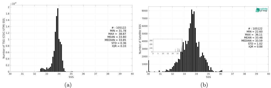
Figure 3: Histograms of SSS from TSG (CSIC-UTM) (a) and SMAP SSS L3 v6 - 8-Day running (RSS) (b) considering all match-up pairs per bins of 0.1 over the Southern Ocean Pi-MEP region and for the full satellite product period.
