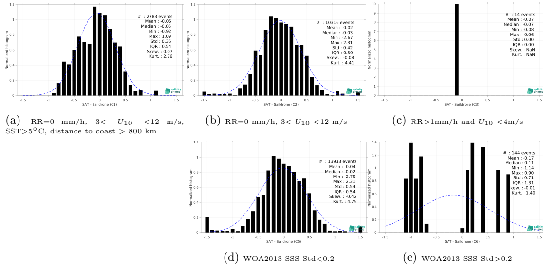
Figure 15: Normalized histogram of \Delta SSS (SMAP SSS L3 v6 - 8-Day running (RSS) - Saildrone) for 5 different subdatasets corresponding to: RR=0 mm/h, 3 < U_{10} < 12 m/s, SST > 5°C, distance to coast > 800 km (a), RR=0 mm/h, 3 < U_{10} < 12 m/s (b), RR > 1mm/h and U_{10} < 4 m/s (c), WOA2013 SSS Std < 0.2 (d), WOA2013 SSS Std > 0.2 (e).
