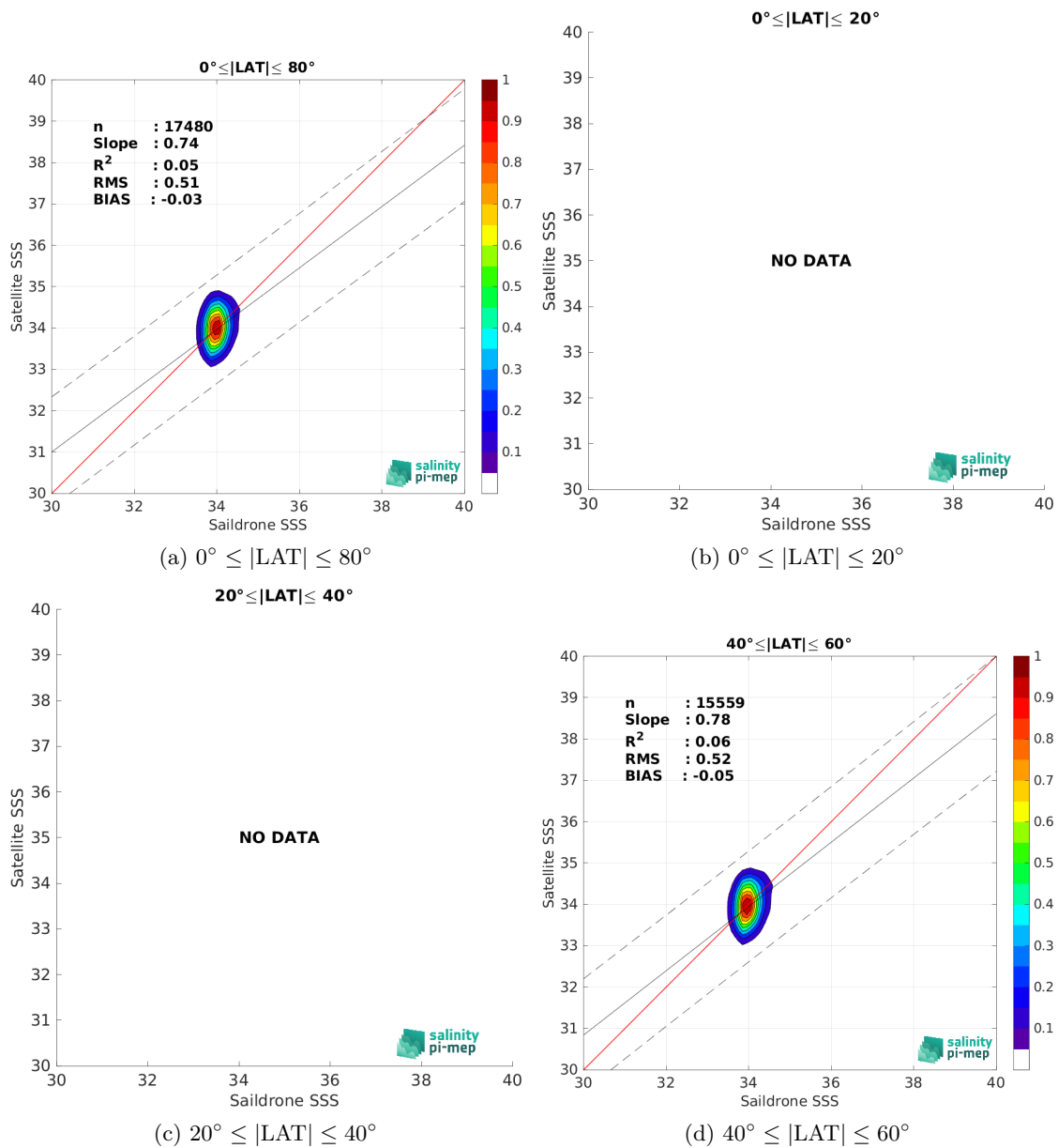
Figure 10: Contour maps of the concentration of SMAP SSS L3 v6 - 8-Day running (RSS) SSS (y-axis) versus Saildrone SSS (x-axis) at match-up pairs for different latitude bands. For each plot, the red line shows x=y . The black thin and dashed lines indicate a linear fit through the data cloud and the \pm 95\% confidence levels, respectively. The number match-up pairs n , the slope and R^2 coefficient of the linear fit, the root mean square (RMS) and the mean bias between satellite and in situ data are indicated for each latitude band in each plots.
