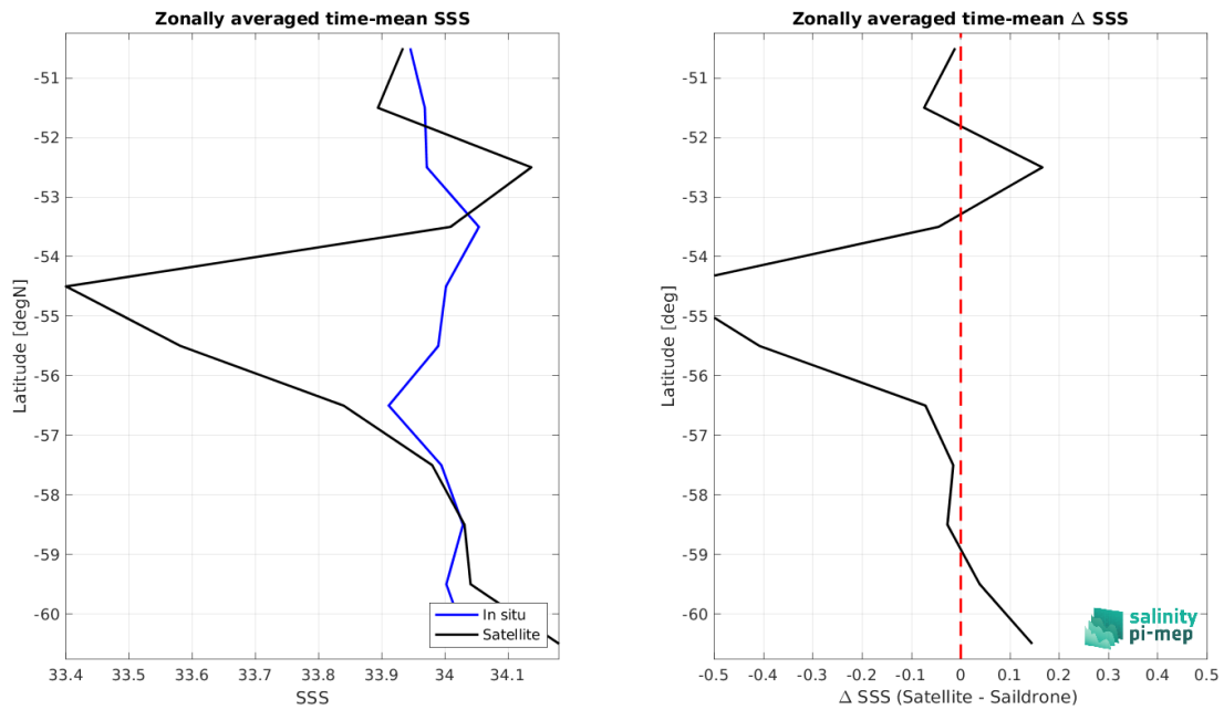
Figure 9: Left panel: Zonal mean SSS from SMAP SSS L3 v6 - 8-Day running (RSS) satellite product (black) and from Sairdron (blue). Right panel: Zonal mean of \Delta SSS (Satellite - Sairdron) for all the collected Pi-MEP match-up pairs estimated over the full satellite product period.
