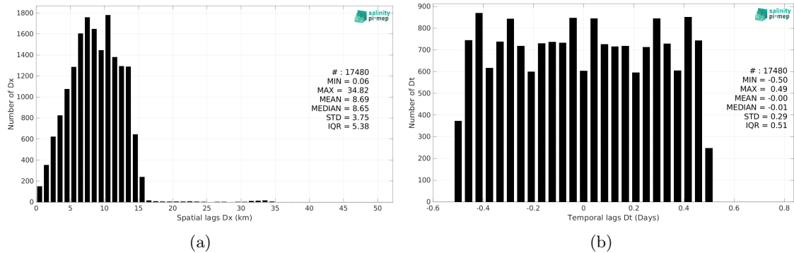
Figure 6: Histograms of the spatial (a) and temporal (b) lags between the location/time of the Sairdrone measurement and the date of the corresponding SMAP SSS L3 v6 - 8-Day running (RSS) SSS pixel.
