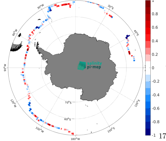
(e) MEAN( \Delta SSS) (Satellite - Saildrone)
