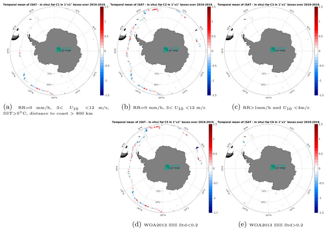
Figure 14: Temporal mean gridded over spatial boxes of size 1^\circ \times 1^\circ of \Delta SSS (SMAP SSS L3 v6 - 8-Day running (RSS) - Saicdrone) for 5 different subdatasets corresponding to:RR=0 mm/h, 3 < U_{10} < 12 m/s, SST >5^\circ C, distance to coast > 800 km (a), RR=0 mm/h, 3 < U_{10} < 12 m/s (b), RR >1 mm/h and U_{10} < 4 m/s (c), WOA2013 SSS Std <0.2 (d), WOA2013 SSS Std >0.2 (e).
