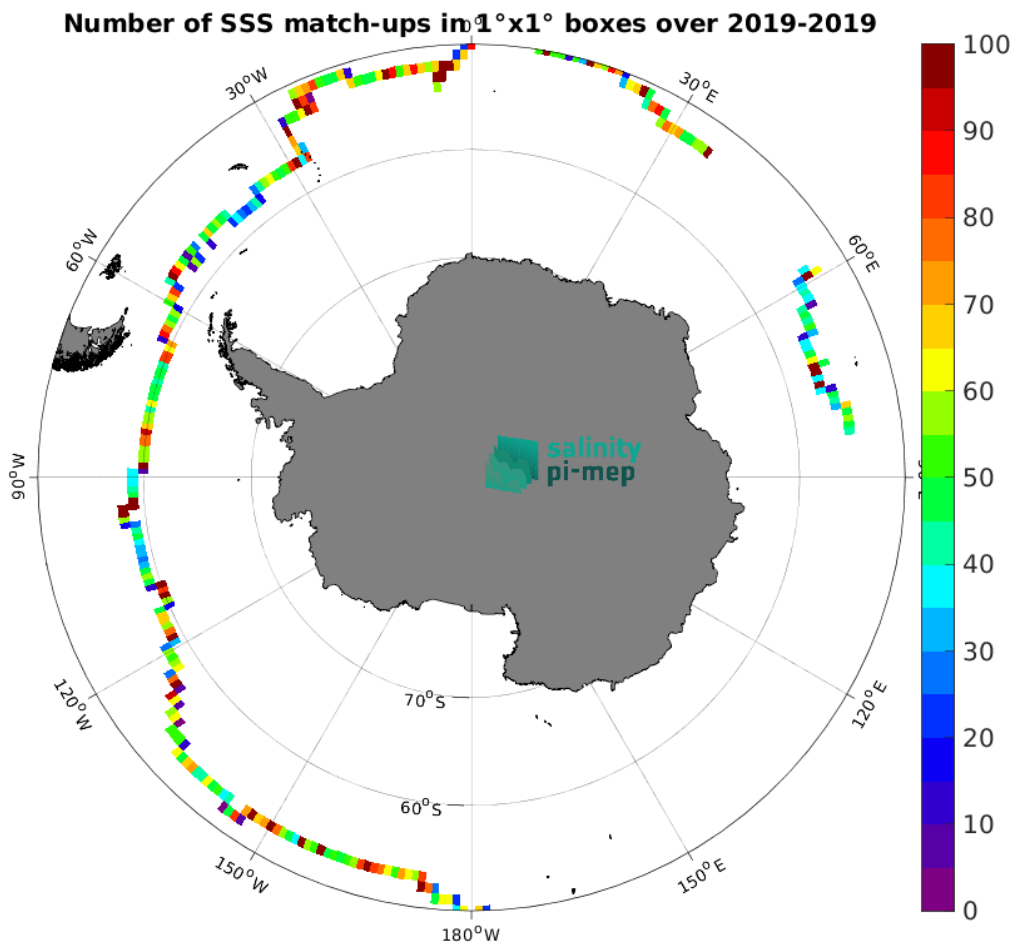
Figure 5: Number of SSS match-ups between Saildrone SSS and the SMAP SSS L3 v6 - 8-Day running (RSS) SSS product for the Southern Ocean Pi-MEP region over 1^{\circ} \times 1^{\circ} boxes and for the full satellite product period.
