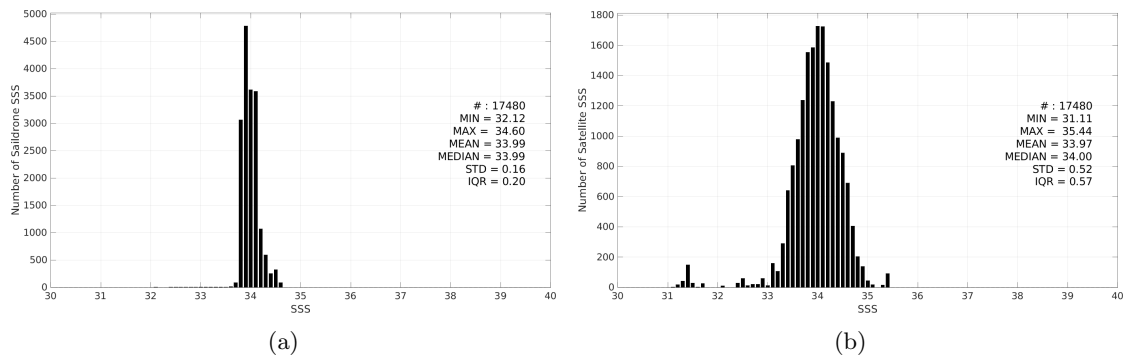
Figure 3: Histograms of SSS from Saildrone (a) and SMAP SSS L3 v6 - 8-Day running (RSS) (b) considering all match-up pairs per bins of 0.1 over the Southern Ocean Pi-MEP region and for the full satellite product period.
