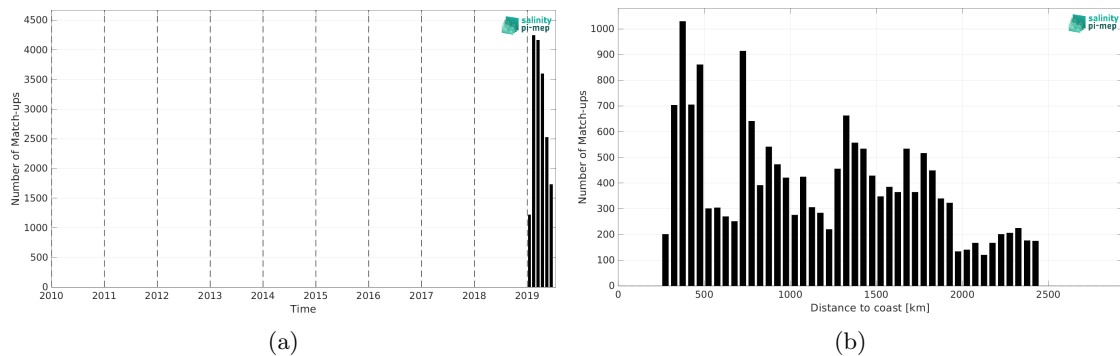
Figure 2: Number of match-ups between Saildrone and SMAP SSS L3 v6 - 8-Day running (RSS) SSS as a function of time (a) and as function of the distance to coast (b) over the Southern Ocean Pi-MEP region and for the full satellite product period.
