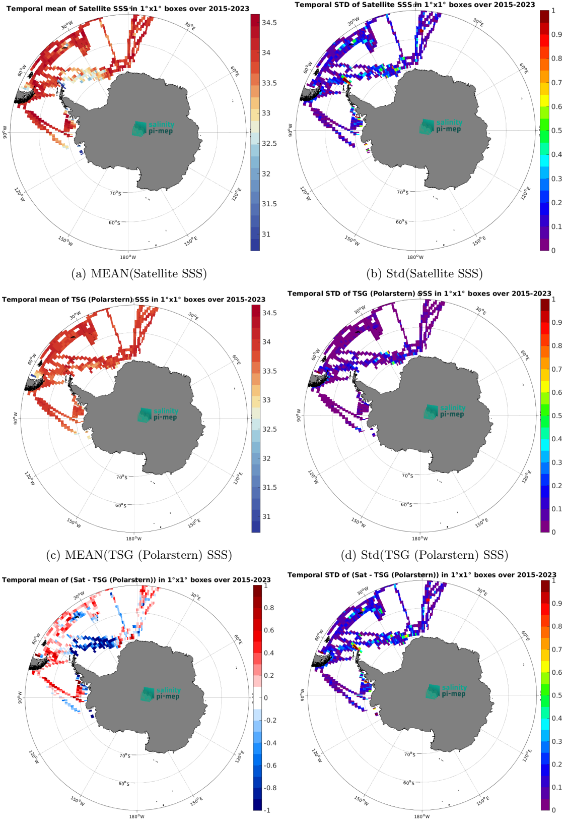
Figure 7: Temporal mean (left) and Std (right) of SSS from SMAP SSS L3 v6 - Monthly (RSS) (top), TSG (Polarstern) (middle), and of \Delta SSS (Satellite - TSG (Polarstern)). Only match-up pairs are used to generate these maps.
