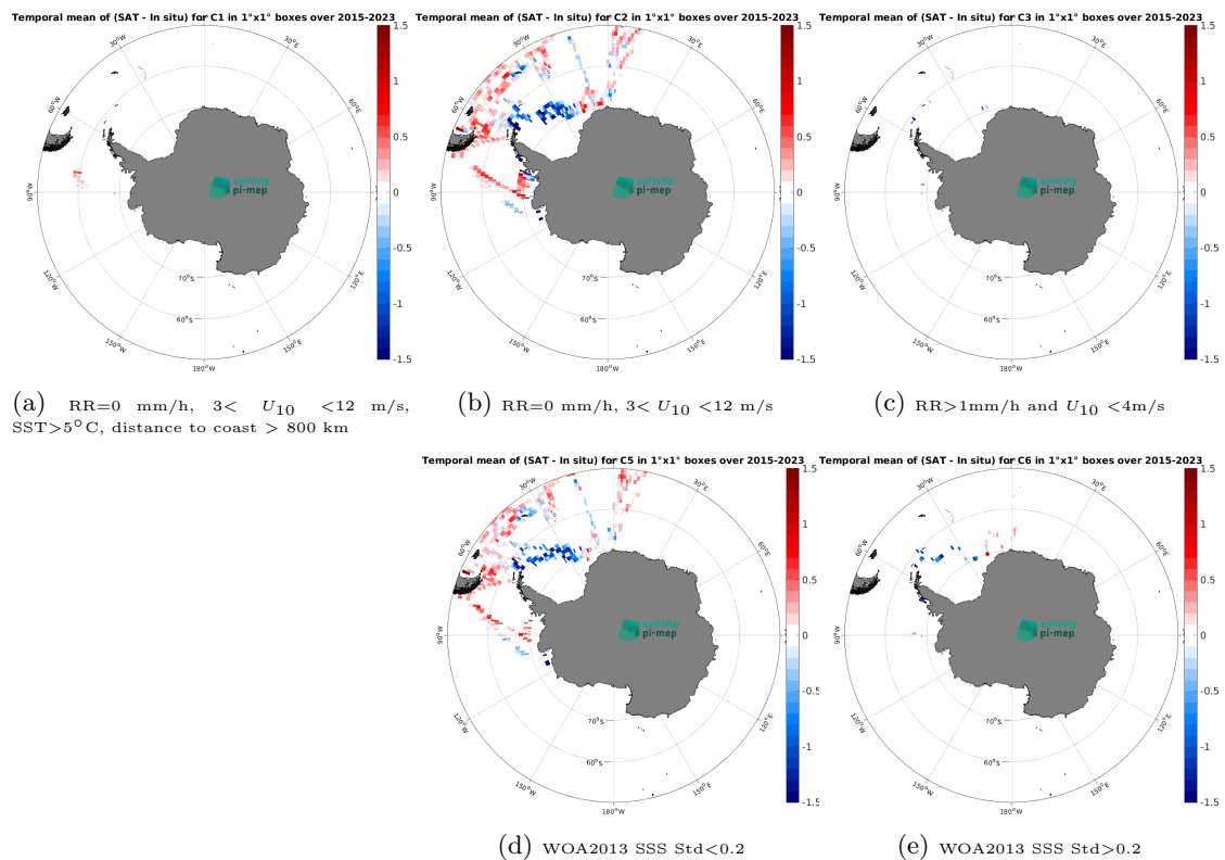
Figure 14: Temporal mean gridded over spatial boxes of size 1^\circ \times 1^\circ of \Delta\text{SSS} (SMAP SSS L3 v6 - Monthly (RSS) - TSG (Polarstern)) for 5 different subdatasets corresponding to:RR=0 mm/h, 3 < U_{10} < 12 m/s, SST>5°C, distance to coast > 800 km (a), RR=0 mm/h, 3 < U_{10} < 12 m/s (b), RR>1mm/h and U_{10} < 4 m/s (c), WOA2013 SSS Std<0.2 (d), WOA2013 SSS Std>0.2 (e).
