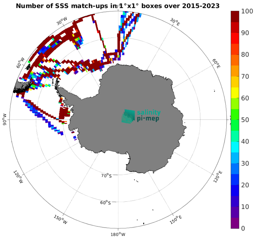
Figure 5: Number of SSS match-ups between TSG (Polarstern) SSS and the SMAP SSS L3 v6 - Monthly (RSS) SSS product for the Southern Ocean Pi-MEP region over 1^\circ \times 1^\circ boxes and for the full satellite product period.
