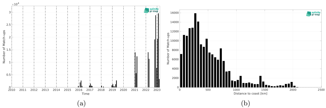
Figure 2: Number of match-ups between TSG (Polarstern) and SMAP SSS L3 v6 - Monthly (RSS) SSS as a function of time (a) and as function of the distance to coast (b) over the Southern Ocean Pi-MEP region and for the full satellite product period.
