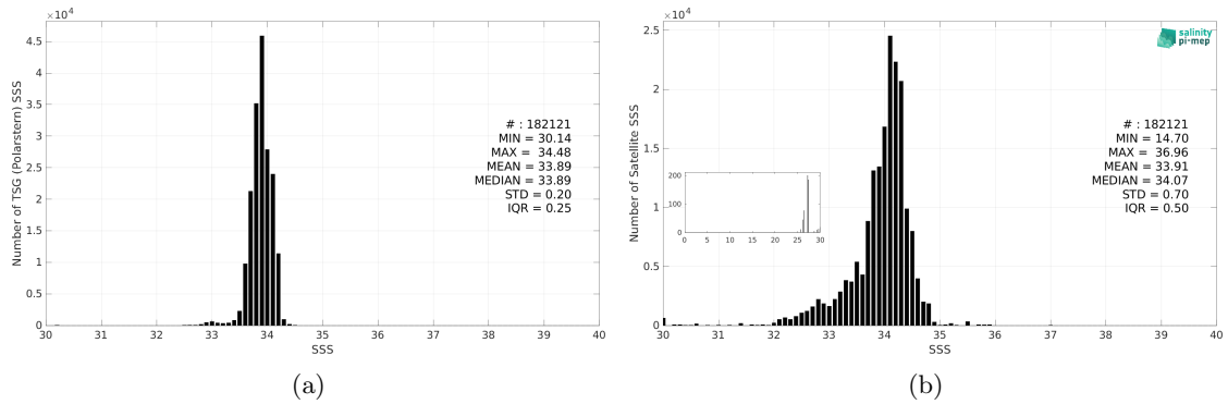
Figure 3: Histograms of SSS from TSG (Polarstern) (a) and SMAP SSS L3 v6 - Monthly (RSS) (b) considering all match-up pairs per bins of 0.1 over the Southern Ocean Pi-MEP region and for the full satellite product period.
