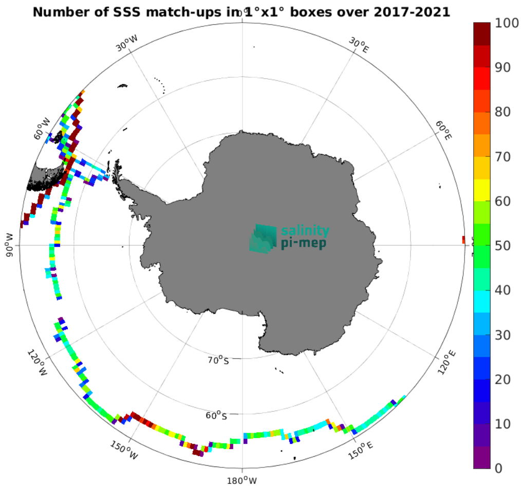
Figure 5: Number of SSS match-ups between TSG (GOSUD-Sailing-ship) SSS and the SMAP SSS L3 v6 - Monthly (RSS) SSS product for the Southern Ocean Pi-MEP region over 1^{\circ} \times 1^{\circ} boxes and for the full satellite product period.
