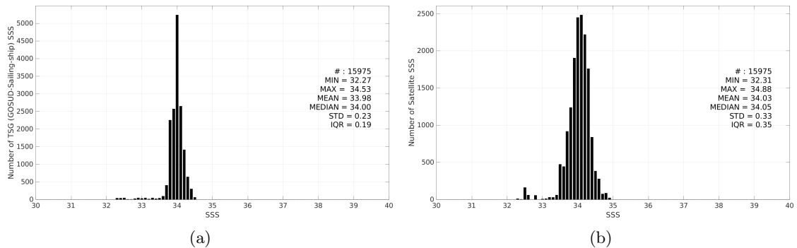
Figure 3: Histograms of SSS from TSG (GOSUD-Sailing-ship) (a) and SMAP SSS L3 v6 - Monthly (RSS) (b) considering all match-up pairs per bins of 0.1 over the Southern Ocean Pi-MEP region and for the full satellite product period.
