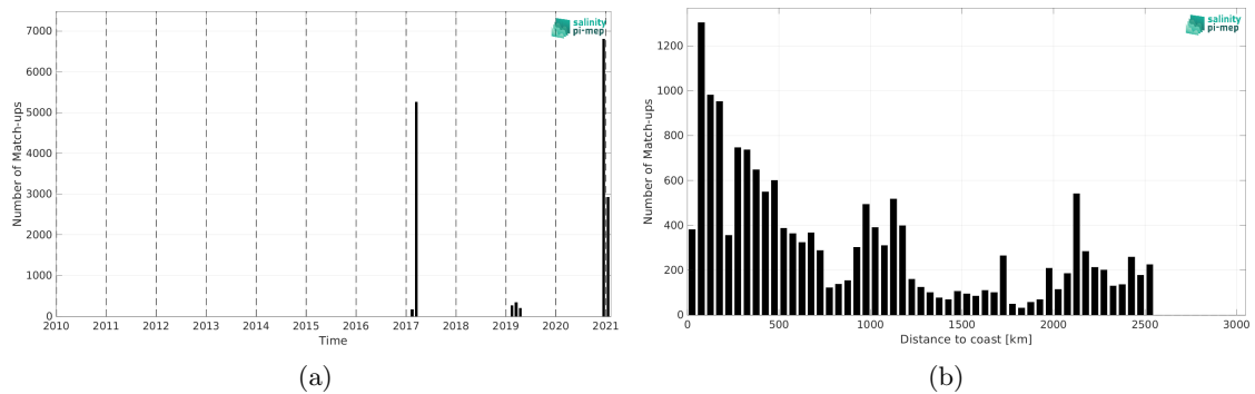
Figure 2: Number of match-ups between TSG (GOSUD-Sailing-ship) and SMAP SSS L3 v6 - Monthly (RSS) SSS as a function of time (a) and as function of the distance to coast (b) over the Southern Ocean Pi-MEP region and for the full satellite product period.
