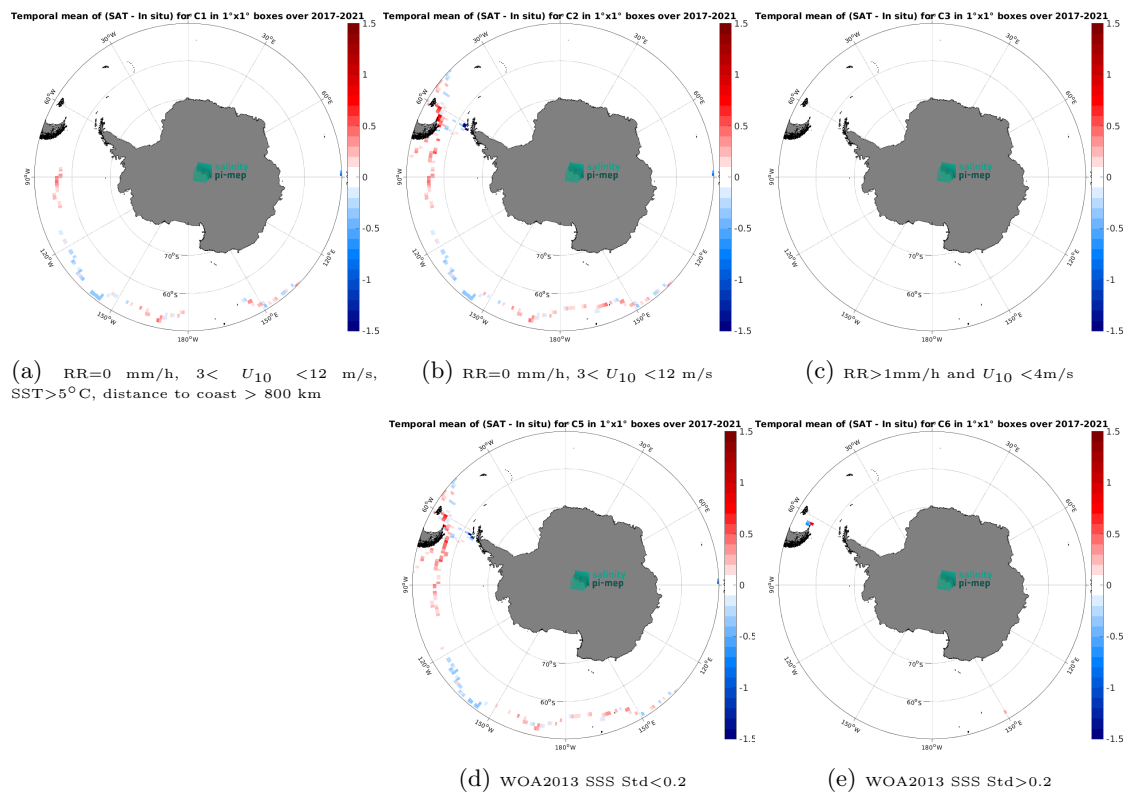
Figure 14: Temporal mean gridded over spatial boxes of size 1^\circ \times 1^\circ of \Delta\text{SSS} (SMAP SSS L3 v6 - Monthly (RSS) - TSG (GOSUD-Sailing-ship)) for 5 different subdatasets corresponding to:RR=0 mm/h, 3 < U_{10} < 12 m/s, SST >5^\circ\text{C} , distance to coast > 800 km (a), RR=0 mm/h, 3 < U_{10} < 12 m/s (b), RR >1 mm/h and U_{10} < 4 m/s (c), WOA2013 SSS Std <0.2 (d), WOA2013 SSS Std >0.2 (e).
