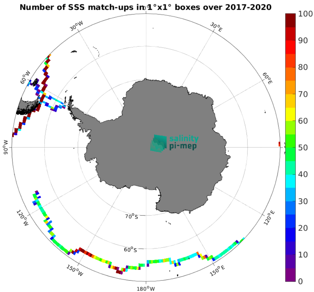
Figure 5: Number of SSS match-ups between TSG (GOSUD-Sailing-ship) SSS and the SMAP SSS L3 v6 - Monthly (RSS) SSS product for the Southern Ocean Pi-MEP region over 1^\circ \times 1^\circ boxes and for the full satellite product period.
