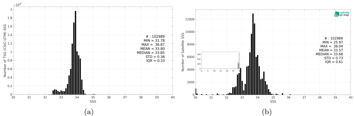
Figure 3: Histograms of SSS from TSG (CSIC-UTM) (a) and SMAP SSS L3 v6 - Monthly (RSS) (b) considering all match-up pairs per bins of 0.1 over the Southern Ocean Pi-MEP region and for the full satellite product period.
