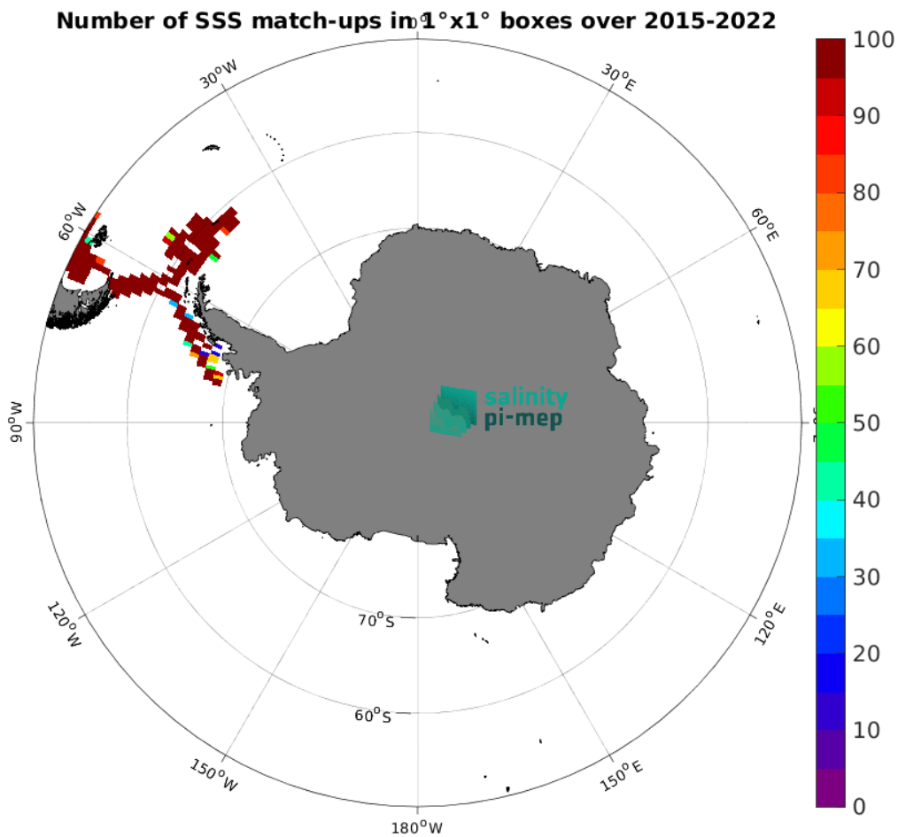
Figure 5: Number of SSS match-ups between TSG (CSIC-UTM) SSS and the SMAP SSS L3 v6 - Monthly (RSS) SSS product for the Southern Ocean Pi-MEP region over 1^\circ \times 1^\circ boxes and for the full satellite product period.
