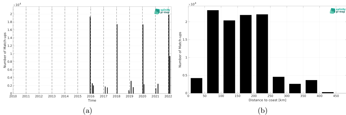
Figure 2: Number of match-ups between TSG (CSIC-UTM) and SMAP SSS L3 v6 - Monthly (RSS) SSS as a function of time (a) and as function of the distance to coast (b) over the Southern Ocean Pi-MEP region and for the full satellite product period.
