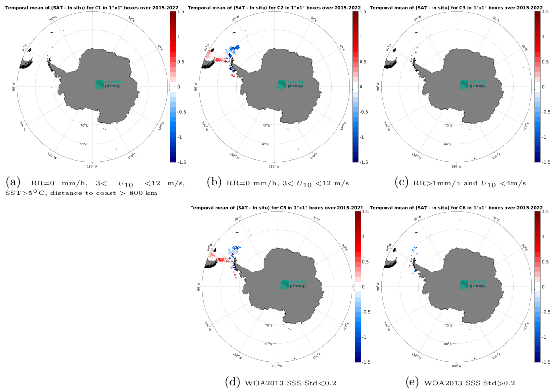
Figure 14: Temporal mean gridded over spatial boxes of size 1^\circ \times 1^\circ of \Delta\text{SSS} (SMAP SSS L3 v6 - Monthly (RSS) - TSG (CSIC-UTM)) for 5 different subdatasets corresponding to:RR=0 mm/h, 3 < U_{10} < 12 m/s, SST>5°C, distance to coast > 800 km (a), RR=0 mm/h, 3 < U_{10} < 12 m/s (b), RR>1mm/h and U_{10} < 4 m/s (c), WOA2013 SSS Std<0.2 (d), WOA2013 SSS Std>0.2 (e).
