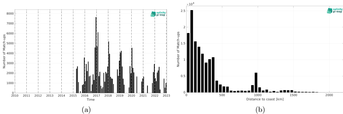
Figure 2: Number of match-ups between TSG (SAMOS) and SMAP SSS L3 v5.3 - 8-Day running (RSS) SSS as a function of time (a) and as function of the distance to coast (b) over the Southern Ocean Pi-MEP region and for the full satellite product period.
