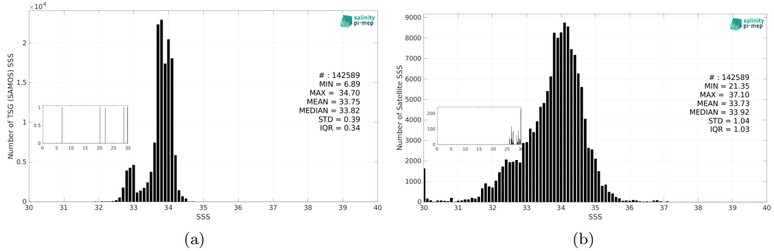
Figure 3: Histograms of SSS from TSG (SAMOS) (a) and SMAP SSS L3 v5.3 - 8-Day running (RSS) (b) considering all match-up pairs per bins of 0.1 over the Southern Ocean Pi-MEP region and for the full satellite product period.
