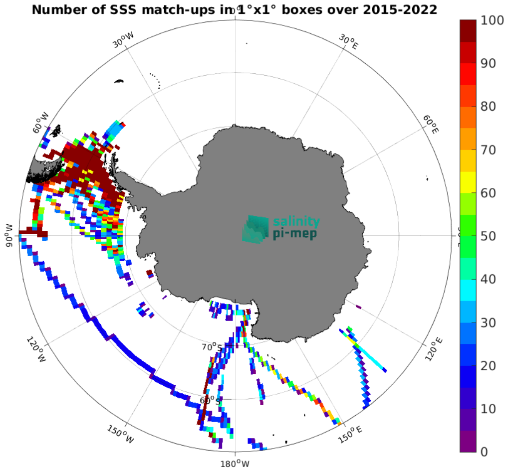
Figure 5: Number of SSS match-ups between TSG (SAMOS) SSS and the SMAP SSS L3 v5.3 - 8-Day running (RSS) SSS product for the Southern Ocean Pi-MEP region over 1^\circ \times 1^\circ boxes and for the full satellite product period.
