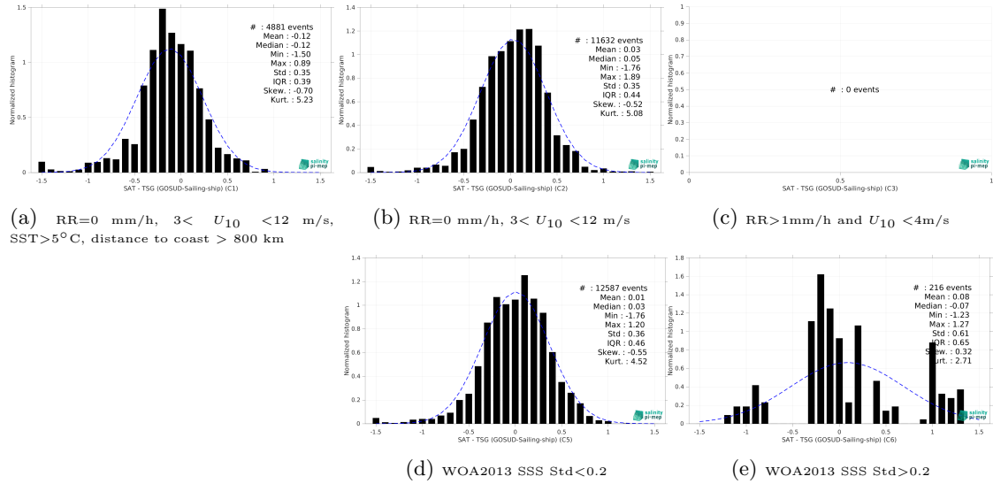
Figure 15: Normalized histogram of \Delta SSS (SMAP SSS L3 v5.3 - 8-Day running (RSS) - TSG (GOSUD-Sailing-ship)) for 5 different subdatasets corresponding to: RR=0 mm/h, 3 < U_{10} < 12 m/s, SST > 5°C, distance to coast > 800 km (a), RR=0 mm/h, 3 < U_{10} < 12 m/s (b), RR > 1mm/h and U_{10} < 4 m/s (c), WOA2013 SSS Std < 0.2 (d), WOA2013 SSS Std > 0.2 (e).
