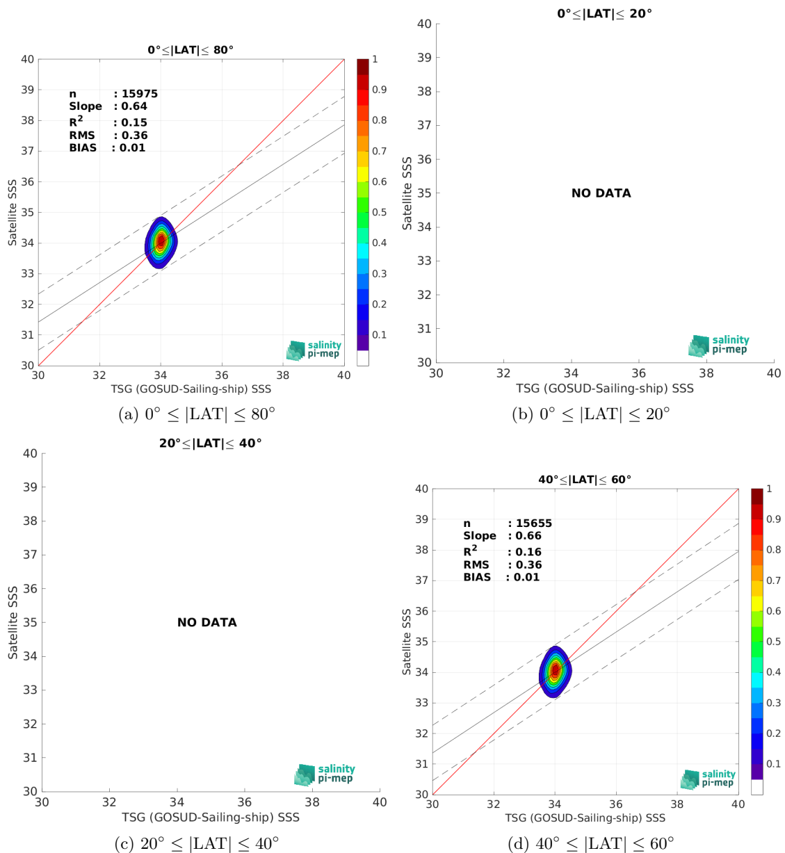
Figure 10: Contour maps of the concentration of SMAP SSS L3 v5.3 - 8-Day running (RSS) SSS (y-axis) versus TSG (GOSUD-Sailing-ship) SSS (x-axis) at match-up pairs for different latitude bands. For each plot, the red line shows x=y . The black thin and dashed lines indicate a linear fit through the data cloud and the \pm 95\% confidence levels, respectively. The number match-up pairs n , the slope and R^2 coefficient of the linear fit, the root mean square (RMS) and the mean bias between satellite and in situ data are indicated for each latitude band in each plots.
