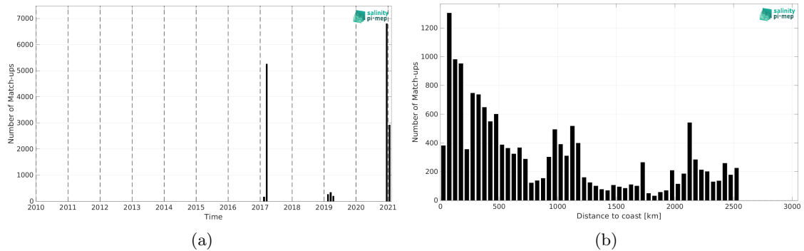
Figure 2: Number of match-ups between TSG (GOSUD-Sailing-ship) and SMAP SSS L3 v5.3 - 8-Day running (RSS) SSS as a function of time (a) and as function of the distance to coast (b) over the Southern Ocean Pi-MEP region and for the full satellite product period.
