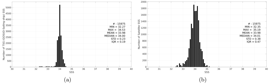
Figure 3: Histograms of SSS from TSG (GOSUD-Sailing-ship) (a) and SMAP SSS L3 v5.3 - 8-Day running (RSS) (b) considering all match-up pairs per bins of 0.1 over the Southern Ocean Pi-MEP region and for the full satellite product period.
