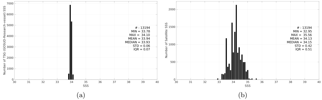
Figure 3: Histograms of SSS from TSG (GOSUD-Research-vessel) (a) and SMAP SSS L3 v5.3 - 8-Day running (RSS) (b) considering all match-up pairs per bins of 0.1 over the Southern Ocean Pi-MEP region and for the full satellite product period.
