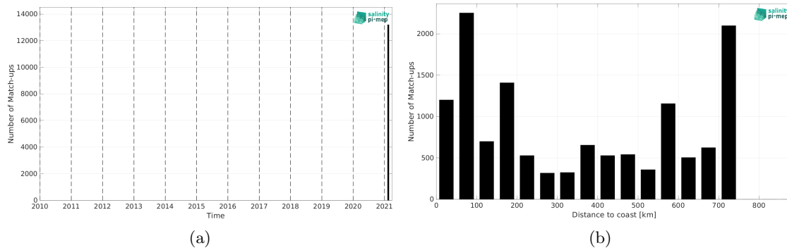
Figure 2: Number of match-ups between TSG (GOSUD-Research-vessel) and SMAP SSS L3 v5.3 - 8-Day running (RSS) SSS as a function of time (a) and as function of the distance to coast (b) over the Southern Ocean Pi-MEP region and for the full satellite product period.
