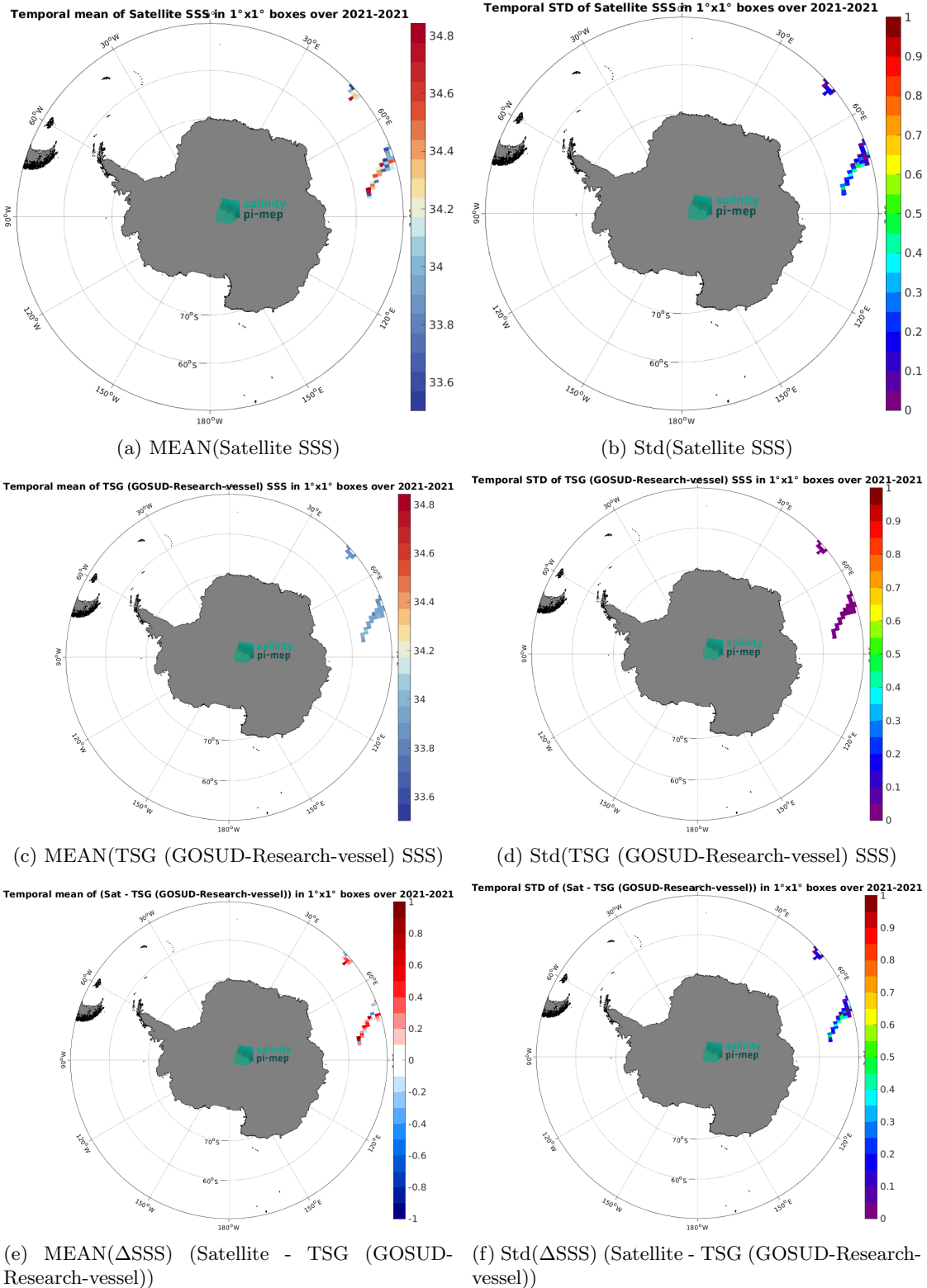
Figure 7: Temporal mean (left) and Std (right) of SSS from SMAP SSS L3 v5.3 - 8-Day running (RSS) (top), TSG (GOSUD-Research-vessel) (middle), and of \Delta SSS (Satellite - TSG (GOSUD-Research-vessel)). Only match-up pairs are used to generate these maps.
