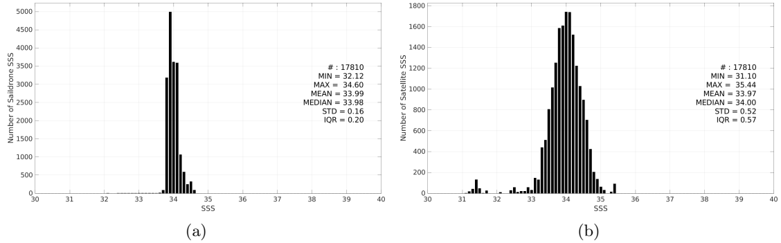
Figure 3: Histograms of SSS from Sairdrone (a) and SMAP SSS L3 v5.3 - 8-Day running (RSS) (b) considering all match-up pairs per bins of 0.1 over the Southern Ocean Pi-MEP region and for the full satellite product period.
