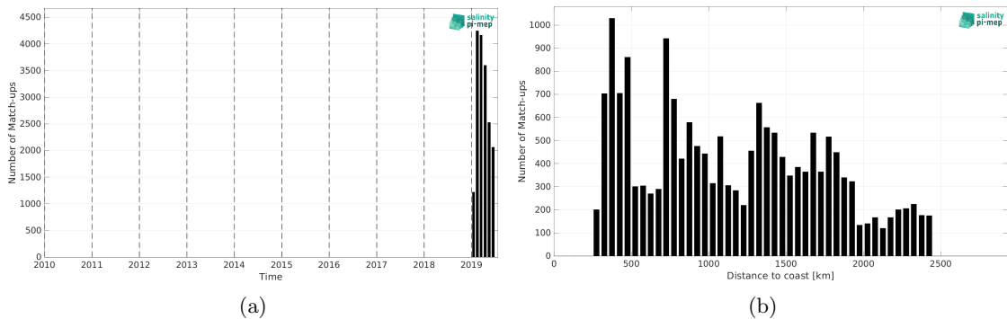
Figure 2: Number of match-ups between Saildrone and SMAP SSS L3 v5.3 - 8-Day running (RSS) SSS as a function of time (a) and as function of the distance to coast (b) over the Southern Ocean Pi-MEP region and for the full satellite product period.
