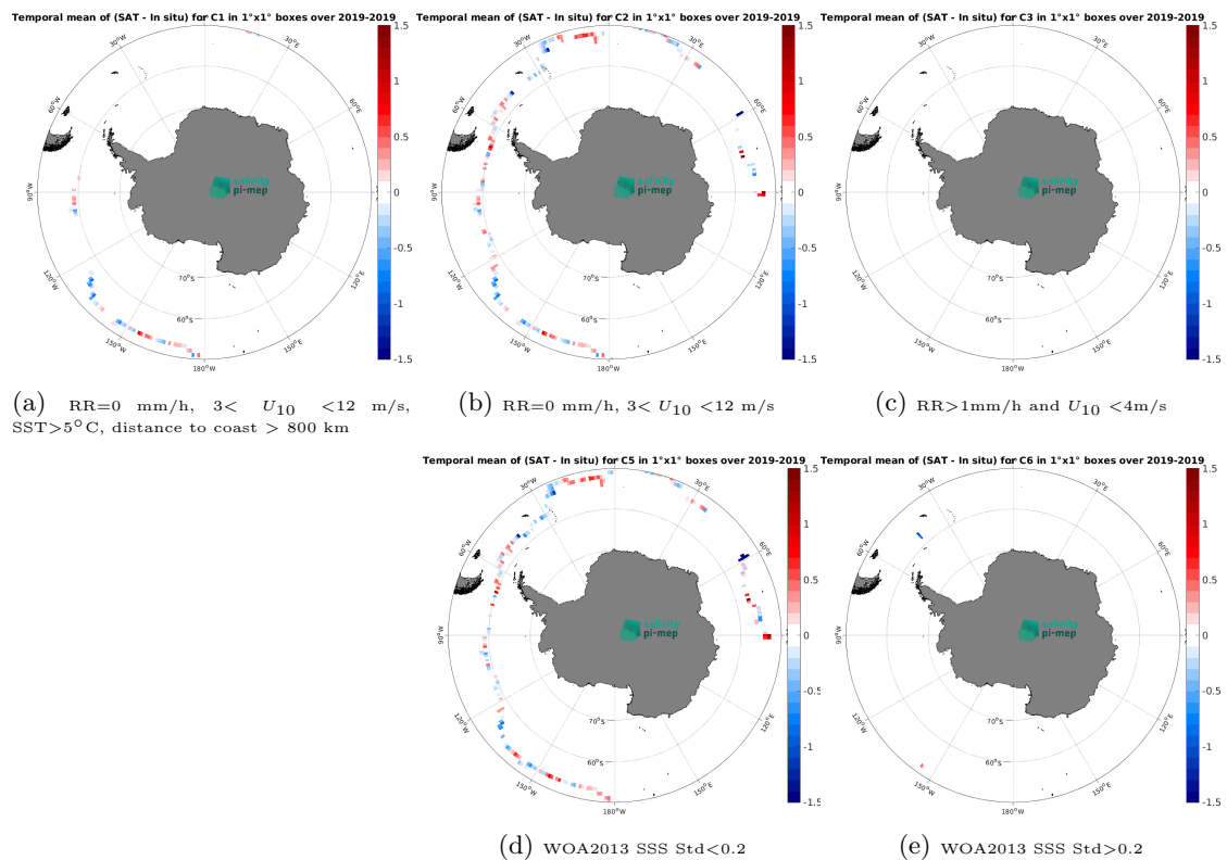
Figure 14: Temporal mean gridded over spatial boxes of size 1^\circ \times 1^\circ of \Delta SSS (SMAP SSS L3 v5.3 - 8-Day running (RSS) - Saildrone) for 5 different subdatasets corresponding to:RR=0 mm/h, 3 < U_{10} < 12 m/s, SST > 5^\circ\text{C} , distance to coast > 800 km (a), RR=0 mm/h, 3 < U_{10} < 12 m/s (b), RR > 1 mm/h and U_{10} < 4 m/s (c), WOA2013 SSS Std < 0.2 (d), WOA2013 SSS Std > 0.2 (e).
