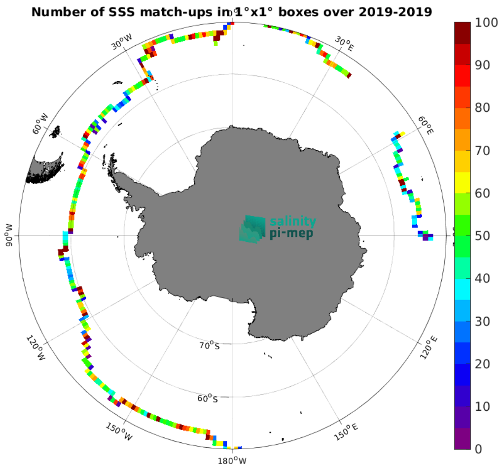
Figure 5: Number of SSS match-ups between Sairdrone SSS and the SMAP SSS L3 v5.3 - 8-Day running (RSS) SSS product for the Southern Ocean Pi-MEP region over 1^\circ \times 1^\circ boxes and for the full satellite product period.
