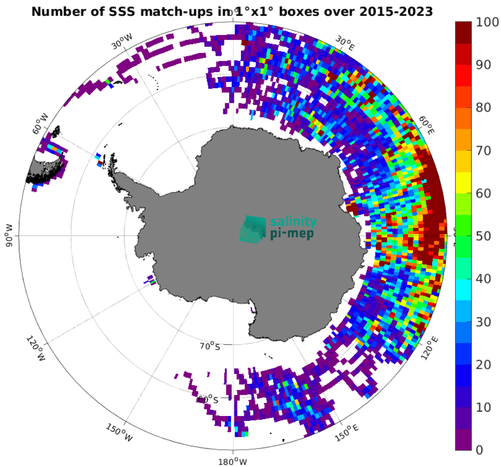
Figure 5: Number of SSS match-ups between Marine mammals SSS and the SMAP SSS L3 v5.3 - 8-Day running (RSS) SSS product for the Southern Ocean Pi-MEP region over 1^\circ \times 1^\circ boxes and for the full satellite product period.
