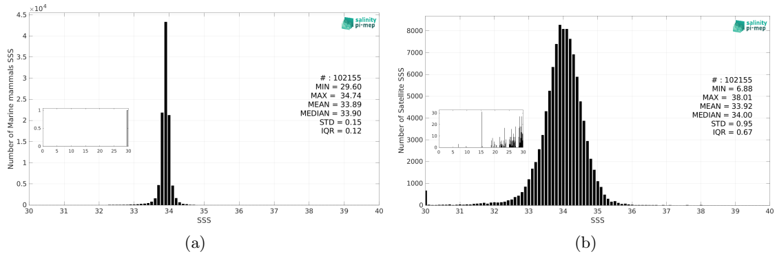
Figure 3: Histograms of SSS from Marine mammals (a) and SMAP SSS L3 v5.3 - 8-Day running (RSS) (b) considering all match-up pairs per bins of 0.1 over the Southern Ocean Pi-MEP region and for the full satellite product period.
