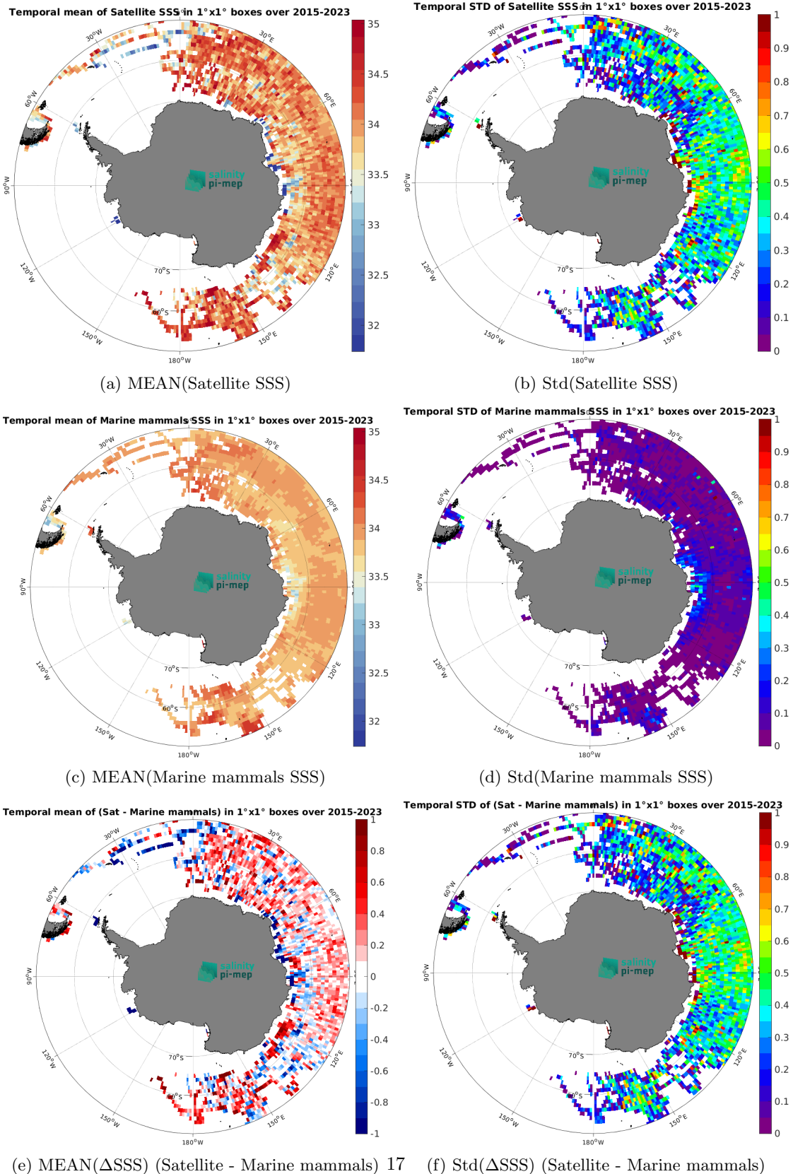
Figure 7: Temporal mean (left) and Std (right) of SSS from SMAP SSS L3 v5.3 - 8-Day running (RSS) (top), Marine mammals (middle), and of \Delta SSS (Satellite - Marine mammals). Only match-up pairs are used to generate these maps.
