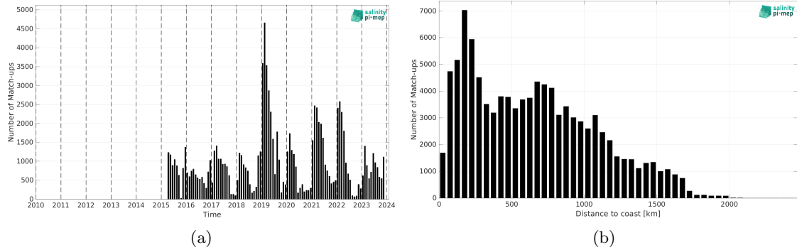
Figure 2: Number of match-ups between Marine mammals and SMAP SSS L3 v5.3 - 8-Day running (RSS) SSS as a function of time (a) and as function of the distance to coast (b) over the Southern Ocean Pi-MEP region and for the full satellite product period.
