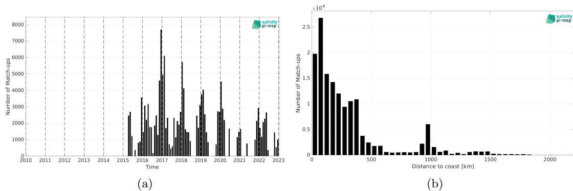
Figure 2: Number of match-ups between TSG (SAMOS) and SMAP SSS L3 v5.3 - Monthly (RSS) SSS as a function of time (a) and as function of the distance to coast (b) over the Southern Ocean Pi-MEP region and for the full satellite product period.
