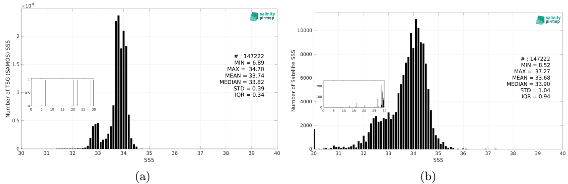
Figure 3: Histograms of SSS from TSG (SAMOS) (a) and SMAP SSS L3 v5.3 - Monthly (RSS) (b) considering all match-up pairs per bins of 0.1 over the Southern Ocean Pi-MEP region and for the full satellite product period.
