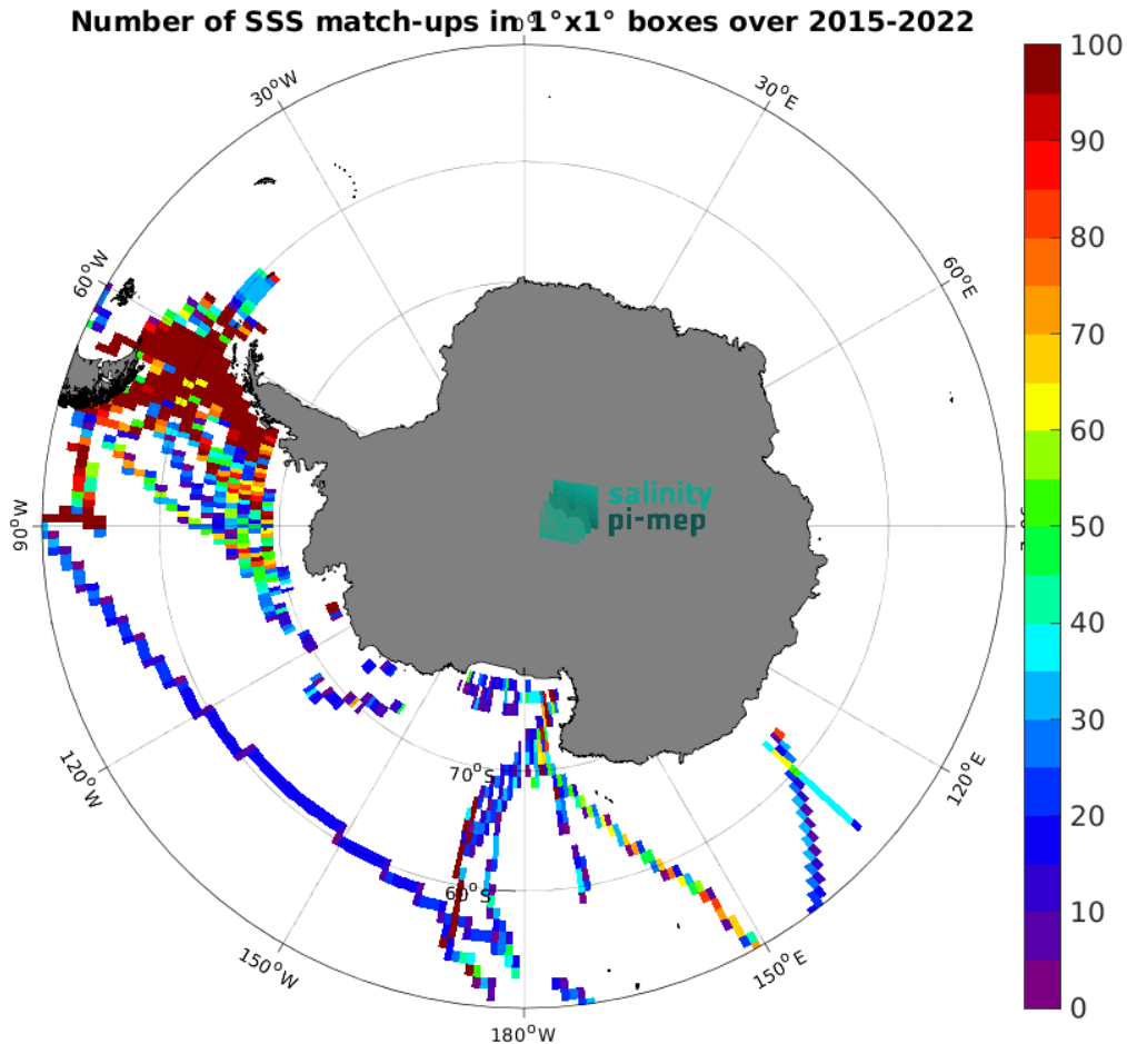
Figure 5: Number of SSS match-ups between TSG (SAMOS) SSS and the SMAP SSS L3 v5.3 - Monthly (RSS) SSS product for the Southern Ocean Pi-MEP region over 1^\circ \times 1^\circ boxes and for the full satellite product period.
