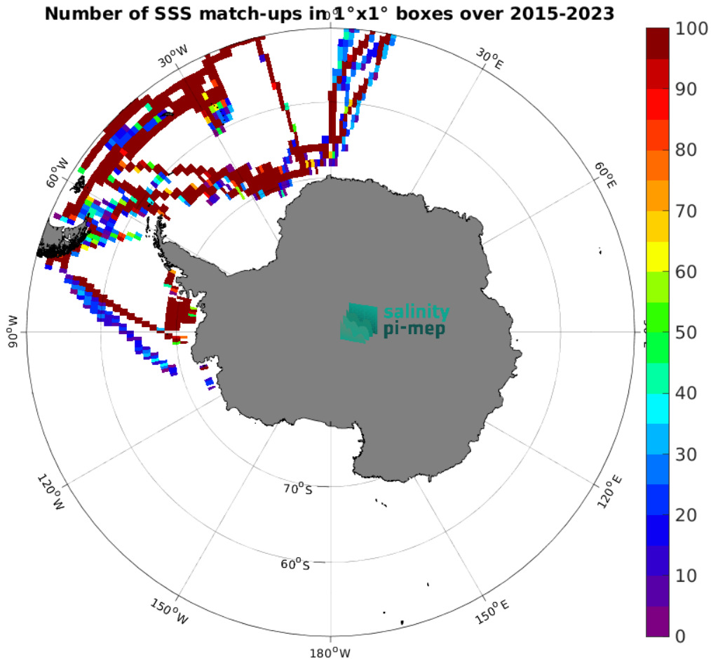
Figure 5: Number of SSS match-ups between TSG (Polarstern) SSS and the SMAP SSS L3 v5.3 - Monthly (RSS) SSS product for the Southern Ocean Pi-MEP region over 1^\circ \times 1^\circ boxes and for the full satellite product period.
