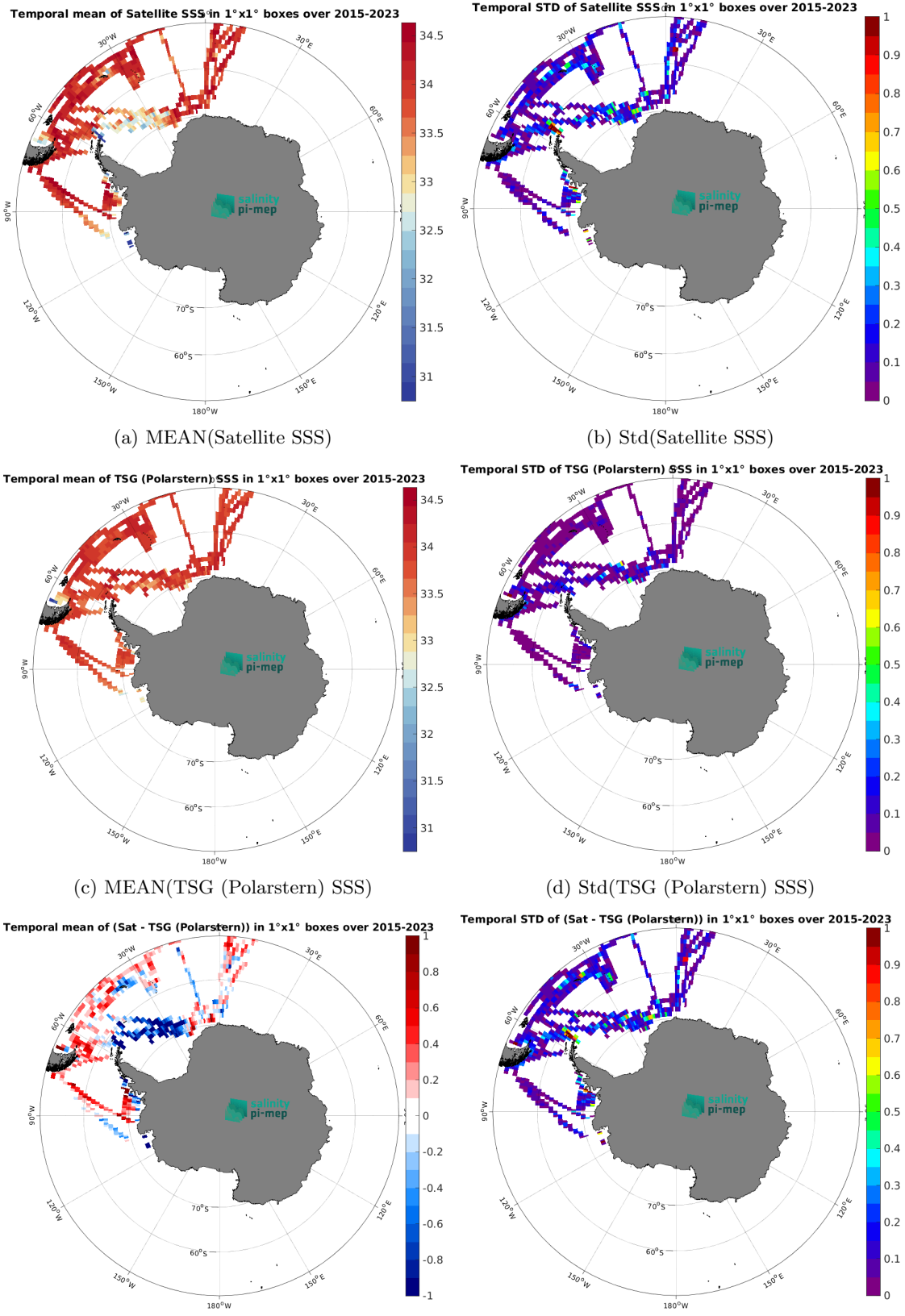
Figure 7: Temporal mean (left) and Std (right) of SSS from SMAP SSS L3 v5.3 - Monthly (RSS) (top), TSG (Polarstern) (middle), and of \Delta SSS (Satellite - TSG (Polarstern)). Only match-up pairs are used to generate these maps.
