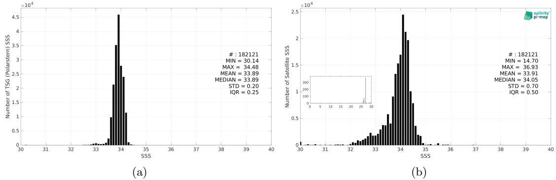
Figure 3: Histograms of SSS from TSG (Polarstern) (a) and SMAP SSS L3 v5.3 - Monthly (RSS) (b) considering all match-up pairs per bins of 0.1 over the Southern Ocean Pi-MEP region and for the full satellite product period.
