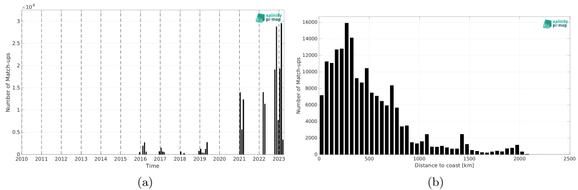
Figure 2: Number of match-ups between TSG (Polarstern) and SMAP SSS L3 v5.3 - Monthly (RSS) SSS as a function of time (a) and as function of the distance to coast (b) over the Southern Ocean Pi-MEP region and for the full satellite product period.
