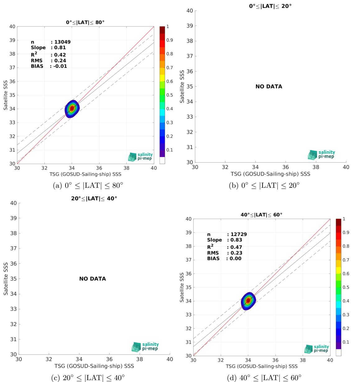
Figure 10: Contour maps of the concentration of SMAP SSS L3 v5.3 - Monthly (RSS) SSS (y-axis) versus TSG (GOSUD-Sailing-ship) SSS (x-axis) at match-up pairs for different latitude bands. For each plot, the red line shows x=y . The black thin and dashed lines indicate a linear fit through the data cloud and the \pm 95\% confidence levels, respectively. The number match-up pairs n , the slope and R^2 coefficient of the linear fit, the root mean square (RMS) and the mean bias between satellite and in situ data are indicated for each latitude band in each plots.
