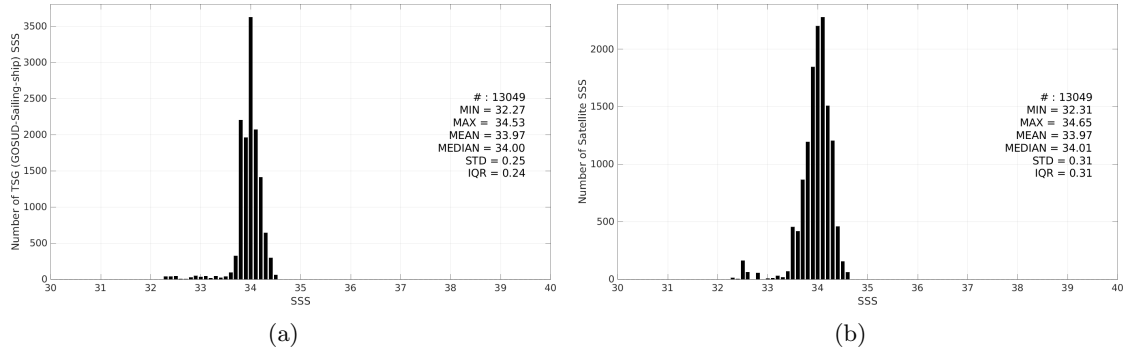
Figure 3: Histograms of SSS from TSG (GOSUD-Sailing-ship) (a) and SMAP SSS L3 v5.3 - Monthly (RSS) (b) considering all match-up pairs per bins of 0.1 over the Southern Ocean Pi-MEP region and for the full satellite product period.
