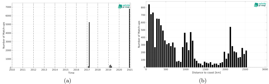
Figure 2: Number of match-ups between TSG (GOSUD-Sailing-ship) and SMAP SSS L3 v5.3 - Monthly (RSS) SSS as a function of time (a) and as function of the distance to coast (b) over the Southern Ocean Pi-MEP region and for the full satellite product period.
