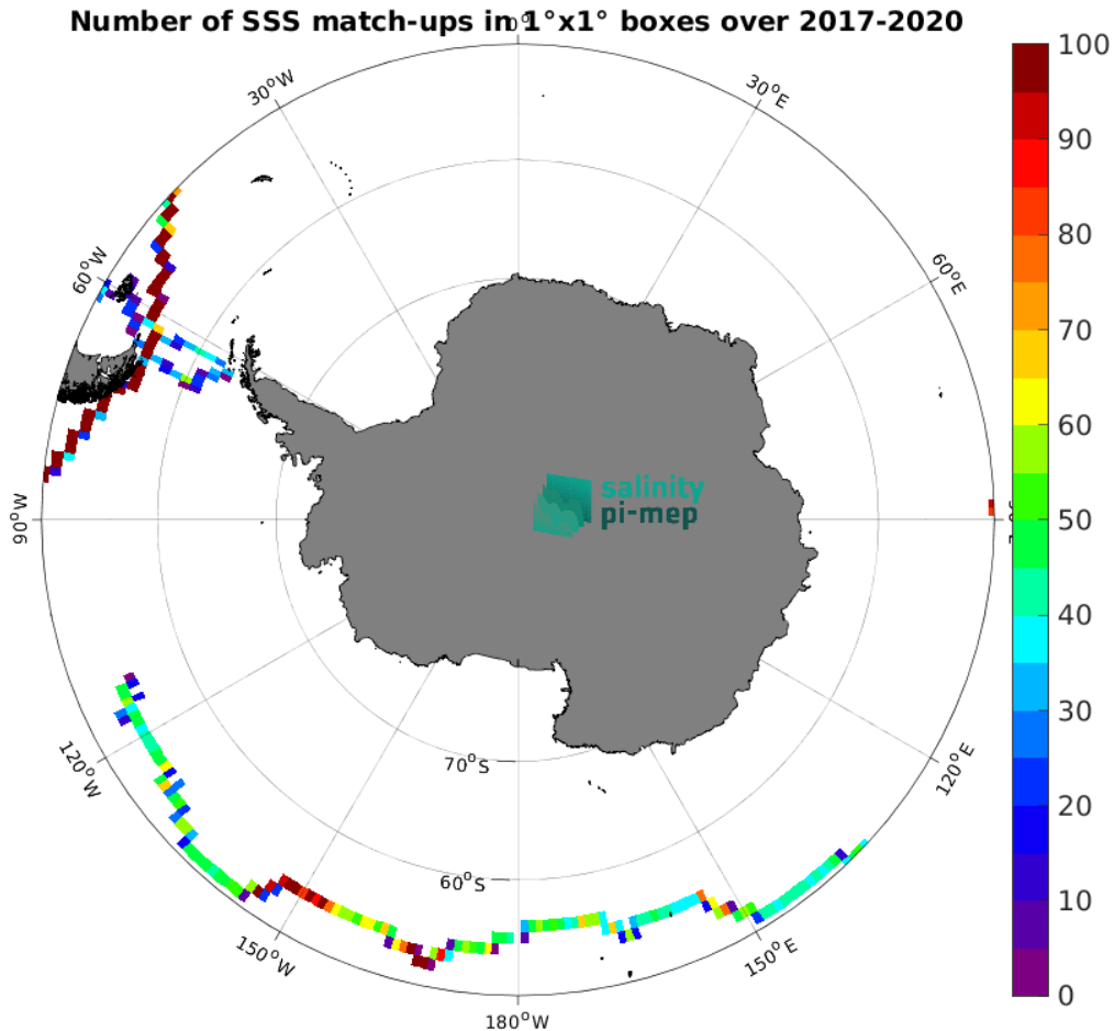
Figure 5: Number of SSS match-ups between TSG (GOSUD-Sailing-ship) SSS and the SMAP SSS L3 v5.3 - Monthly (RSS) SSS product for the Southern Ocean Pi-MEP region over 1^\circ \times 1^\circ boxes and for the full satellite product period.
