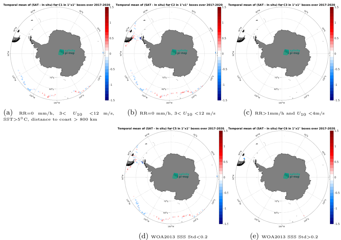
Figure 14: Temporal mean gridded over spatial boxes of size 1^\circ \times 1^\circ of \Delta SSS (SMAP SSS L3 v5.3 - Monthly (RSS) - TSG (GOSUD-Sailing-ship)) for 5 different subdatasets corresponding to:RR=0 mm/h, 3 < U_{10} < 12 m/s, SST >5^\circ C, distance to coast > 800 km (a), RR=0 mm/h, 3 < U_{10} < 12 m/s (b), RR >1 mm/h and U_{10} < 4 m/s (c), WOA2013 SSS Std <0.2 (d), WOA2013 SSS Std >0.2 (e).
