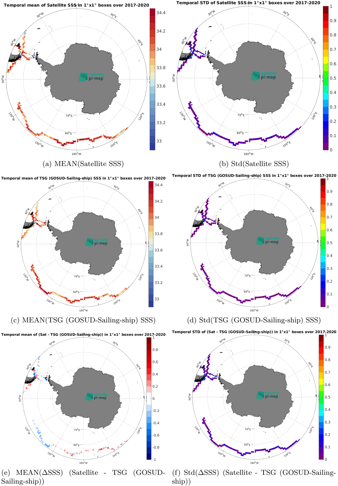
Figure 7: Temporal mean (left) and Std (right) of SSS from SMAP SSS L3 v5.3 - Monthly (RSS) (top), TSG (GOSUD-Sailing-ship) (middle), and of \Delta SSS (Satellite - TSG (GOSUD-Sailing-ship)). Only match-up pairs are used to generate these maps.
